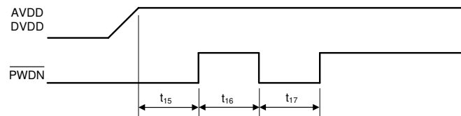
図 7-15. Power-Up Timing Sequence
