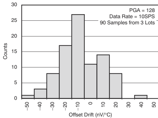
图 5-13. Offset Drift ( -40^\circ\text{C} to +25^\circ\text{C} )
