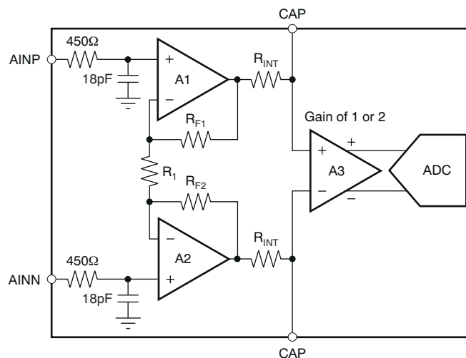
図 7-2. Simplified Diagram of the PGA
