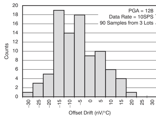
图 5-14. Offset Drift ( 25^\circ\text{C} to 105^\circ\text{C} )
