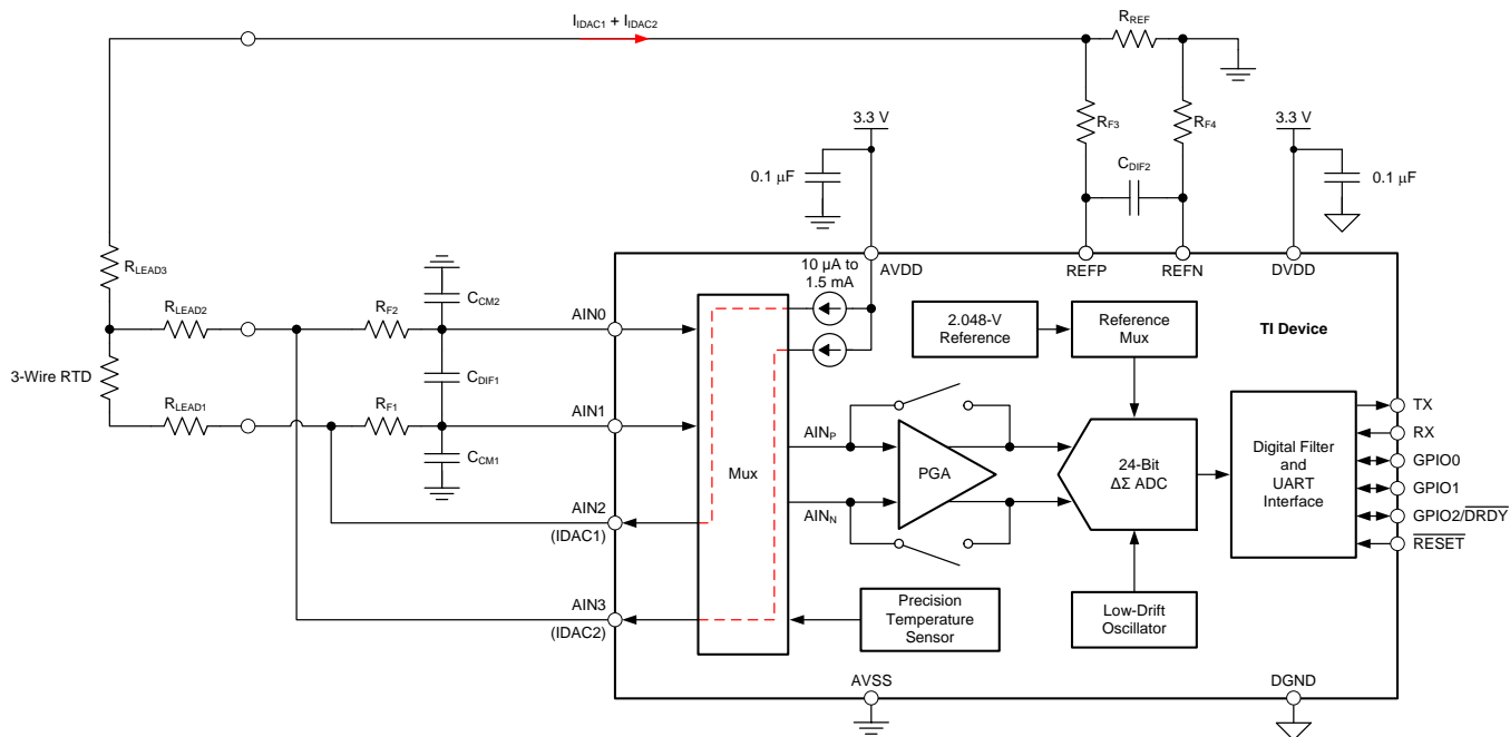
☒ 79. 3-Wire RTD Measurement
