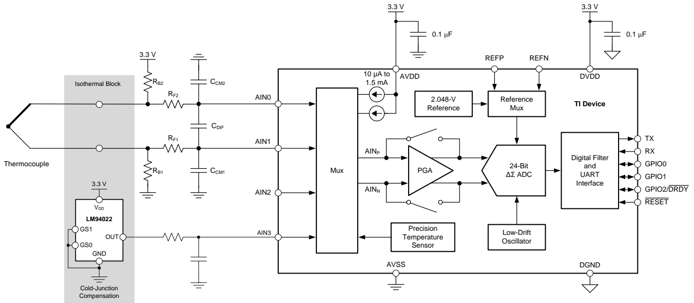
Figure 76. Thermocouple Measurement
