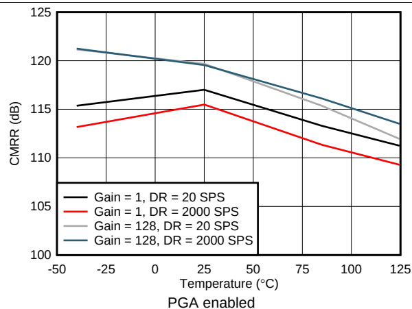
23. DC CMRR vs Temperature
