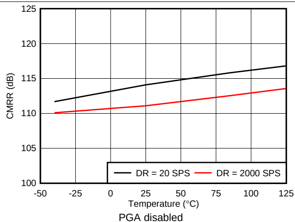
22. DC CMRR vs Temperature
