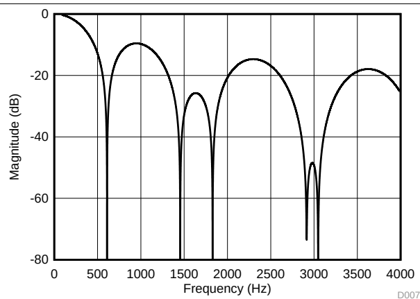
FIG 51. Filter Response (Normal Mode, DR = 600 SPS)
