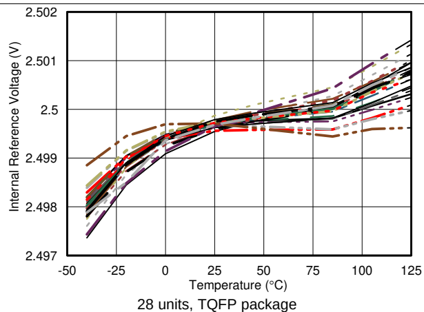
FIG 20. Internal Reference Voltage vs Temperature
