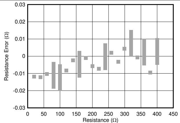
Figure 98. Measured Resistance Error vs Equivalent RTD Resistance
