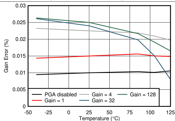
FIG 19. Gain Error vs Temperature
