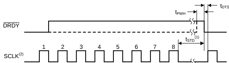
✎ 1. Serial Interface Timing, DRDY MODE Bit = 0
