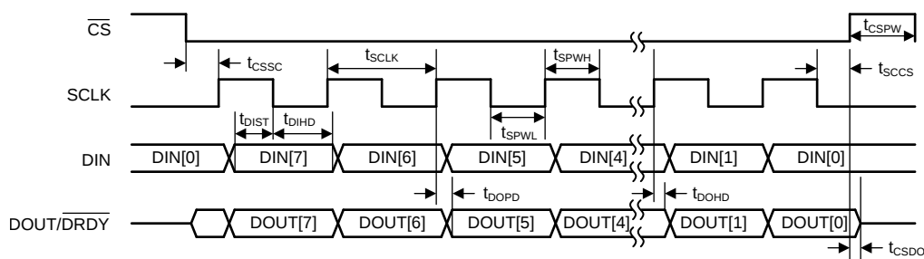
✎ 1. Serial Interface Timing, DRDY MODE Bit = 0
