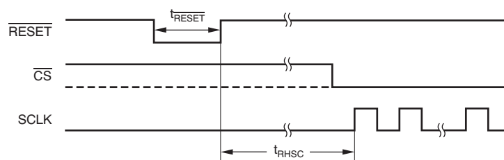
✎ 4. Reset Pulse Duration and Serial Interface Communication After Reset
