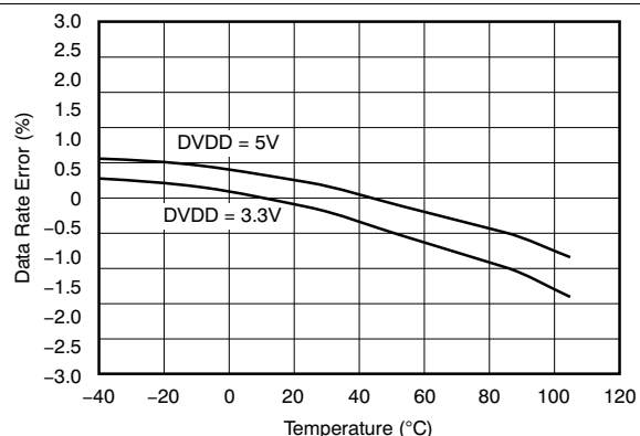
FIG 6. Data Rate Error vs Temperature
