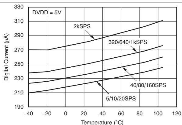
FIG 14. Digital Supply Current vs Temperature
