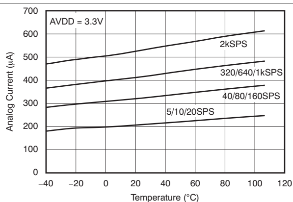
FIG 15. Analog Supply Current vs Temperature
