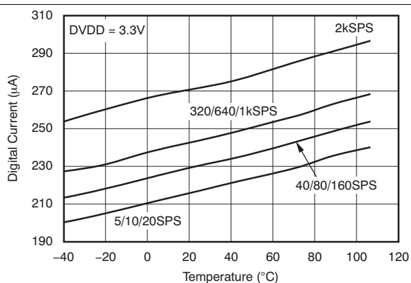
FIG 16. Digital Supply Current vs Temperature
