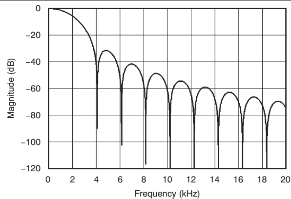
图 35. Filter Profile With Data Rate = 2 kSPS
