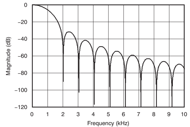
图 34. Filter Profile With Data Rate = 1 kSPS
