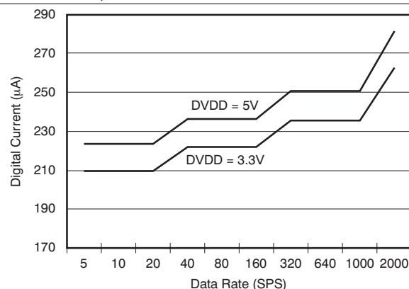
FIG 12. Digital Supply Current vs Data Rate
