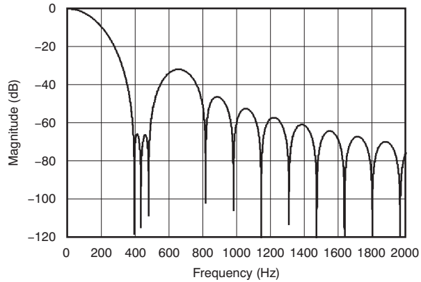
图 31. Filter Profile With Data Rate = 160 SPS
