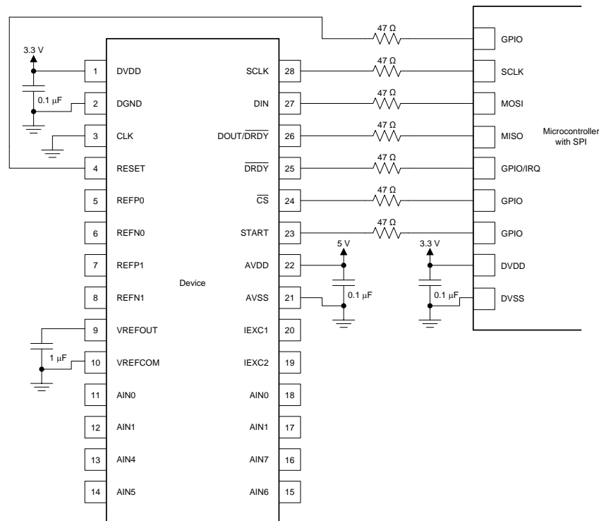
Figure 77. Serial Interface Connections
