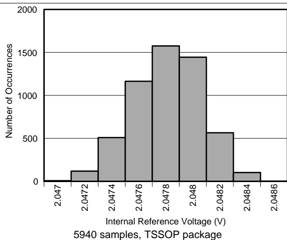
FIG 26. Internal Reference Voltage Histogram
