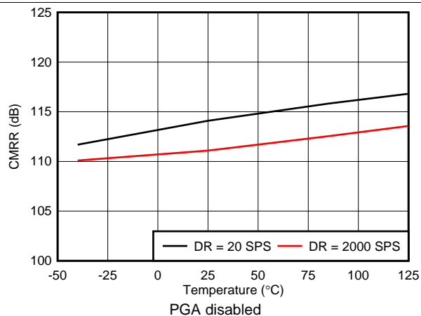
FIG 24. DC CMRR vs Temperature
