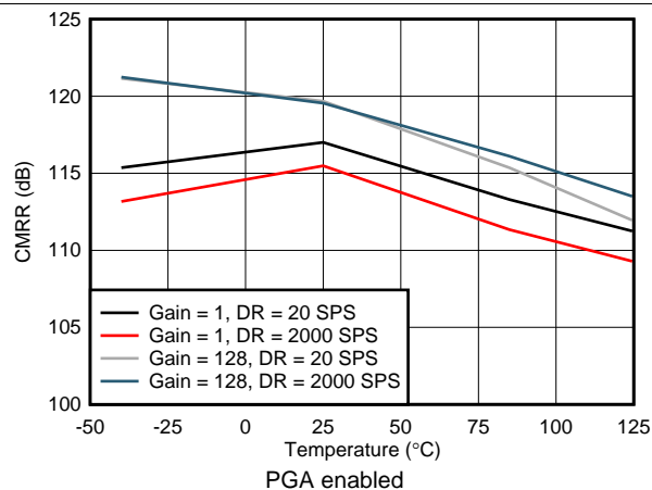
FIG 25. DC CMRR vs Temperature
