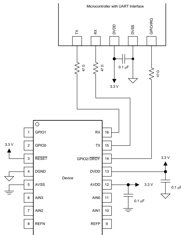
Figure 74. Interface Connections
