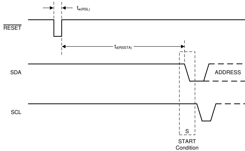
2. RESET Pin Timing Requirements
