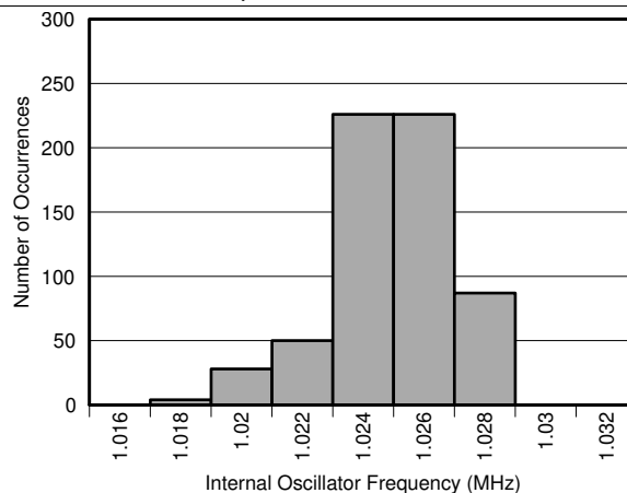
FIG 17. Internal Oscillator Frequency Histogram
