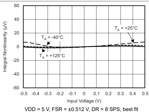
FIG 6-12. INL vs Input Signal
