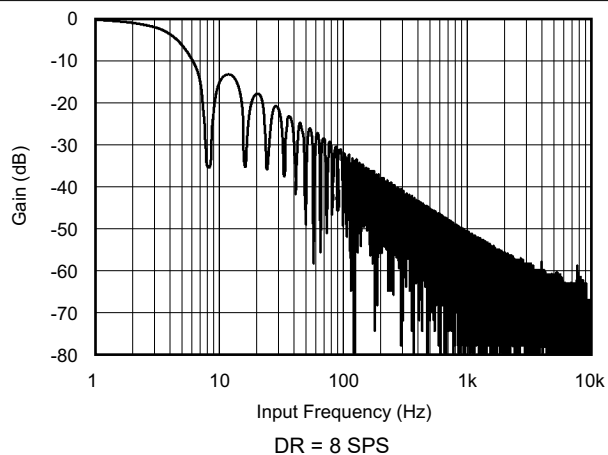
6-21. Digital Filter Frequency Response
