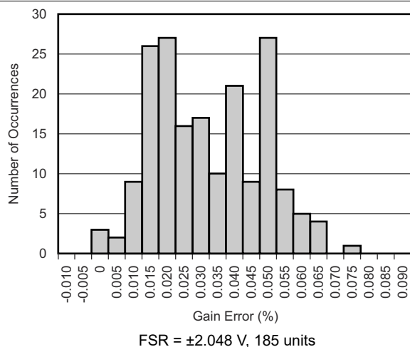
6-17. Gain Error Histogram
