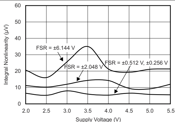
FIG 6-8. INL vs Supply Voltage
