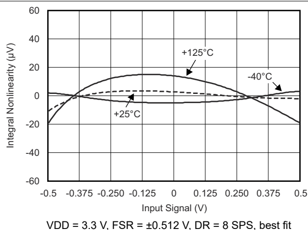
FIG 6-10. INL vs Input Signal
