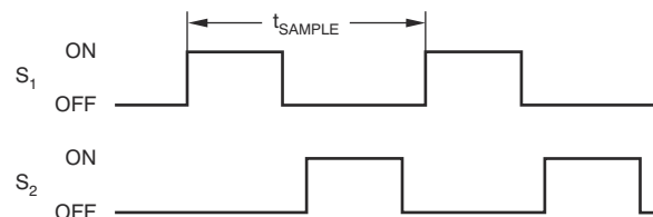
Figure 8-6. S_1 and S_2 Switch Timing
