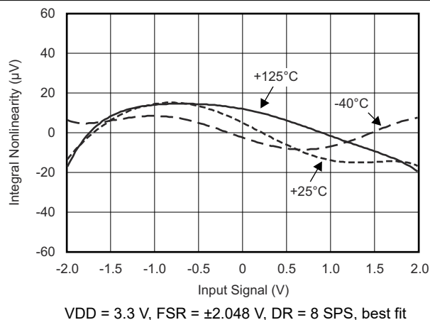
FIG 6-9. INL vs Input Signal
