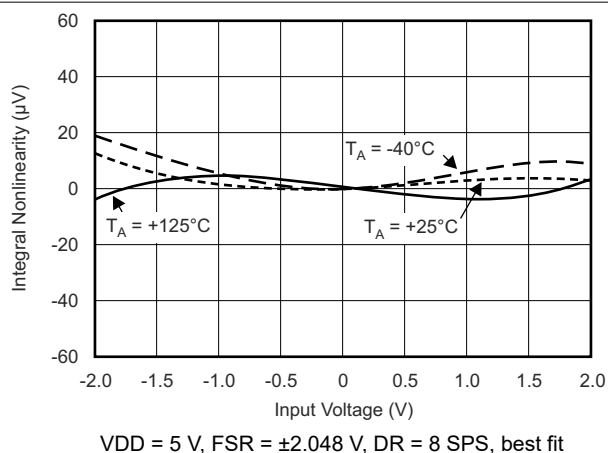
FIG 6-11. INL vs Input Signal
