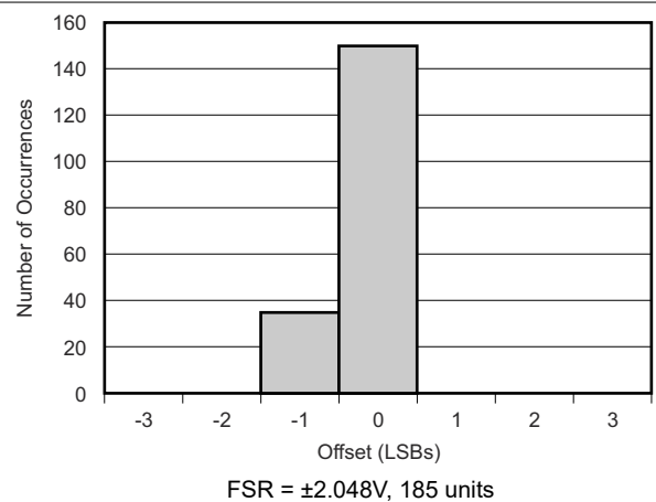
5-18. Offset Histogram
