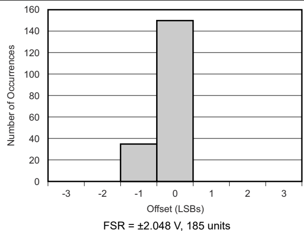
FIG 6-18. Offset Histogram
