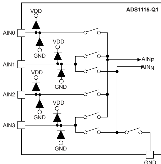
8-4. Input Multiplexer
