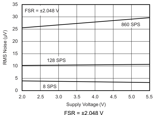
FIG 6-15. Noise vs Supply Voltage
