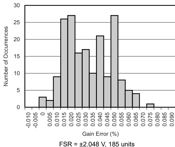
FIG 6-17. Gain Error Histogram
