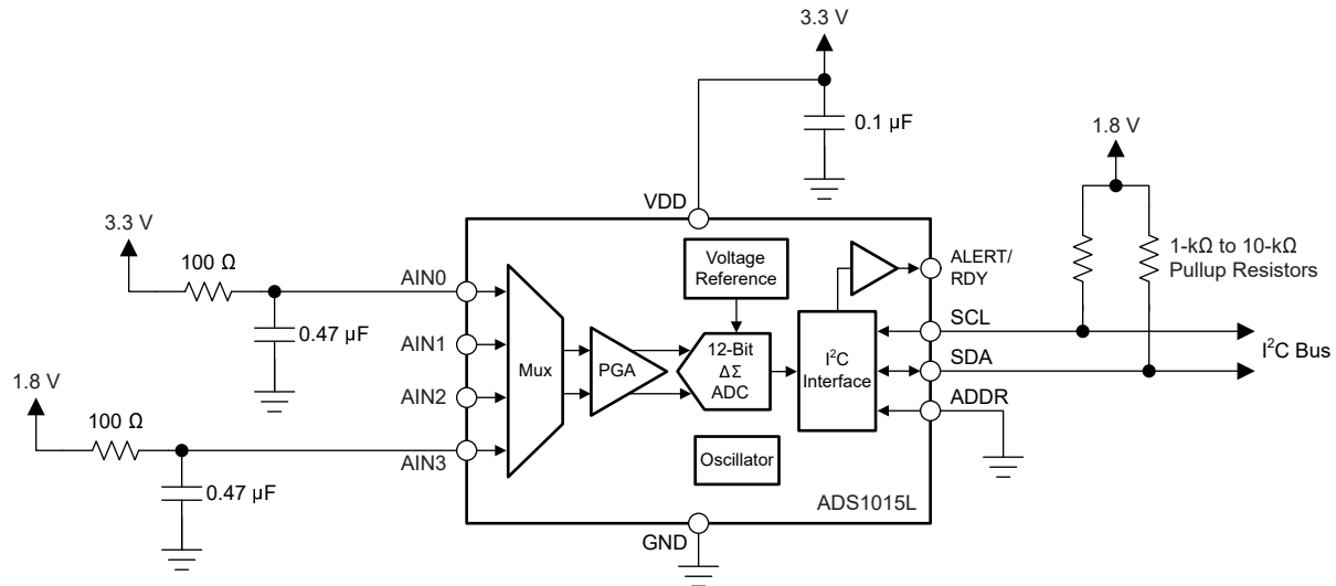
図 9-9. Monitoring Two Supply Voltage Rails Using the ADS1015L
