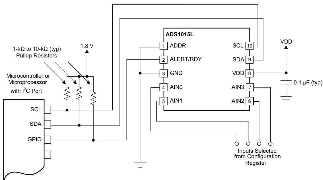
図 9-1. Typical Connections of the ADS1015L
