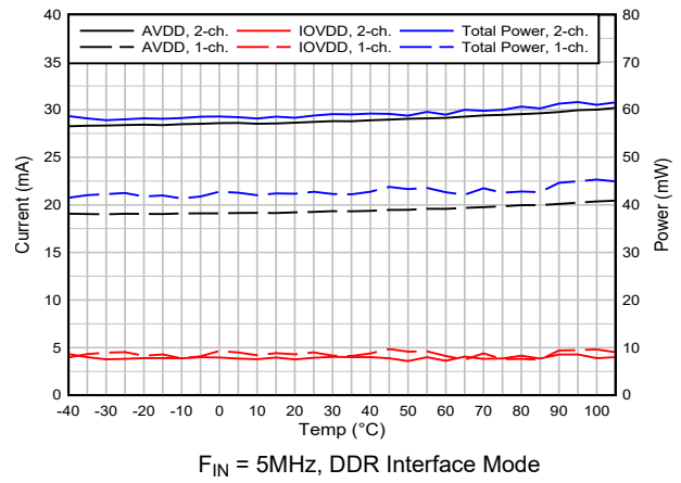
Figure 5-22. Current vs Temperature
