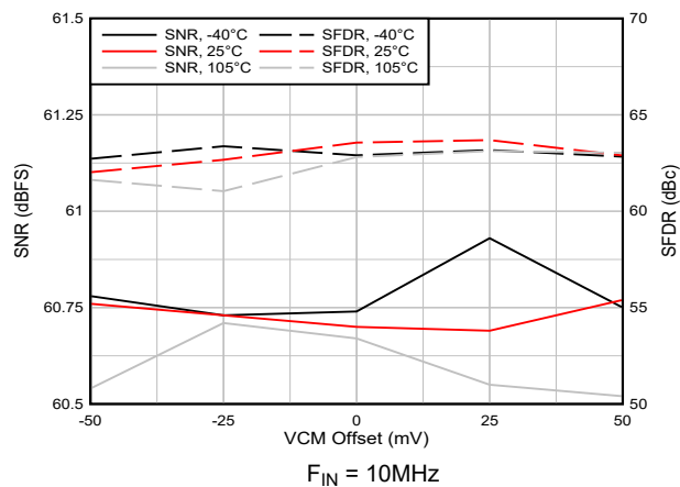
图 5-58. AC Performance vs VCM vs Temperature
