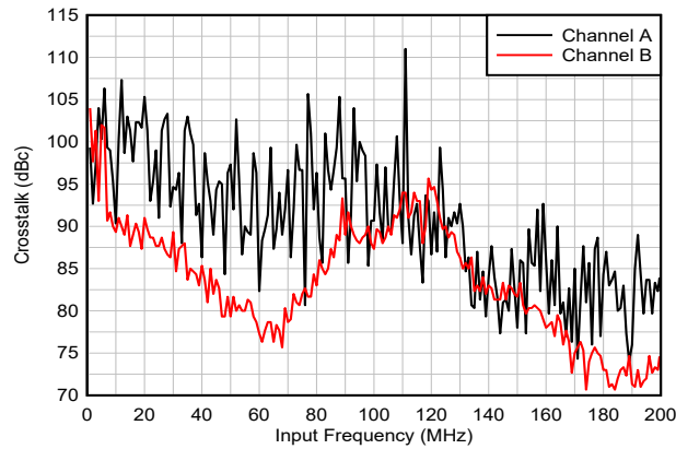
图 5-56. Crosstalk vs Input Frequency
