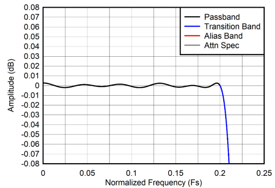
図 6-13. Decimation by 2 passband ripple response
