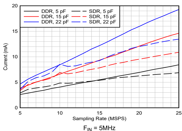
5-23. I_{OVDD} Current vs Load Capacitance
