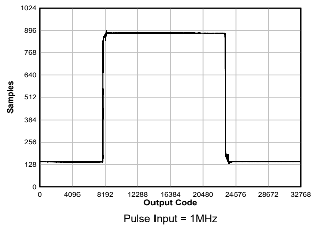
Figure 5-19. Pulse Response
