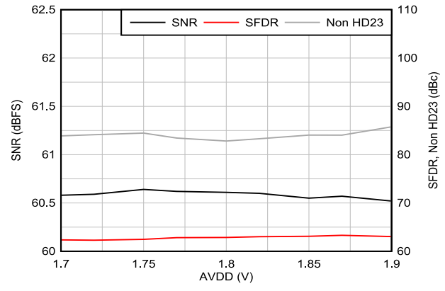
图 5-57. AC Performance vs AVDD
