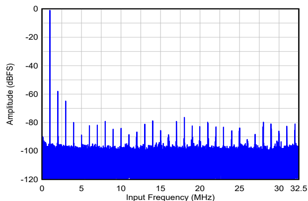
図 5-25. Single Tone FFT at F_{IN} = 1\text{MHz} , Single-ended input
