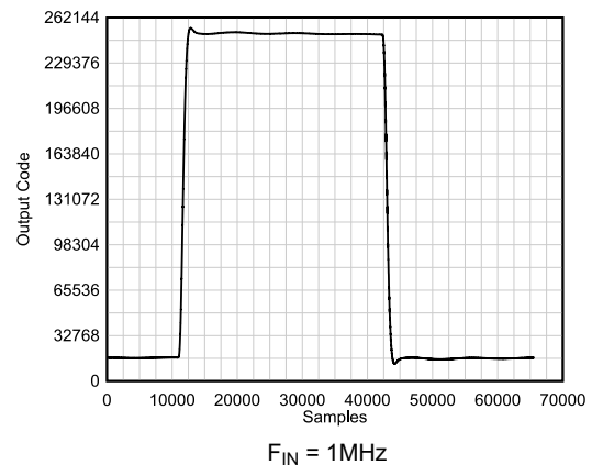
FIG 5-24. Pulse Response
