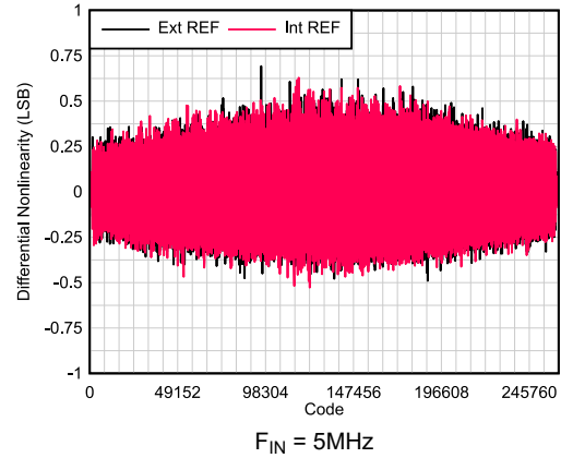
FIG 5-22. DNL vs Code
