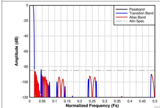
7-35. Decimation by 32 complex frequency response
