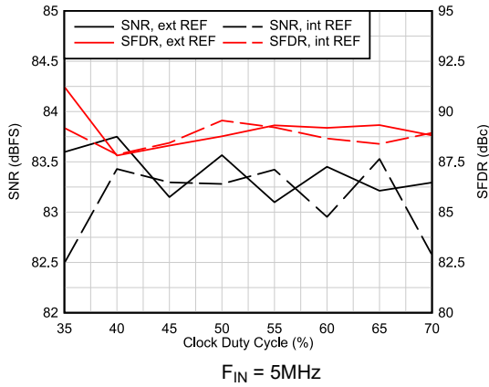
FIG 5-19. AC Performance vs Clock Duty Cycle
