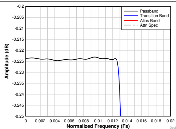
7-36. Decimation by 32 complex passband ripple response
