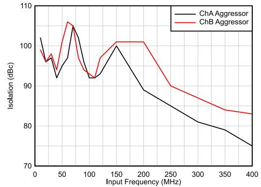
FIG 5-20. Isolation vs Input Frequency
