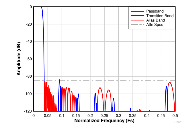
7-33. Decimation by 16 complex frequency response
