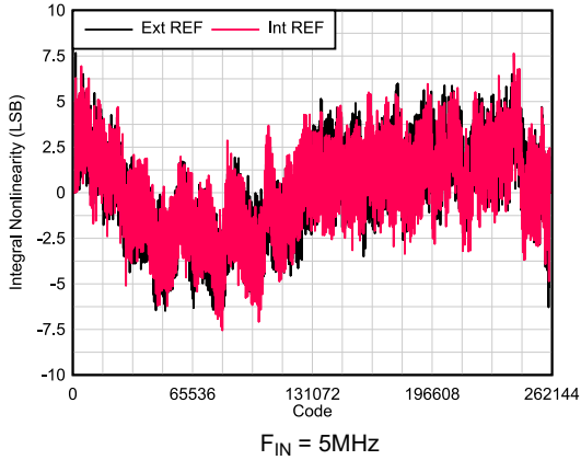
FIG 5-21. INL vs Code
