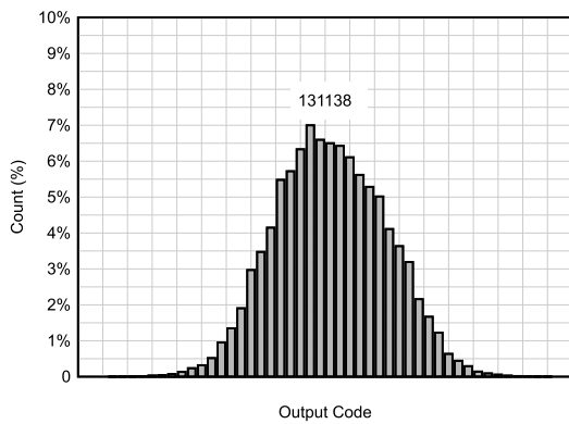
FIG 5-23. DC Offset Histogram
