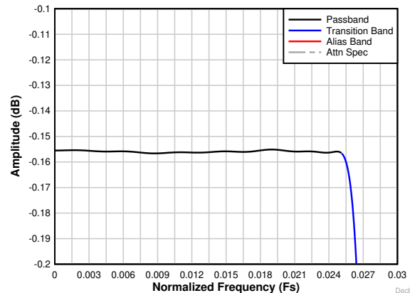
7-34. Decimation by 16 complex passband ripple response
