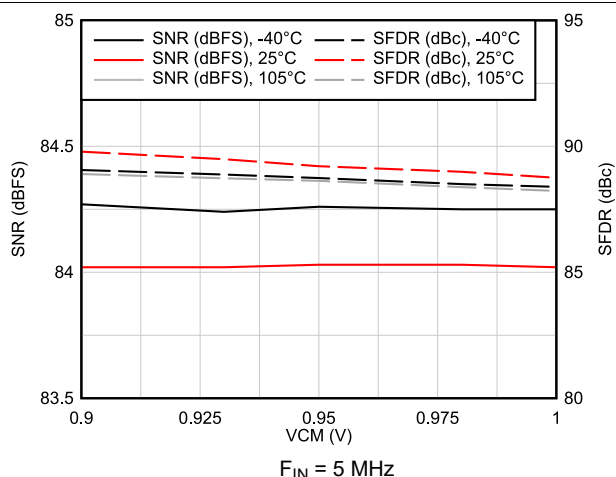
FIG 6-57. AC Performance vs VCM vs Temperature
