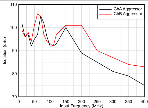
FIG 6-59. Isolation vs Input Frequency
