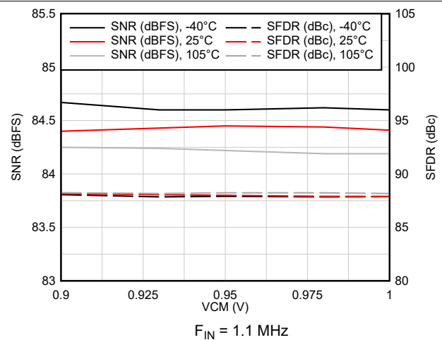
Figure 6-33. AC Performance vs VCM vs Temperature
