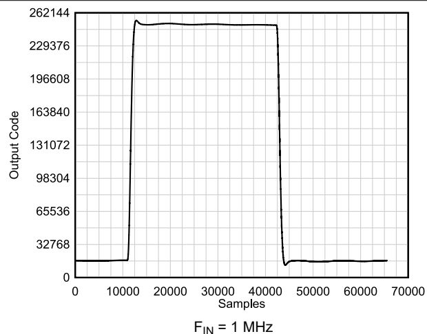
FIG 6-63. Pulse Response
