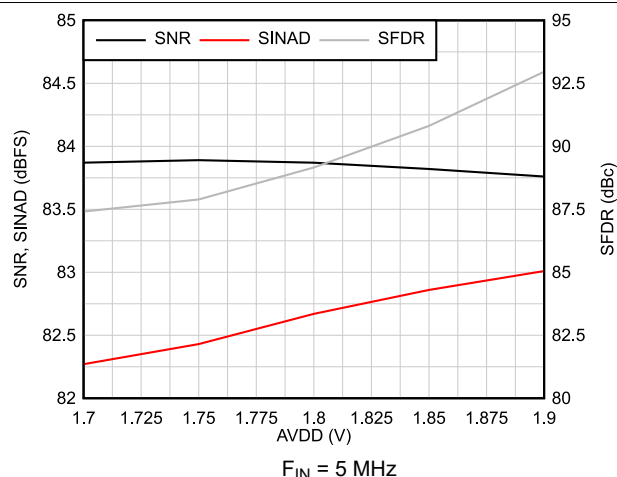
FIG 6-56. AC Performance vs AVDD
