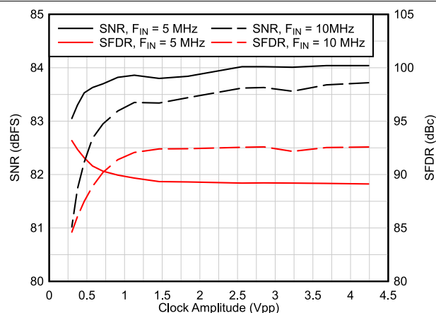
FIG 6-54. AC Performance vs Clock Amplitude
