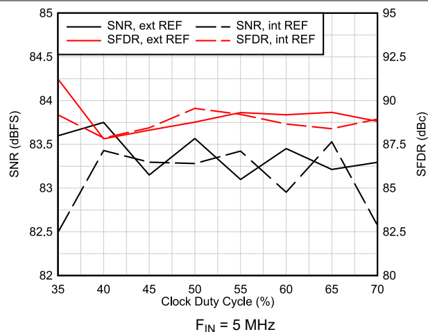
FIG 6-58. AC Performance vs Clock Duty Cycle
