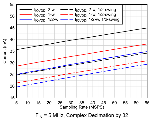
FIG 6-66. I_{IOVDD} Current vs Output Interface
