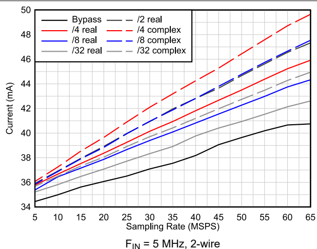
FIG 6-65. I_{IOVDD} Current vs Decimation
