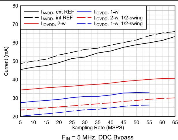
FIG 6-64. Current vs Sampling Rate
