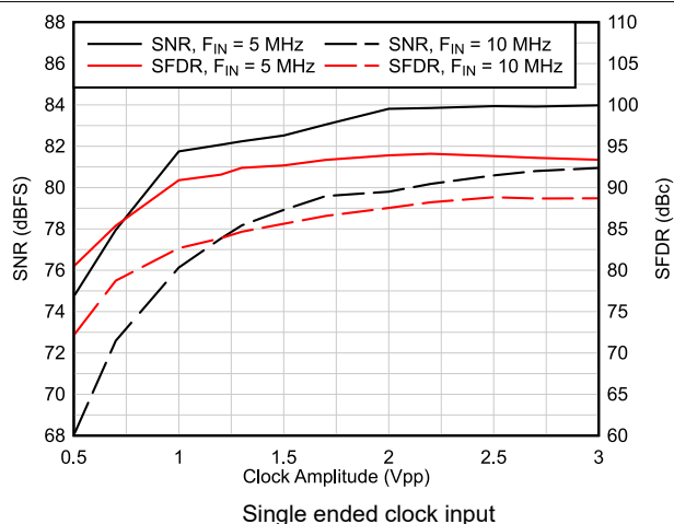
FIG 6-55. AC Performance vs Clock Amplitude
