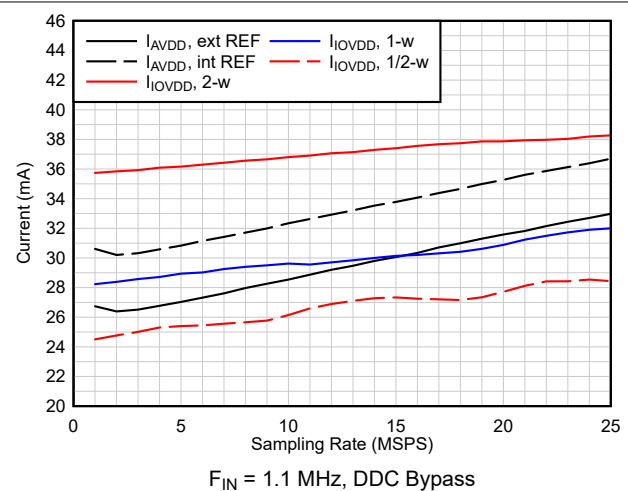
FIG 6-37. Current vs Sampling Rate
