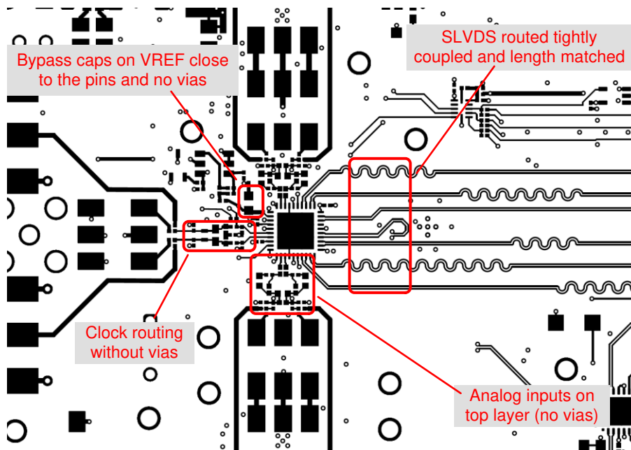
FIG 9-10. Layout example: top layer of ADC368x EVM
