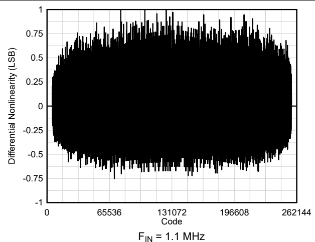
FIG 6-35. DNL vs Code
