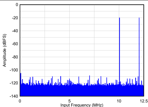
A_{IN} = -20\text{ dBFS/line} , \text{IMD3} = 88\text{ dBc} 6-26. Two Tone FFT at F_{IN} = 10/12\text{ MHz}
