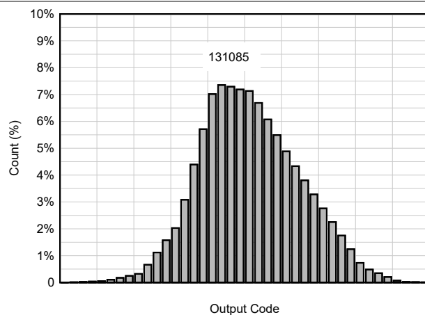
FIG 6-36. DC Offset Histogram
