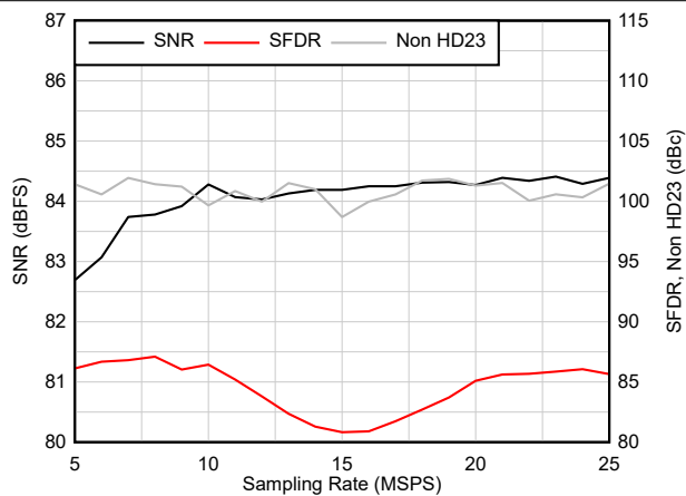
F_{IN} = 1.1\text{ MHz} 6-30. AC Performance vs Sampling Rate
