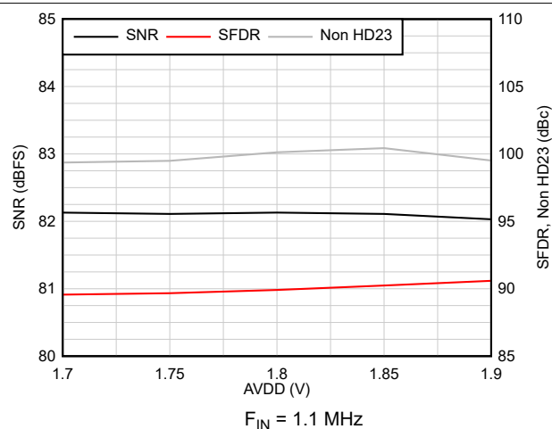
6-32. AC Performance vs AVDD
