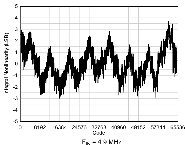
6-34. INL vs Code
