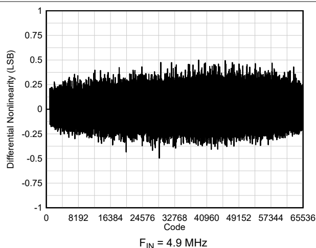
6-35. DNL vs Code
