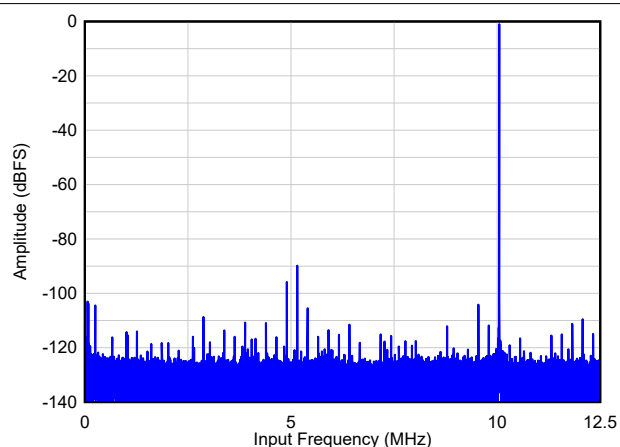
FIG 6-21. Single Tone FFT at F_{IN} = 10 MHz
