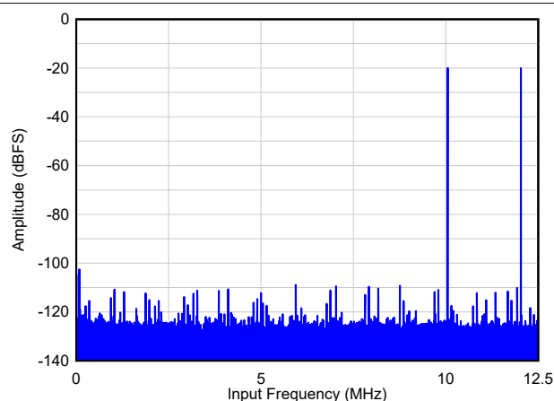
Figure 6-26. Two Tone FFT at F_{IN} = 10/12 MHz A_{IN} = -20 dBFS/tone, IMD3 = 88 dBc
