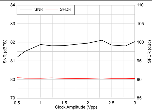
Figure 6-31. AC Performance vs Clock Amplitude F_{IN} = 1.1 MHz
