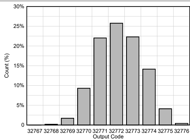
6-36. DC Offset Histogram
