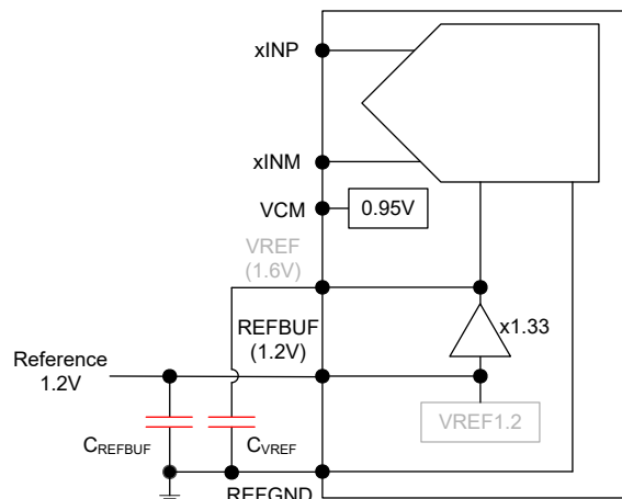
FIG 8-20. External 1.2V reference using internal reference buffer
