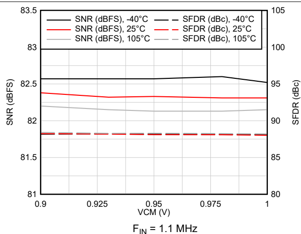
6-33. AC Performance vs VCM vs Temperature
