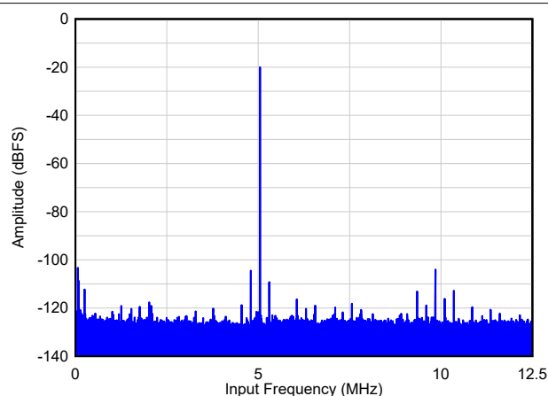
FIG 6-20. Single Tone FFT at F_{IN} = 5 MHz, A_{IN} = -20 dBFS
