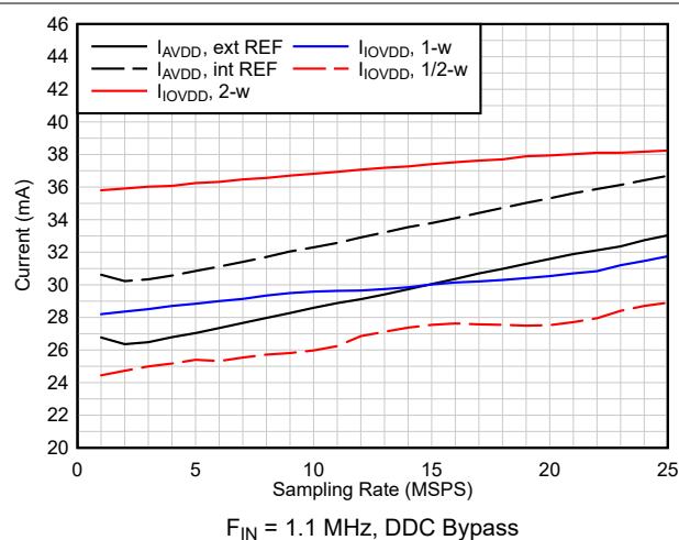
6-37. Current vs Sampling Rate
