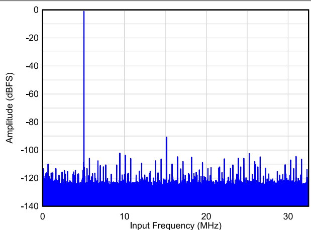
图 6-41. Single Tone FFT at F_{IN} = 5 MHz
