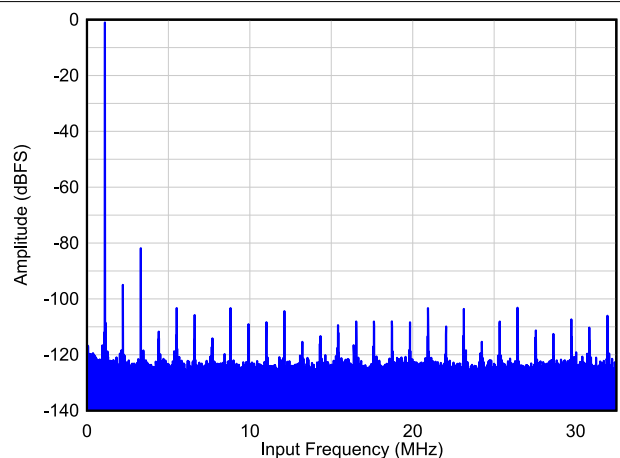
图 6-40. Single Tone FFT at F_{IN} = 1 MHz
