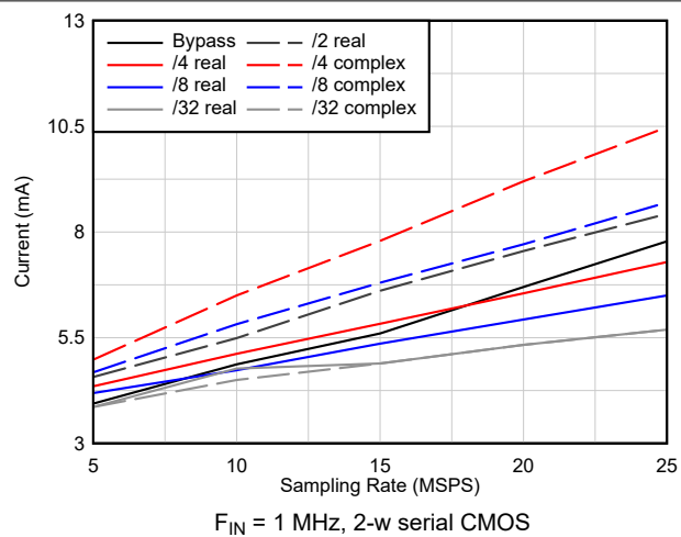
6-37. I_{IOVDD} Current vs Decimation
