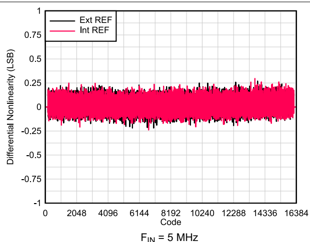
FIG 6-56. DNL vs Code
