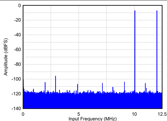
6-24. Two Tone FFT at F_{IN} = 10, 12 MHz
