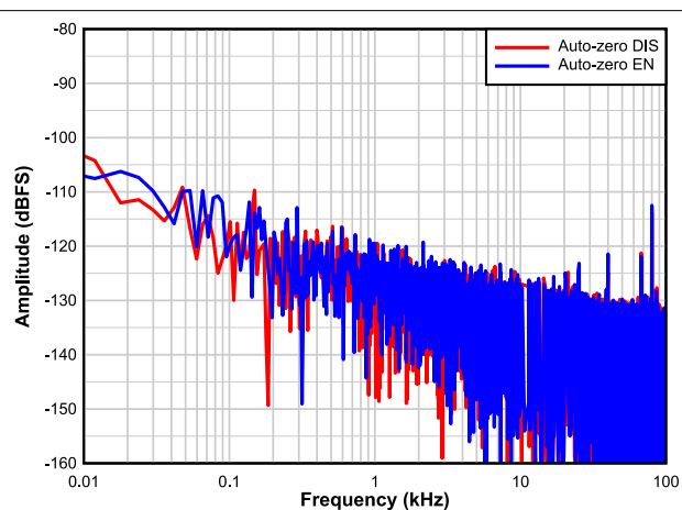
8-12. F_S = 25 MSPS, F_{IN} = 1.1 MHz
