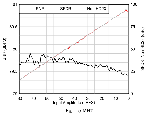
6-50. AC Performance vs Input Amplitude
