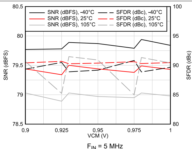
6-54. AC Performance vs VCM vs Temperature
