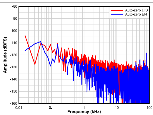
8-14. F_S = 65 MSPS, F_{IN} = 5 MHz
