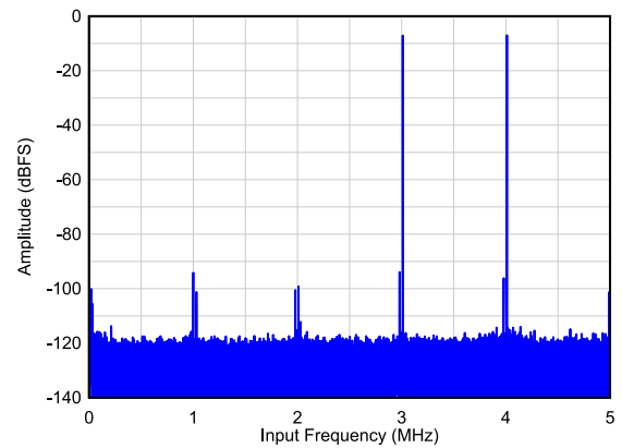
FIG 6-2. Two Tone FFT at F_{IN} = 3,4 MHz
