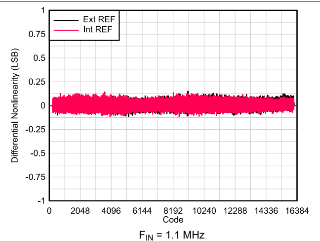
6-12. DNL vs Code
