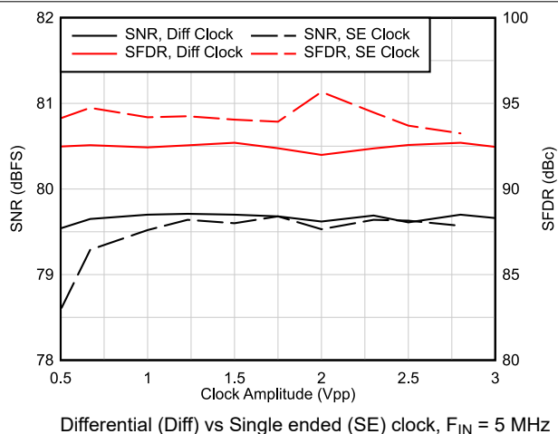
6-52. AC Performance vs Clock Amplitude
