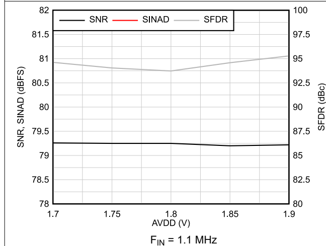
6-9. AC Performance vs AVDD
