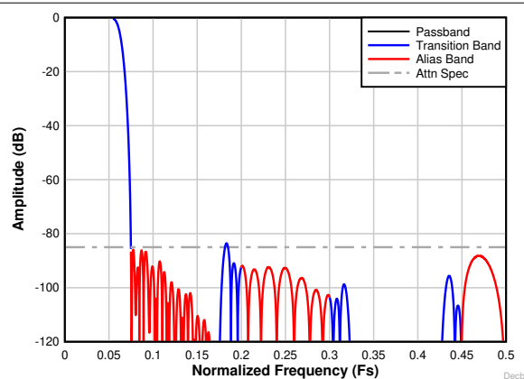
8-29. Decimation by 8 complex frequency response
