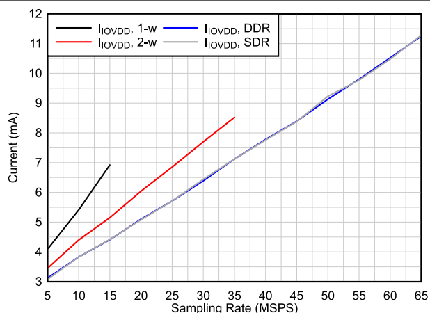
6-62. I_{OVDD} Current vs Output Interface
