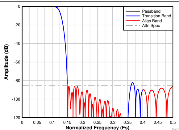
8-27. Decimation by 4 complex frequency response
