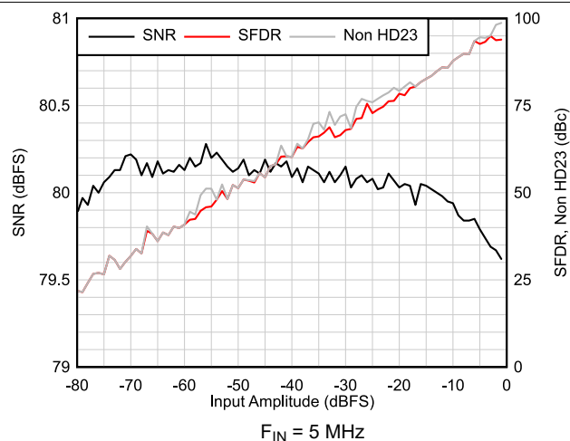
6-27. AC Performance vs Input Amplitude
