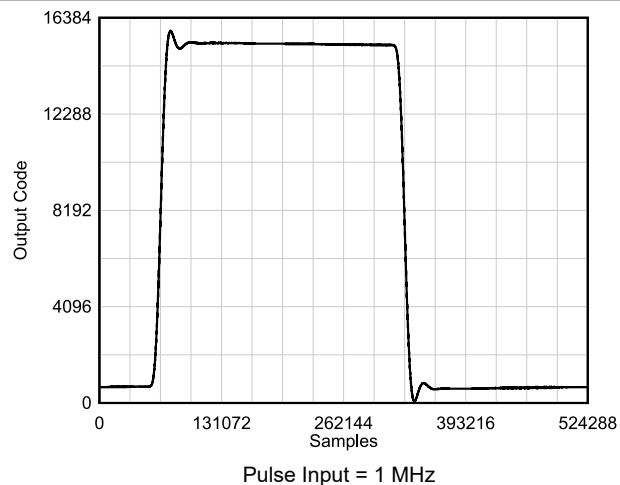
FIG 6-58. Pulse Response
