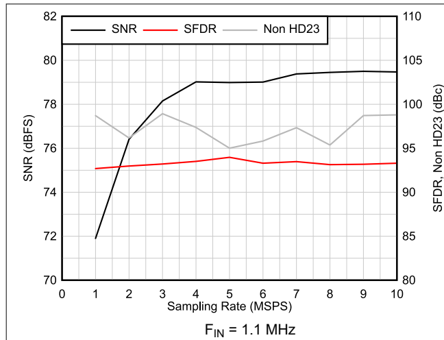
6-7. AC Performance vs Sampling Rate
