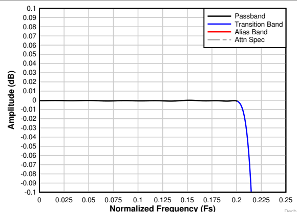
8-26. Decimation by 2 complex passband ripple response
