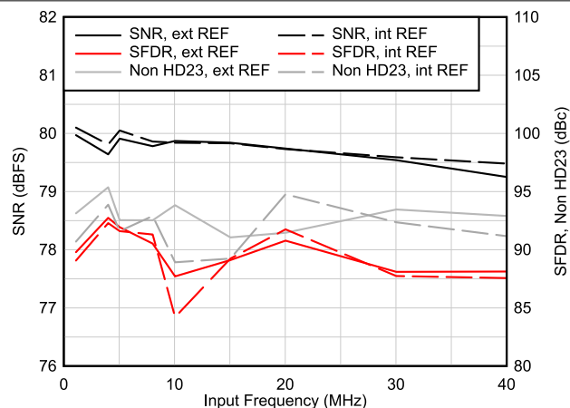
6-25. AC Performance vs Input Frequency
