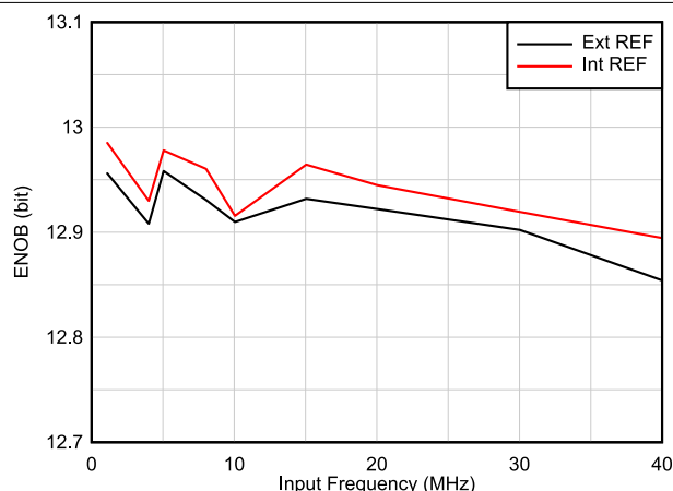
6-26. ENOB vs Input Frequency
