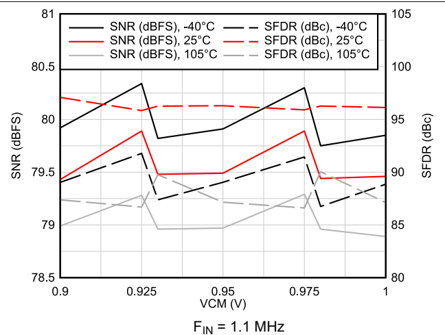
6-10. AC Performance vs VCM vs Temperature
