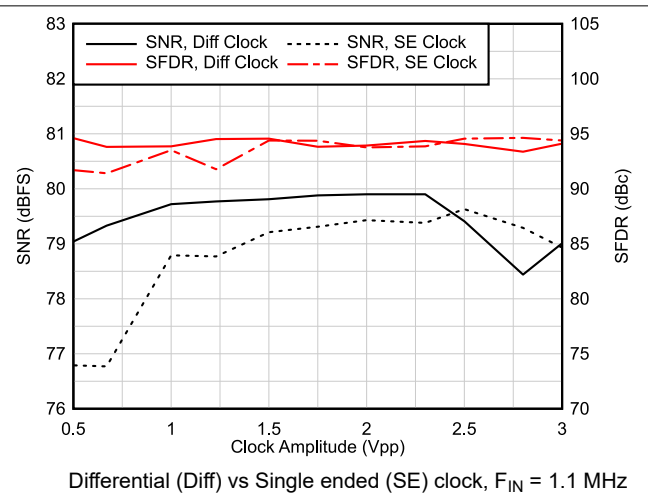
6-8. AC Performance vs Clock Amplitude
