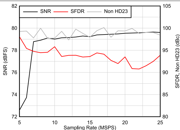
6-28. AC Performance vs Sampling Rate
