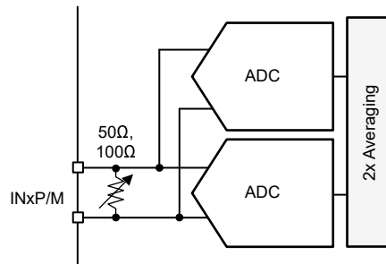
図 6-45. Internal Digital Averaging
