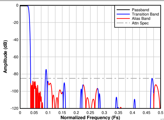
6-28. Complex Decimation by 16 Filter Response
