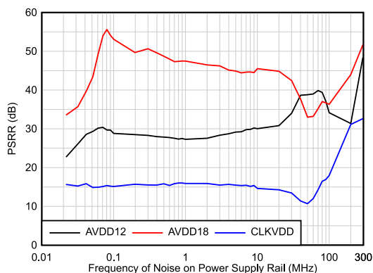
図 7-5. Power supply rejection ratio (PSRR) vs frequency
