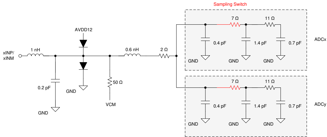
図 6-1. Equivalent input schematic
