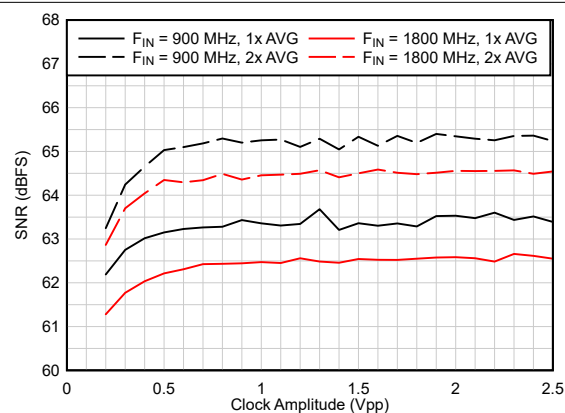
6-13. SNR vs Clock Amplitude (Dither ON)
