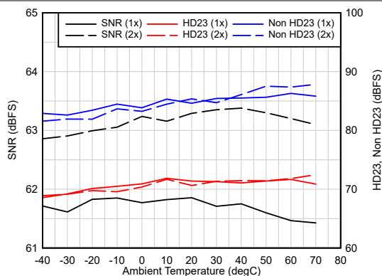
5-35. AC Performance vs Temperature
