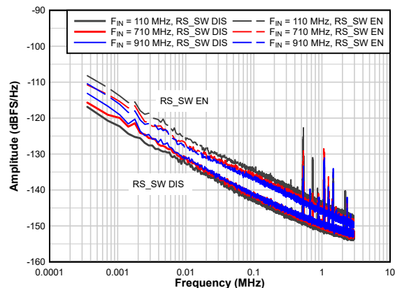
図 6-10. Amplitude Noise vs Input Frequency
