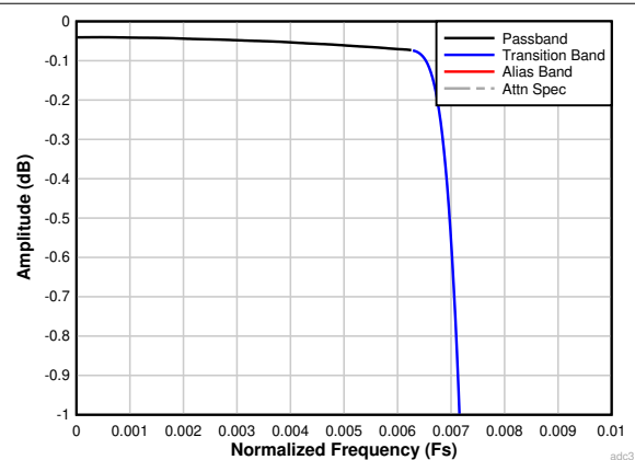
図 6-34. Decimation by 64 Passband Ripple Response
