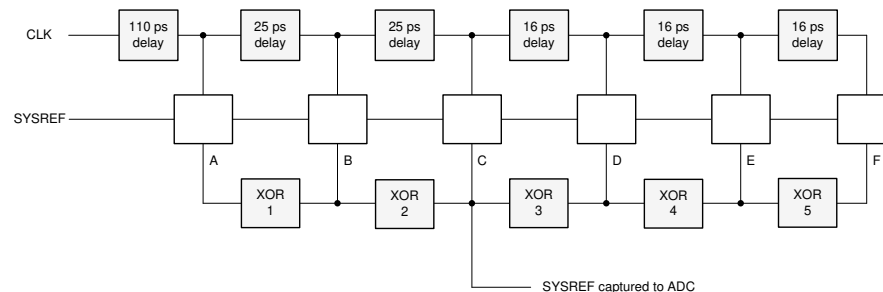
✎ 6-21. SYSREF Detection Circuitry
