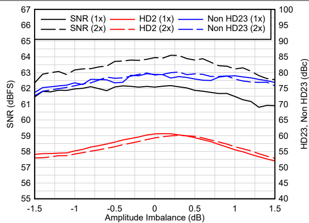
Figure 6-5. Amplitude Imbalance - 3.0 GSPS
