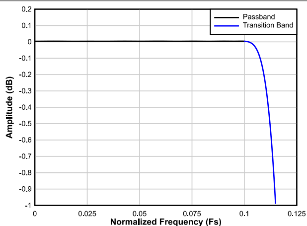
6-25. Decimation by 4 Passband Ripple Response
