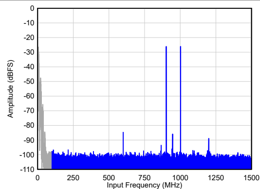
図 5-20. Two Tone FFT at F_{IN} = 900/1000 MHz
