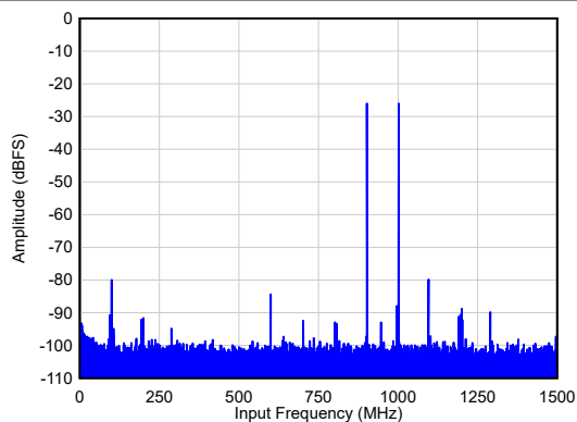
図 5-19. Two Tone FFT at F_{IN} = 900/1000 MHz
