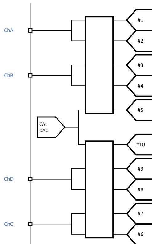
図 6-15. Internal ADC setup for 2x averaging mode
