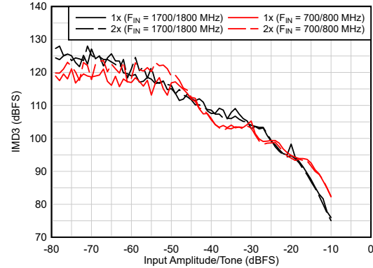
图 5-30. IMD3 Performance vs A_{IN}
