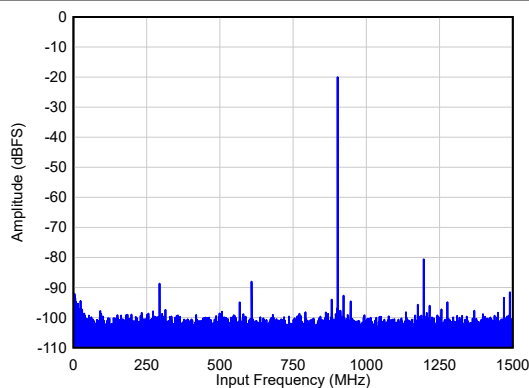
Figure 5-13. Single Tone FFT at F_{IN} = 900 MHz
