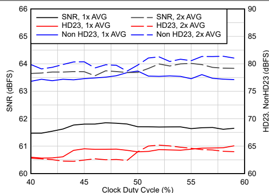
5-36. AC Performance vs Clock Duty Cycle
