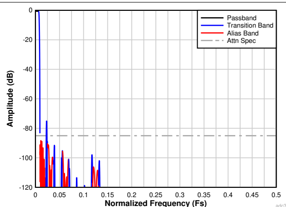
図 6-32. Complex Decimation by 64 Filter Response
