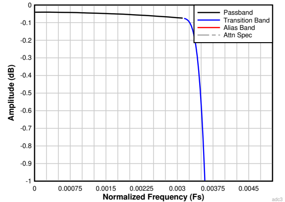
図 6-37. Decimation by 128 Passband Ripple Response
