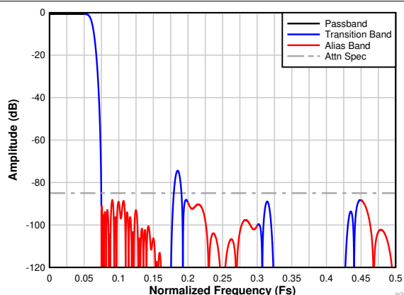
6-26. Complex Decimation by 8 Filter Response
