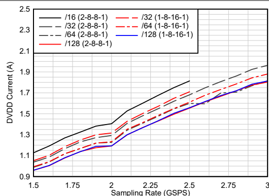
FIG 5-44. Current vs Sampling Rate vs Real Decimation
