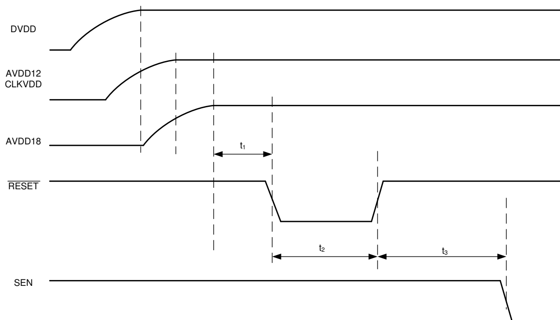
図 7-4. Initialization of serial registers after power up
