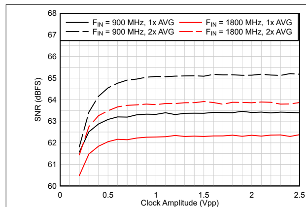
6-12. SNR vs Clock Amplitude (Dither OFF)
