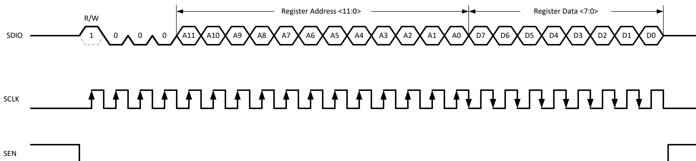
図 6-47. Serial Register Read Timing Diagram
