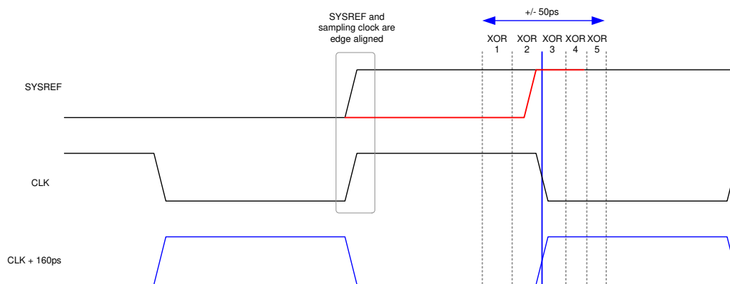
✎ 6-22. Detection of SYSREF Transition within Capture Window
