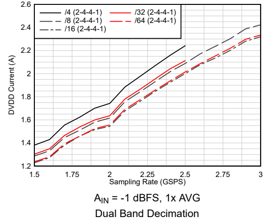
5-48. Current vs Sampling Rate vs Complex Decimation
