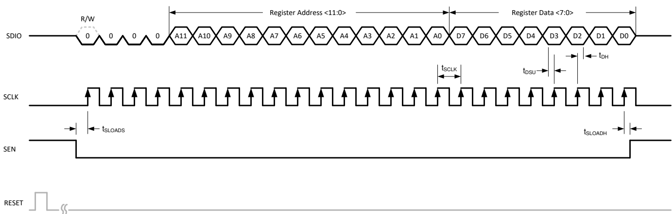
図 6-46. Serial Register Write Timing Diagram
