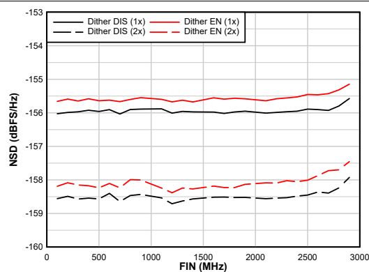
Figure 5-24. AC Performance vs F_{IN}
