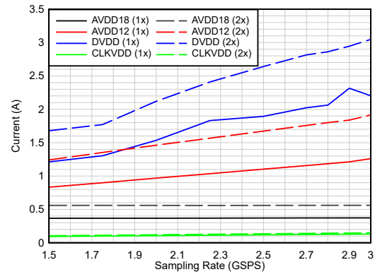
FIG 5-42. Current vs Sampling Rate vs Averaging
