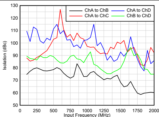
5-37. Isolation vs Input Frequency
