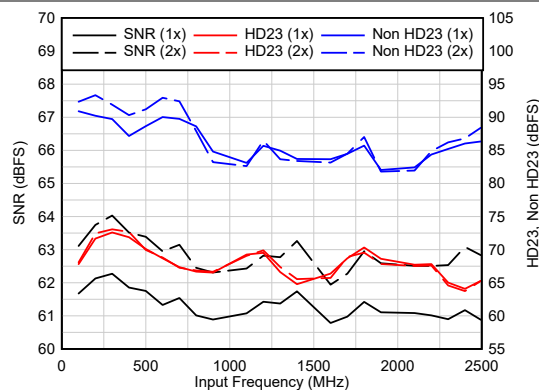
Figure 5-24. AC Performance vs F_{IN}
