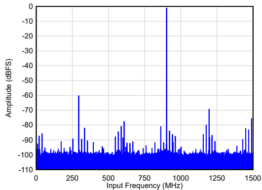
Figure 5-5. Single Tone FFT at F_{IN} = 900 MHz
