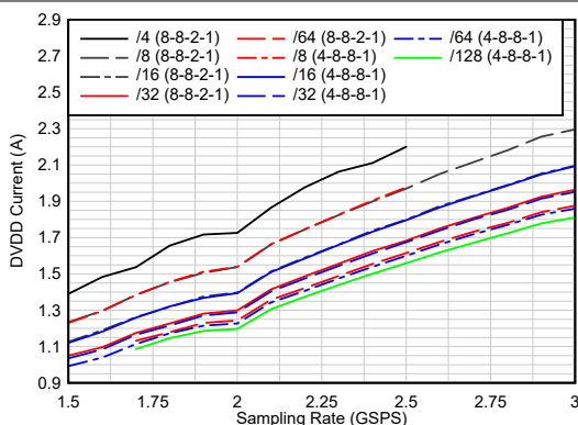
FIG 5-43. Current vs Sampling Rate vs Real Decimation
