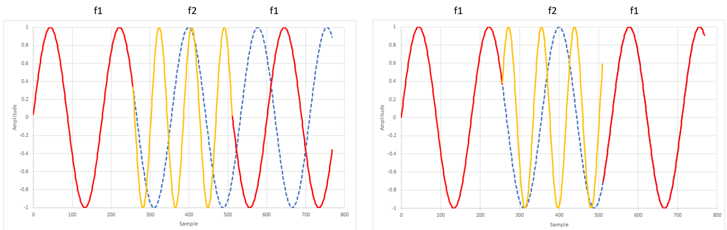
図 6-39. Phase Continuous (left) and Infinite Phase Coherent (right) NCO Frequency Switching
