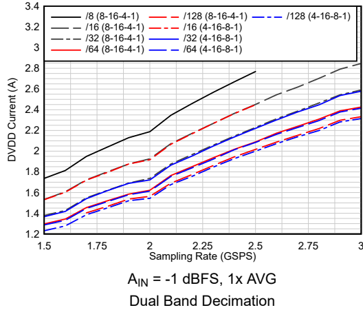
5-47. Current vs Sampling Rate vs Complex Decimation
