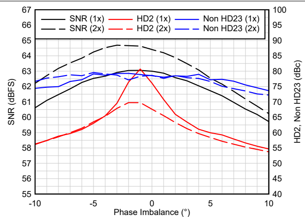
Figure 6-4. Phase Imbalance - 2.6 GSPS
