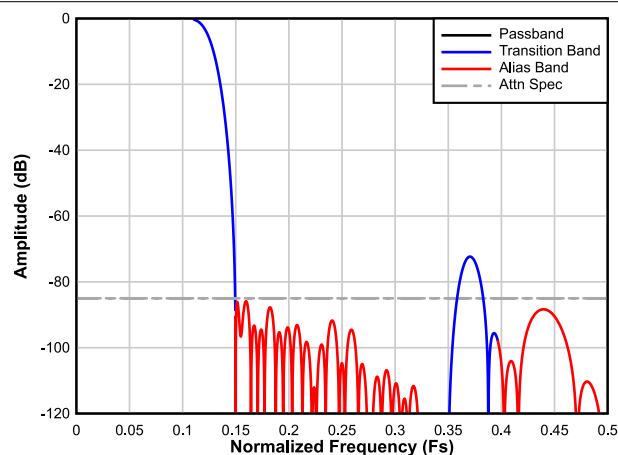
6-24. Complex Decimation by 4 Filter Response
