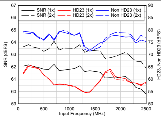
Figure 5-23. AC Performance vs F_{IN}
