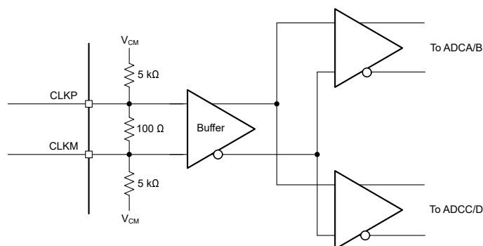
6-14. Clock Input Internal Circuitry
