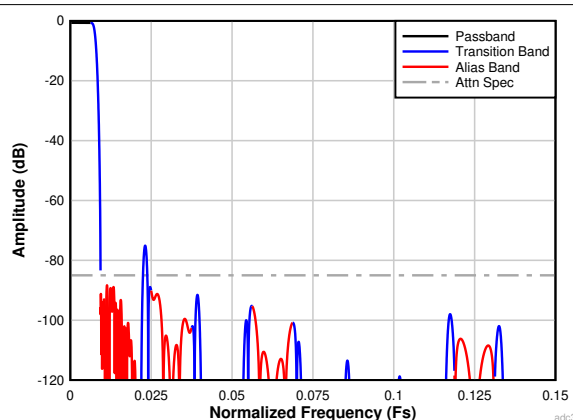
図 6-33. Complex Decimation by 64 Filter Response
