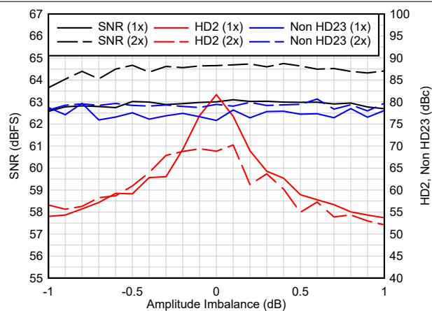
Figure 6-3. Amplitude Imbalance - 2.6 GSPS
