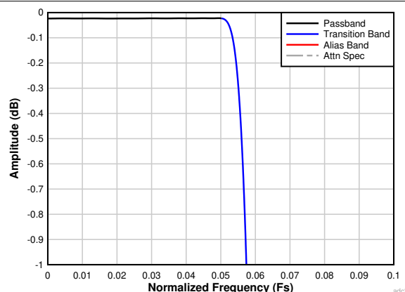
6-27. Decimation by 8 Passband Ripple Response
