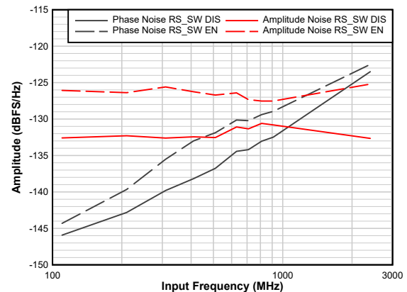
図 6-11. Amplitude and Phase noise at 10 kHz offset vs Input Frequency
