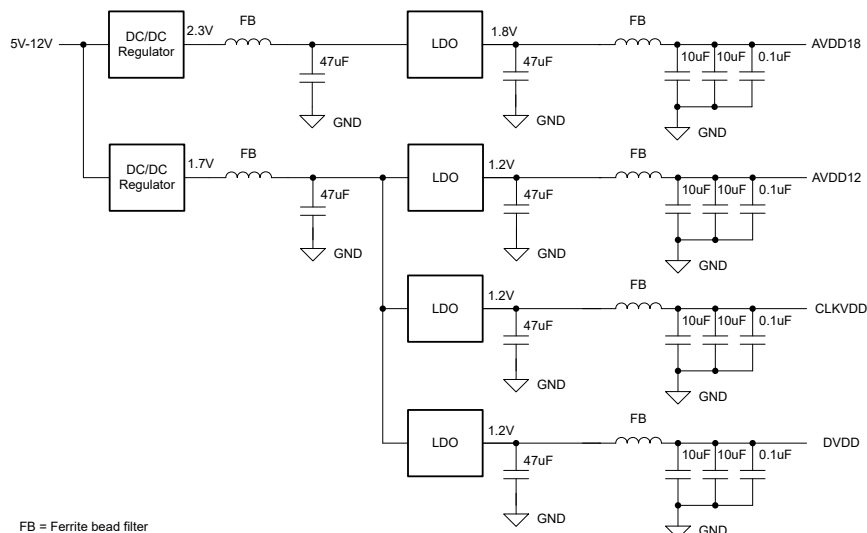
図 7-6. Power supply design example
