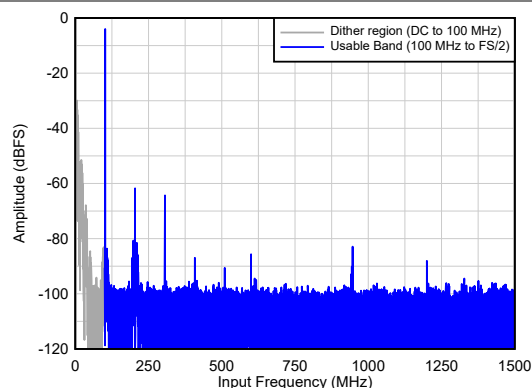
図 5-2. Single Tone FFT at F_{IN} = 100 MHz
