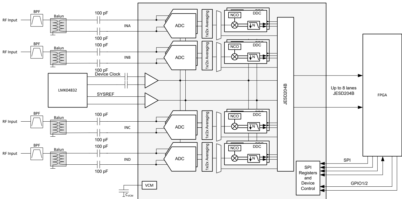
図 7-1. Typical Configuration for Wideband RF Sampling
