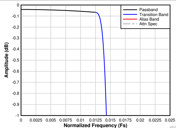
図 6-31. Decimation by 32 Passband Ripple Response
