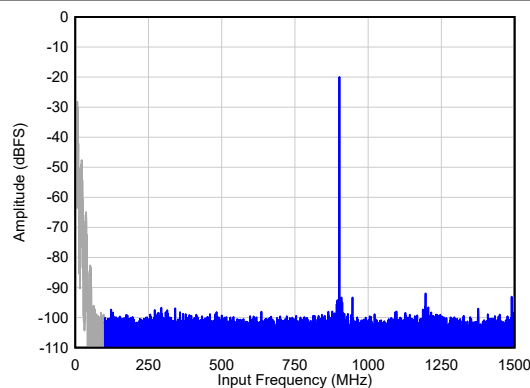
Figure 5-14. Single Tone FFT at F_{IN} = 900 MHz
