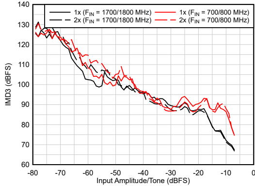
图 5-29. IMD3 Performance vs A_{IN}
