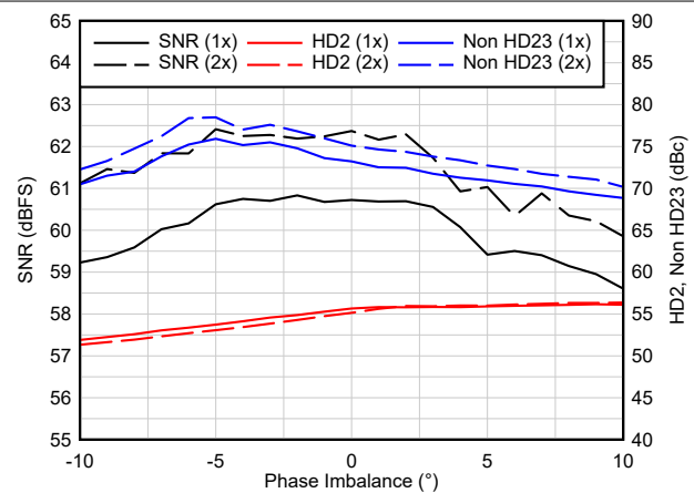
Figure 6-6. Phase Imbalance - 3.0 GSPS
