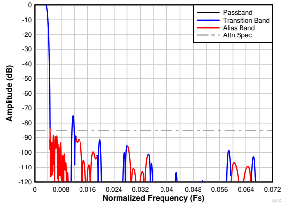
図 6-36. Complex Decimation by 128 Filter Response
