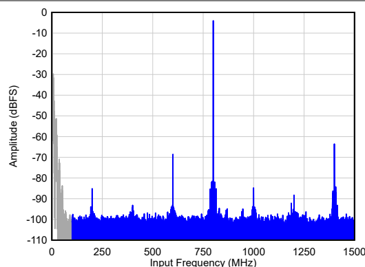
Figure 5-12. Single Tone FFT at F_{IN} = 2200 MHz
