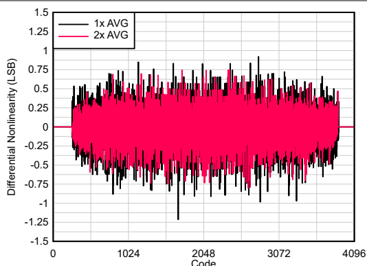
5-39. DNL vs Code
