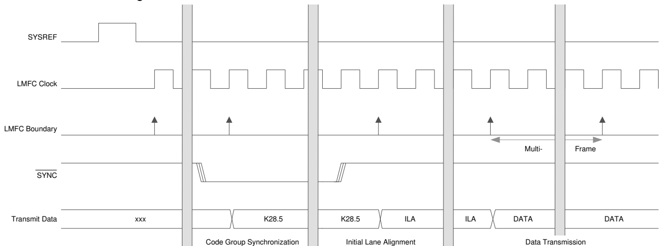
図 6-42. JESD204B Internal Timing Diagram
