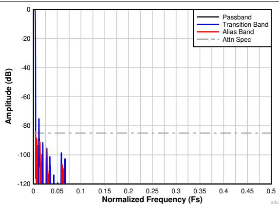
図 6-35. Complex Decimation by 128 Filter Response
