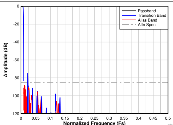
7-29. Complex Decimation by 64 Filter Response
