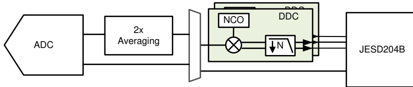
図 7-20. Digital Decimation Filter Options
