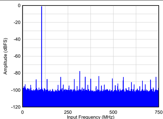
6-1. Single Tone FFT at F_{IN} = 100\text{ MHz}
