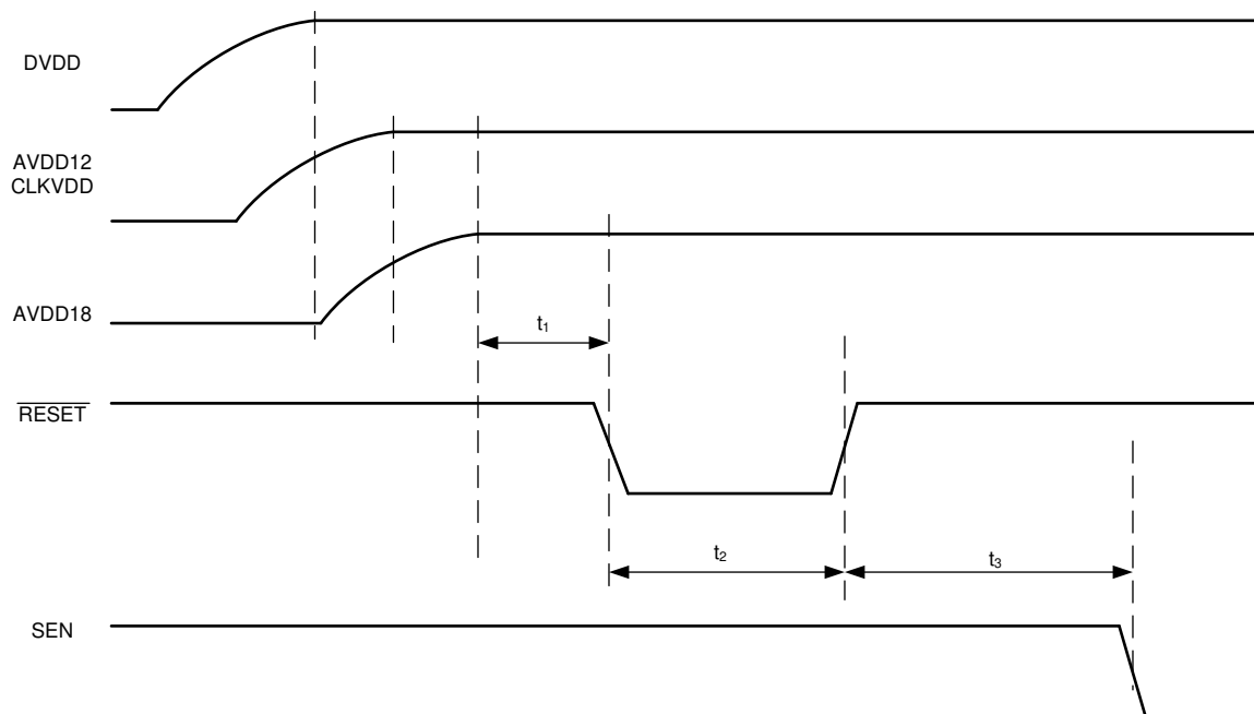
8-8. Initialization of serial registers after power up
