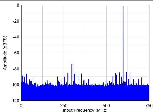
6-3. Single Tone FFT at F_{IN} = 600\text{ MHz}
