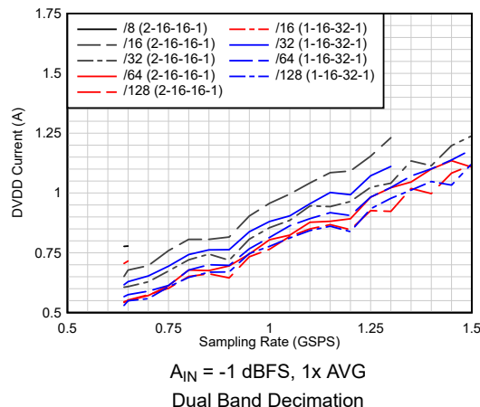
6-50. Current vs Sampling Rate vs Complex Decimation
