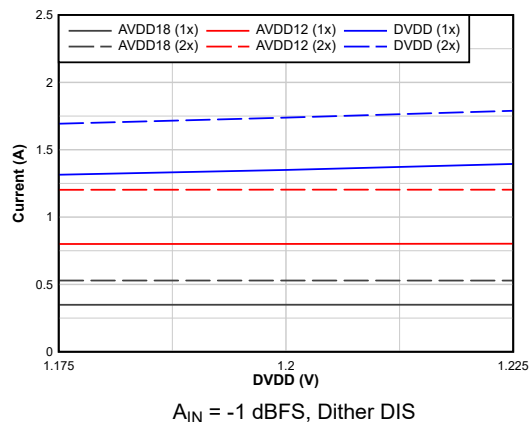
6-53. Current vs DVDD
