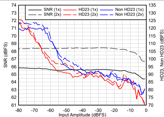
6-27. Dither Spur vs A_{IN}
