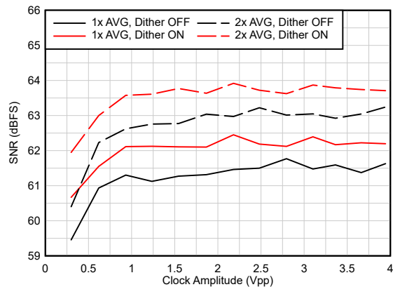
7-9. SNR vs Clock Amplitude ( F_{IN} = 900 MHz)
