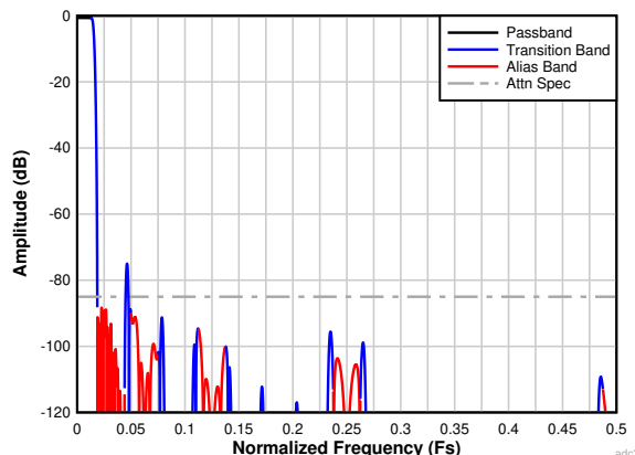
7-27. Complex Decimation by 32 Filter Response
