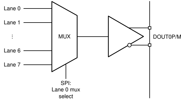
図 7-40. SERDES Output Mux for DOUT0
