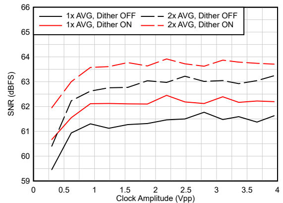
7-10. SNR vs Clock Amplitude ( F_{IN} = 1800 MHz)
