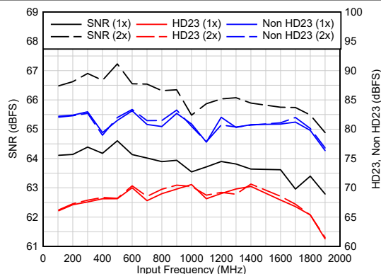
6-25. AC Performance vs F_{IN}
