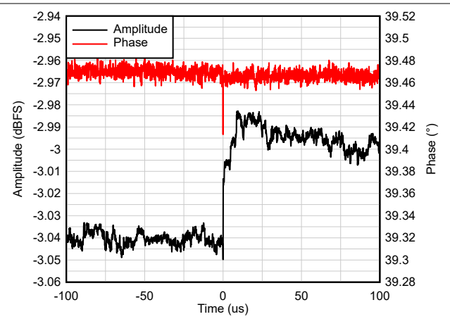
图 7-19. Amplitude and Phase vs Time
