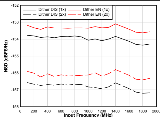
6-26. AC Performance vs F_{IN}
