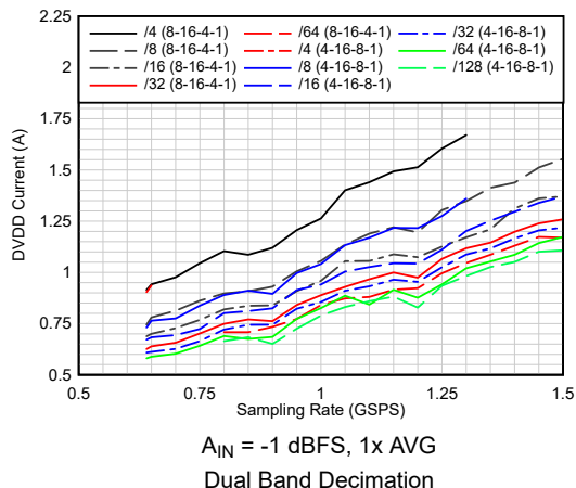
6-49. Current vs Sampling Rate vs Complex Decimation
