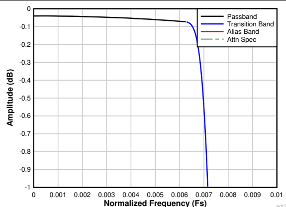
7-31. Decimation by 64 Passband Ripple Response
