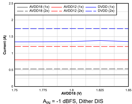
6-51. Current vs AVDD18
