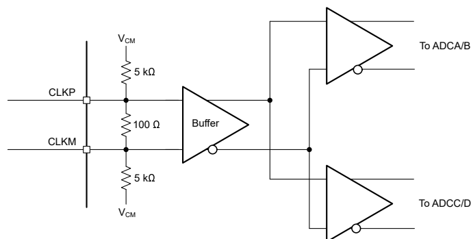
7-11. Clock Input Internal Circuitry
