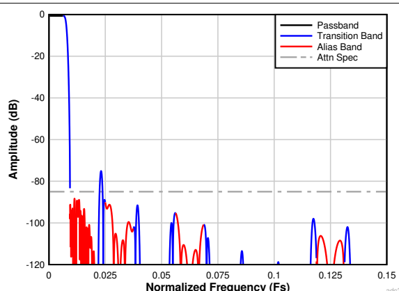
7-30. Complex Decimation by 64 Filter Response
