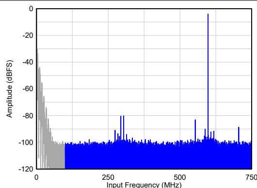
6-4. Single Tone FFT at F_{IN} = 600\text{ MHz}
