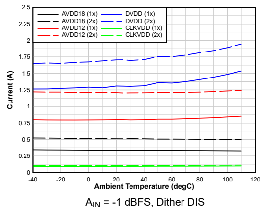
6-54. Current vs Temperature
