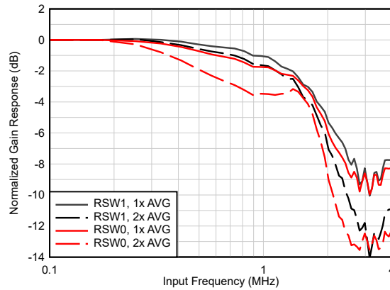
7-2. Full power input bandwidth (100 Ω)
