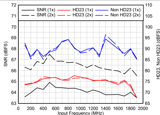
6-26. AC Performance vs F_{IN}
