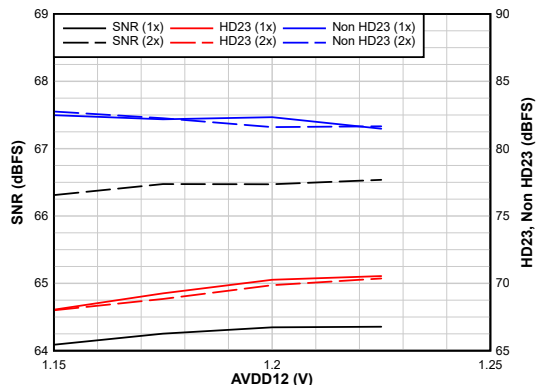
6-37. AC Performance vs AVDD12
