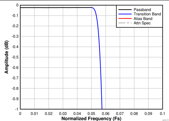
7-24. Decimation by 8 Passband Ripple Response
