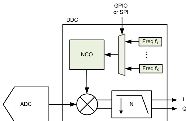
図 7-35. NCO Block Diagram
