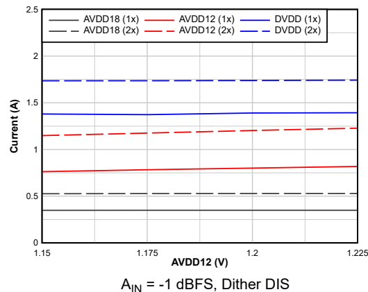
6-52. Current vs AVDD12
