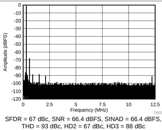
Figure 9. FFT for 450-MHz Input Signal (Dither On)
