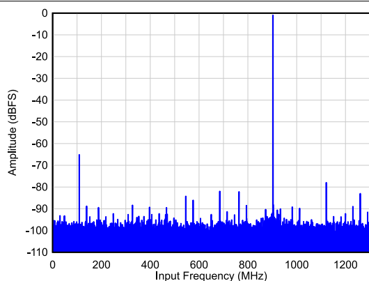
FIG 6-5. Single Tone FFT at F_{IN} = 900 MHz
