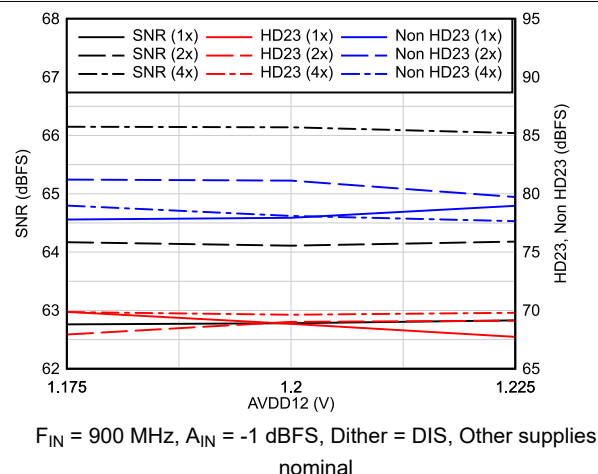
FIG 6-38. AC Performance vs AVDD12
