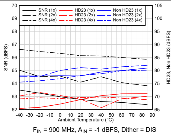
FIG 6-39. AC Performance vs Temperature
