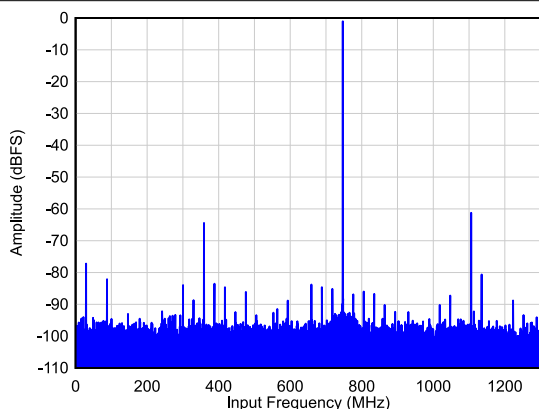
FIG 6-7. Single Tone FFT at F_{IN} = 1400 MHz
