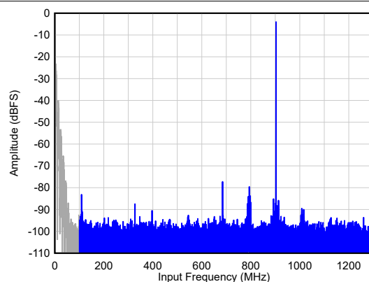
FIG 6-6. Single Tone FFT at F_{IN} = 900 MHz
