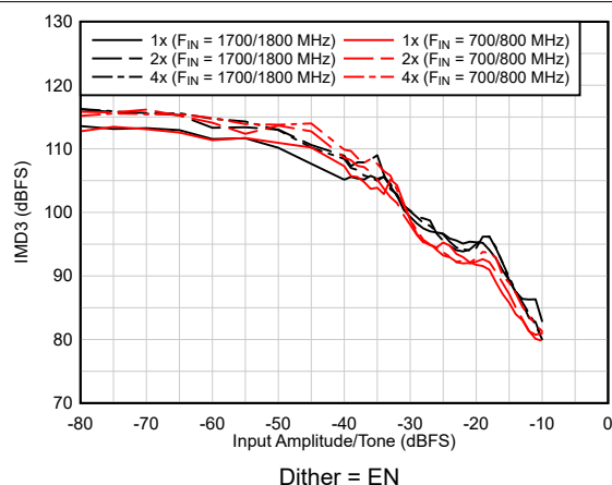
FIG 6-35. IMD3 Performance vs A_{IN}
