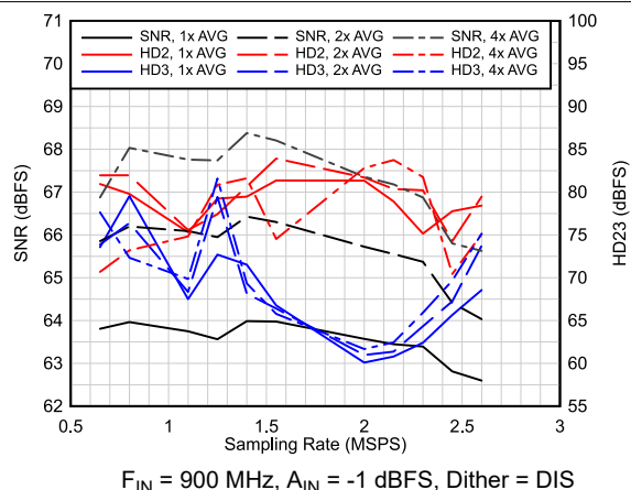
FIG 6-36. AC Performance vs F_s
