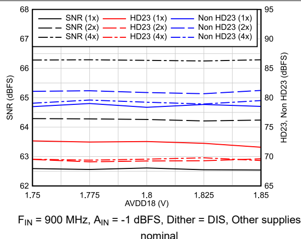
FIG 6-37. AC Performance vs AVDD18
