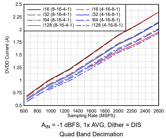
FIG 6-54. Current vs Sampling Rate vs Decimation
