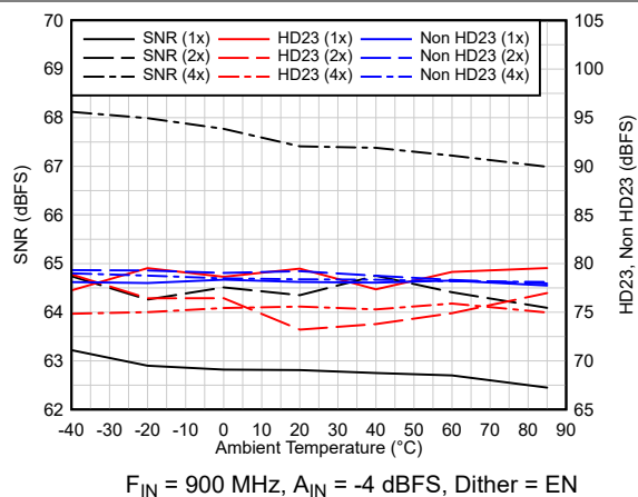
FIG 6-40. AC Performance vs Temperature
