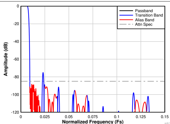
図 7-30. Complex Decimation by 64 Filter Response
