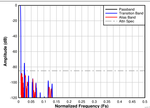
図 7-29. Complex Decimation by 64 Filter Response
