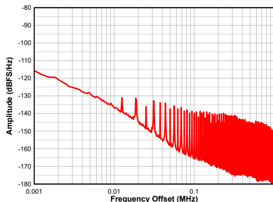
Figure 7-6. Dither Close-Up
