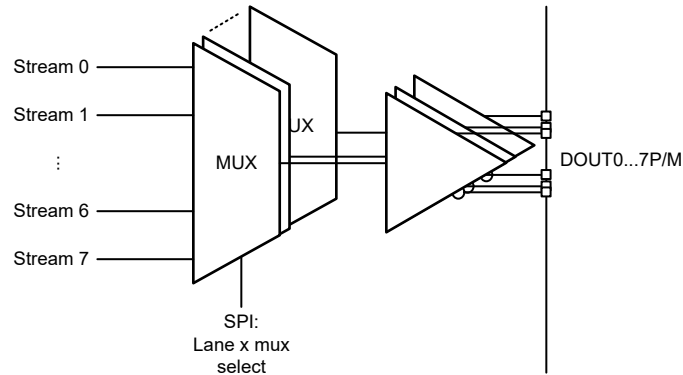
図 7-40. SERDES output mux for DOUT0
