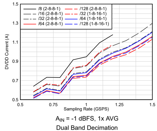
Figure 6-54. Current vs Sampling Rate vs Complex Decimation
