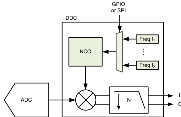
図 7-35. NCO Block Diagram
