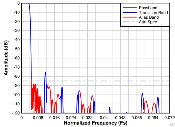
図 7-33. Complex Decimation by 128 Filter Response
