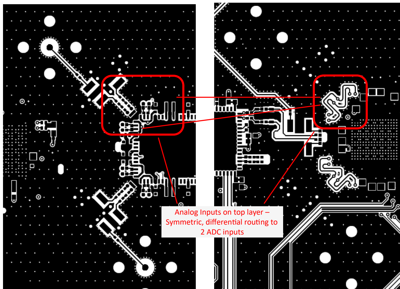
図 8-8. Layout example for 4x AVG: ADC32RF5x EVM
