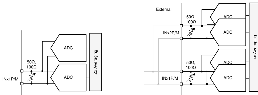
図 7-42. Internal digital averaging (left: 2x, right: 4x)
