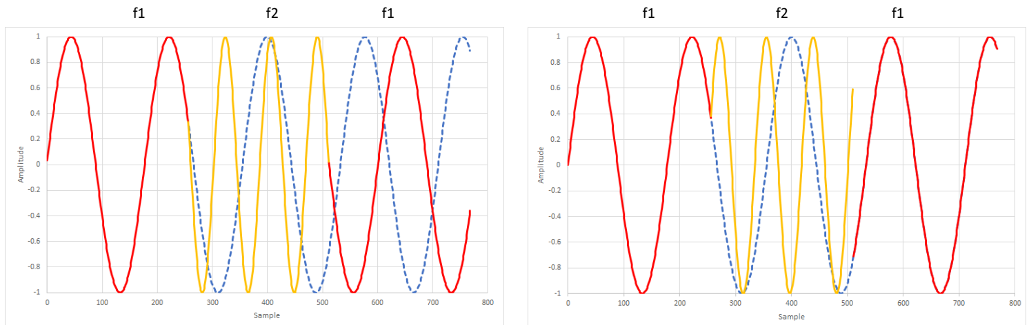
図 7-36. Phase Continuous (left) and Infinite Phase Coherent (right) NCO Frequency Switching
