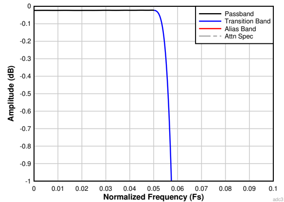
7-24. Decimation by 8 Passband Ripple Response
