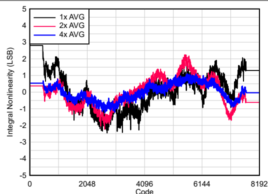
Figure 6-44. INL vs Code
