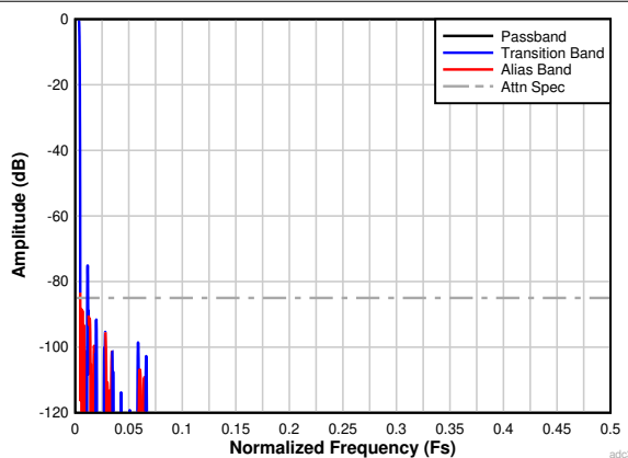
図 7-32. Complex Decimation by 128 Filter Response
