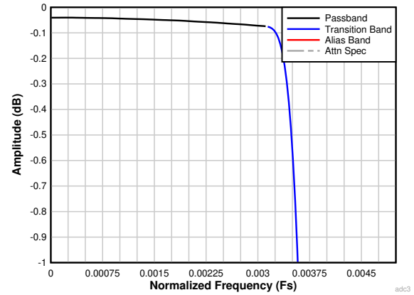
図 7-34. Decimation by 128 Passband Ripple Response
