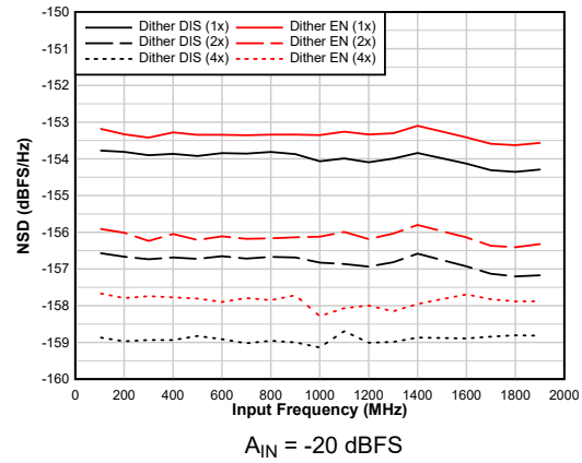
FIG 6-32. NSD Performance vs F_{IN}
