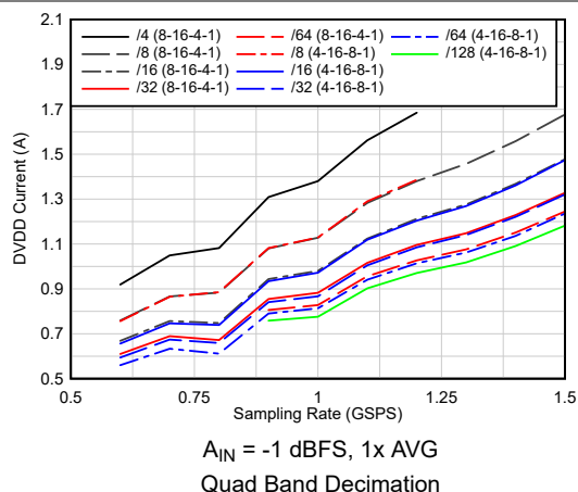
6-55. Current vs Sampling Rate vs Complex Decimation
