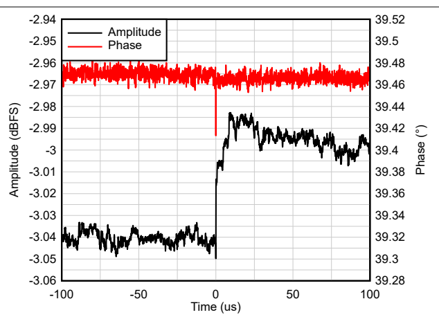
図 7-19. Amplitude and Phase vs Time
