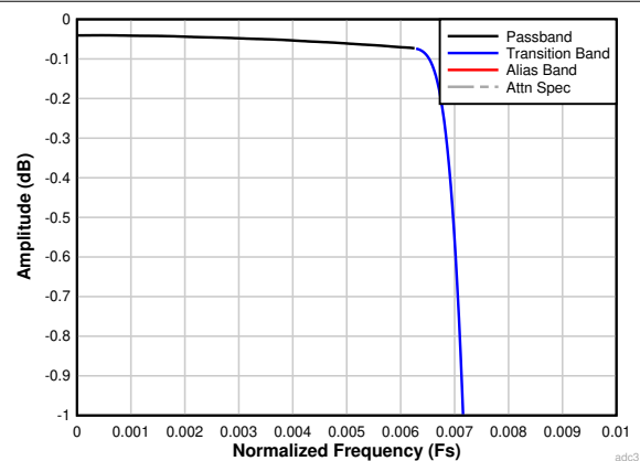
図 7-31. Decimation by 64 Passband Ripple Response
