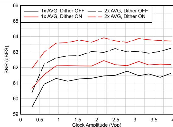
Figure 7-10. SNR vs Clock Amplitude ( F_{IN} = 1800 \text{ MHz} )
