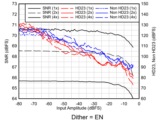
FIG 6-34. AC Performance vs A_{IN}
