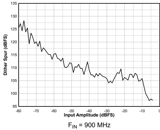
FIG 6-31. Dither Spur vs A_{IN}
