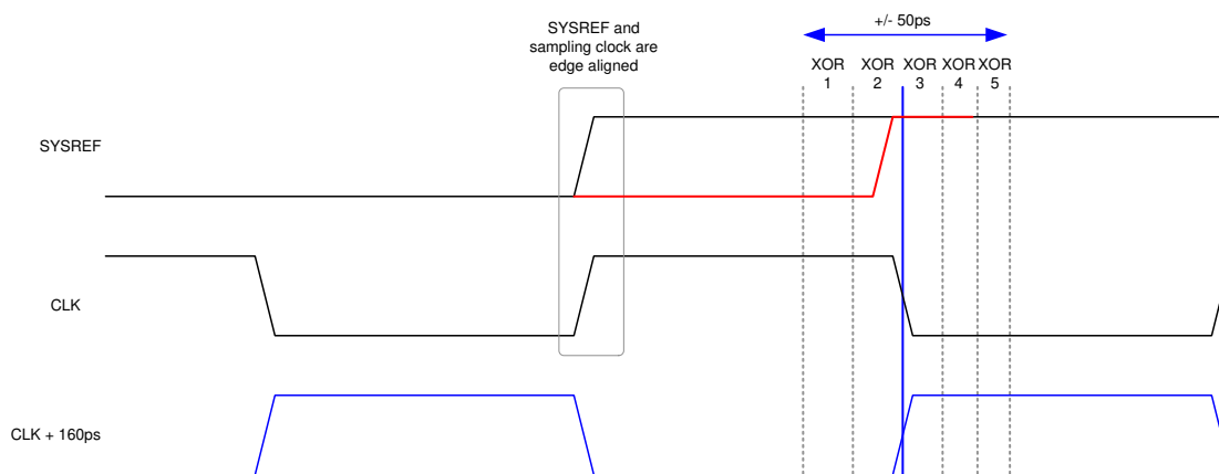
7-14. Detection of SYSREF Transition within Capture Window
