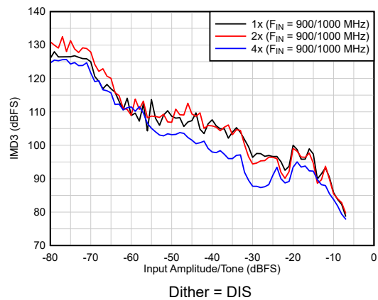
FIG 6-36. IMD3 Performance vs A_{IN}
