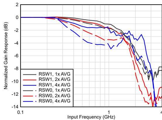
図 7-2. Full power input bandwidth
