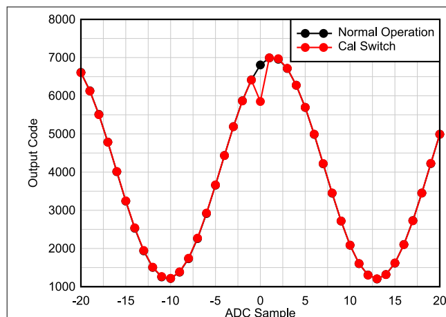
図 7-18. Output Code vs ADC Sample
