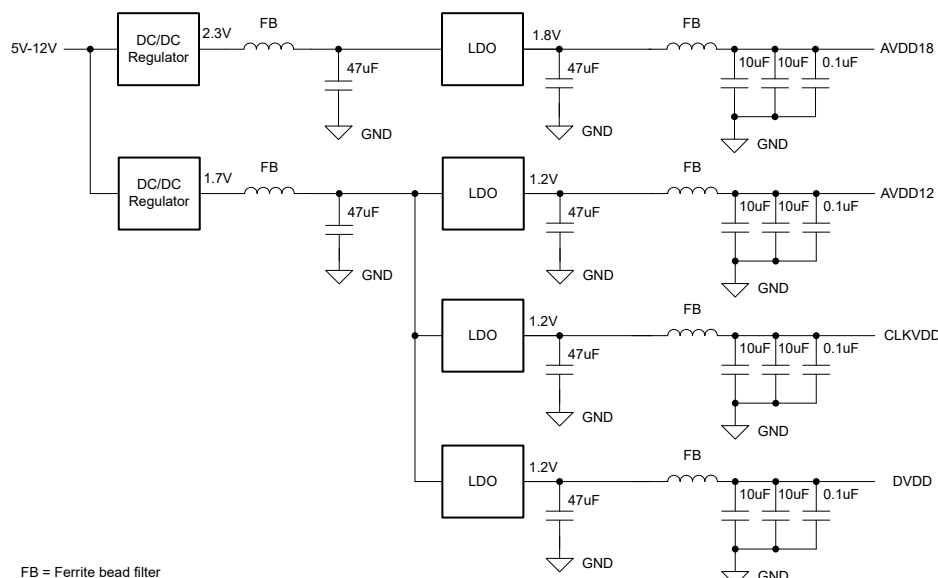
図 8-6. Power supply design example
