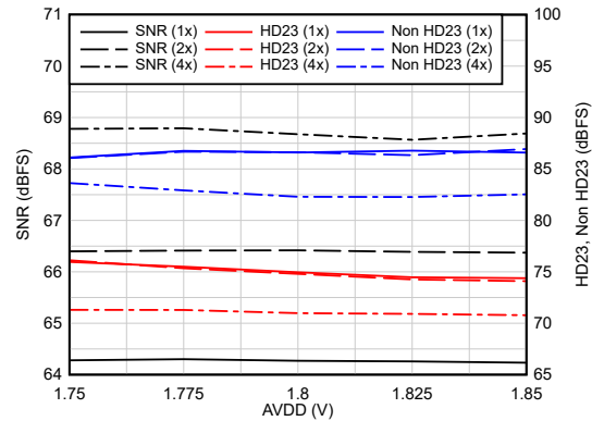
FIG 6-40. AC Performance vs AVDD18
