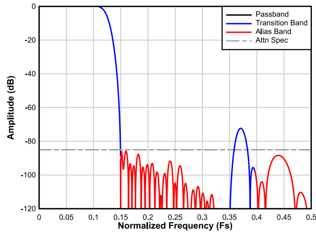
7-21. Complex Decimation by 4 Filter Response
