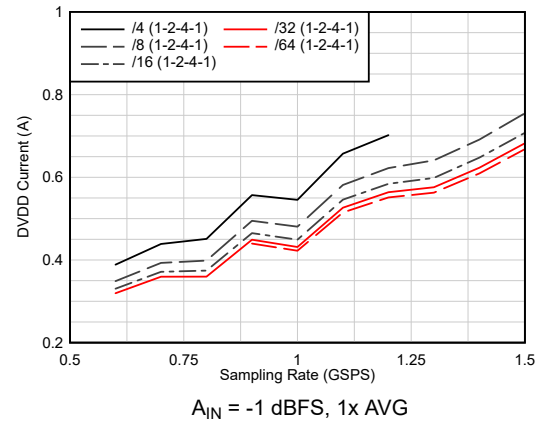
Figure 6-50. Current vs Sampling Rate vs Real Decimation
