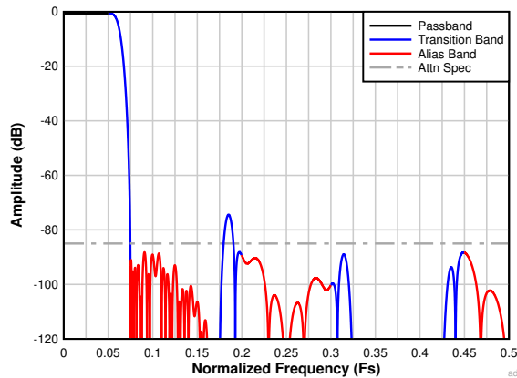
7-23. Complex Decimation by 8 Filter Response
