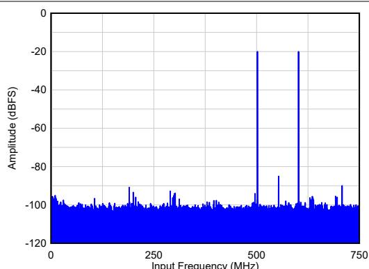
6-21. Two Tone FFT at F_{IN} = 900, 1000 MHz
