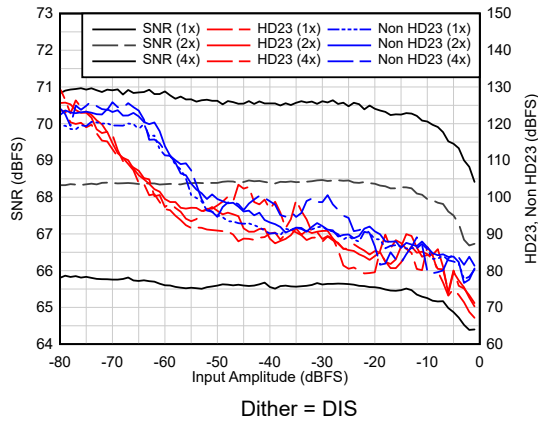
FIG 6-33. AC Performance vs A_{IN}
