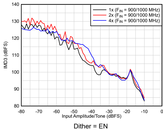
FIG 6-37. IMD3 Performance vs A_{IN}
