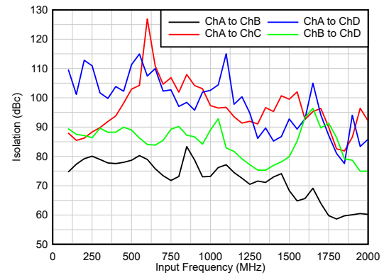
FIG 6-38. Isolation vs Input Frequency
