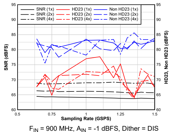
FIG 6-35. AC Performance vs F_S
