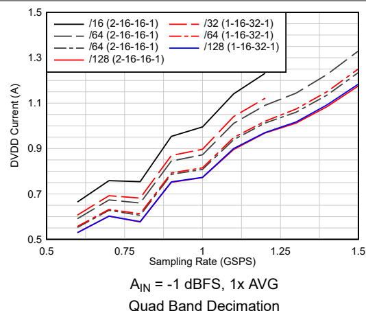
6-56. Current vs Sampling Rate vs Complex Decimation
