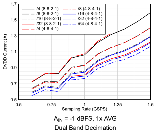
Figure 6-53. Current vs Sampling Rate vs Complex Decimation
