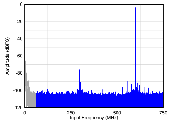
6-14. Single Tone FFT at F_{IN} = 900\text{ MHz}
