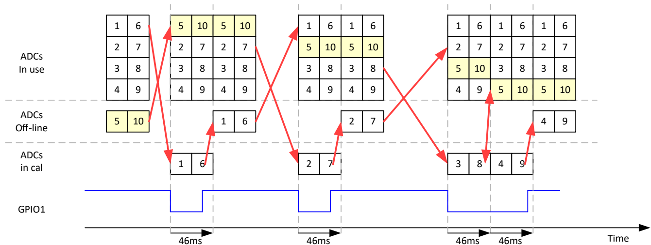
Figure 7-16. Timing diagram - calibration (4x AVG example)
