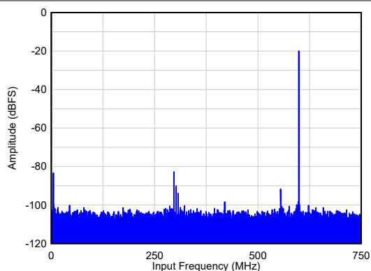
6-19. Single Tone FFT at F_{IN} = 900 MHz
