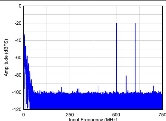
6-22. Two Tone FFT at F_{IN} = 900, 1000 MHz
