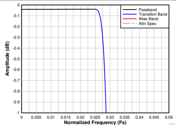
7-26. Decimation by 16 Passband Ripple Response
