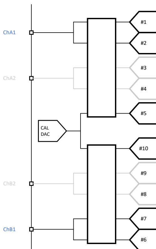
図 7-15. Internal ADC setup for 2x averaging mode
