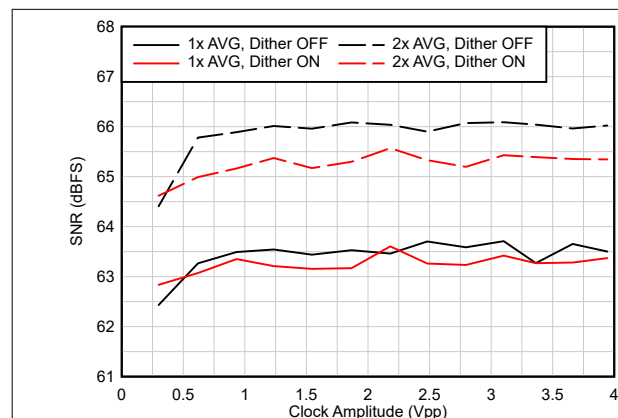
Figure 7-9. SNR vs Clock Amplitude ( F_{IN} = 900 \text{ MHz} )
