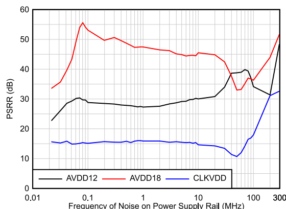
図 8-5. Power supply rejection ratio (PSRR) vs frequency
