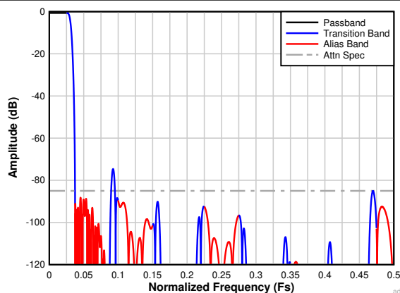
7-25. Complex Decimation by 16 Filter Response
