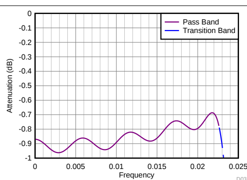
Figure 93. Divide-by-18 Filter Response (Zoomed)
