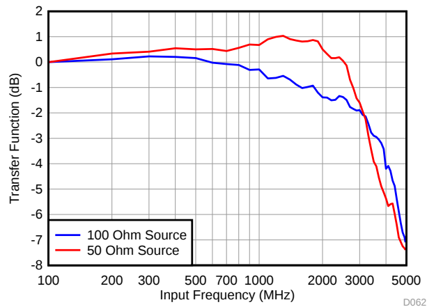
Figure 64. Input Bandwidth with a 100- \Omega Source Resistance
