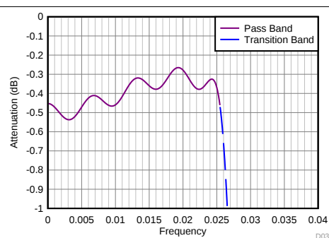
Figure 91. Divide-by-16 Filter Response (Zoomed)
