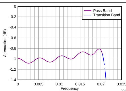
Figure 95. Divide-by-20 Filter Response (Zoomed)
