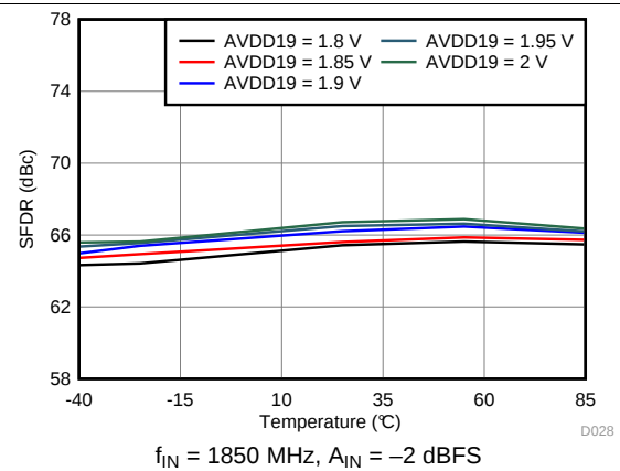
Figure 30. Spurious-Free Dynamic Range vs AVDD19 Supply and Temperature
