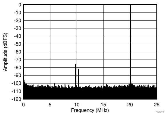
FIG 6-35. FFT for 170-MHz Input Signal (Dither On)
