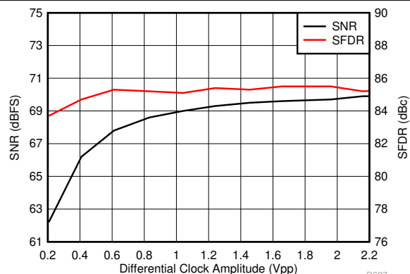
Figure 6-57. Performance vs Differential Clock Amplitude (40 MHz)
