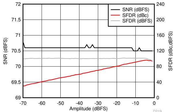
FIG 6-109. Performance vs Input Amplitude (30 MHz)
