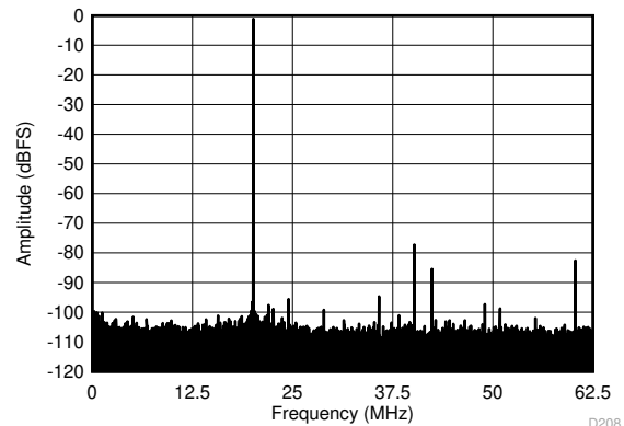
FIG 6-98. FFT for 270-MHz Input Signal (Dither Off)
