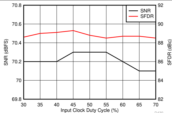
FIG 6-90. Performance vs Clock Duty Cycle (150 MHz)
