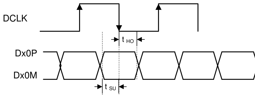
7-3. Setup and Hold Time
