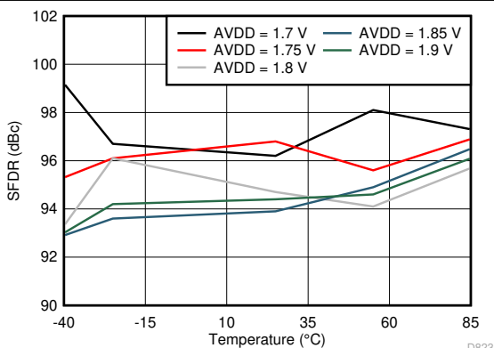
FIG 6-23. Spurious-Free Dynamic Range vs AV_{DD} Supply and Temperature (30 MHz)
