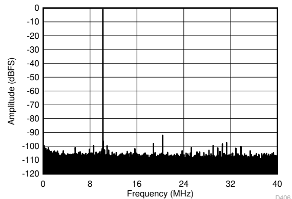
FIG 6-64. FFT for 70-MHz Input Signal (Dither Off)
