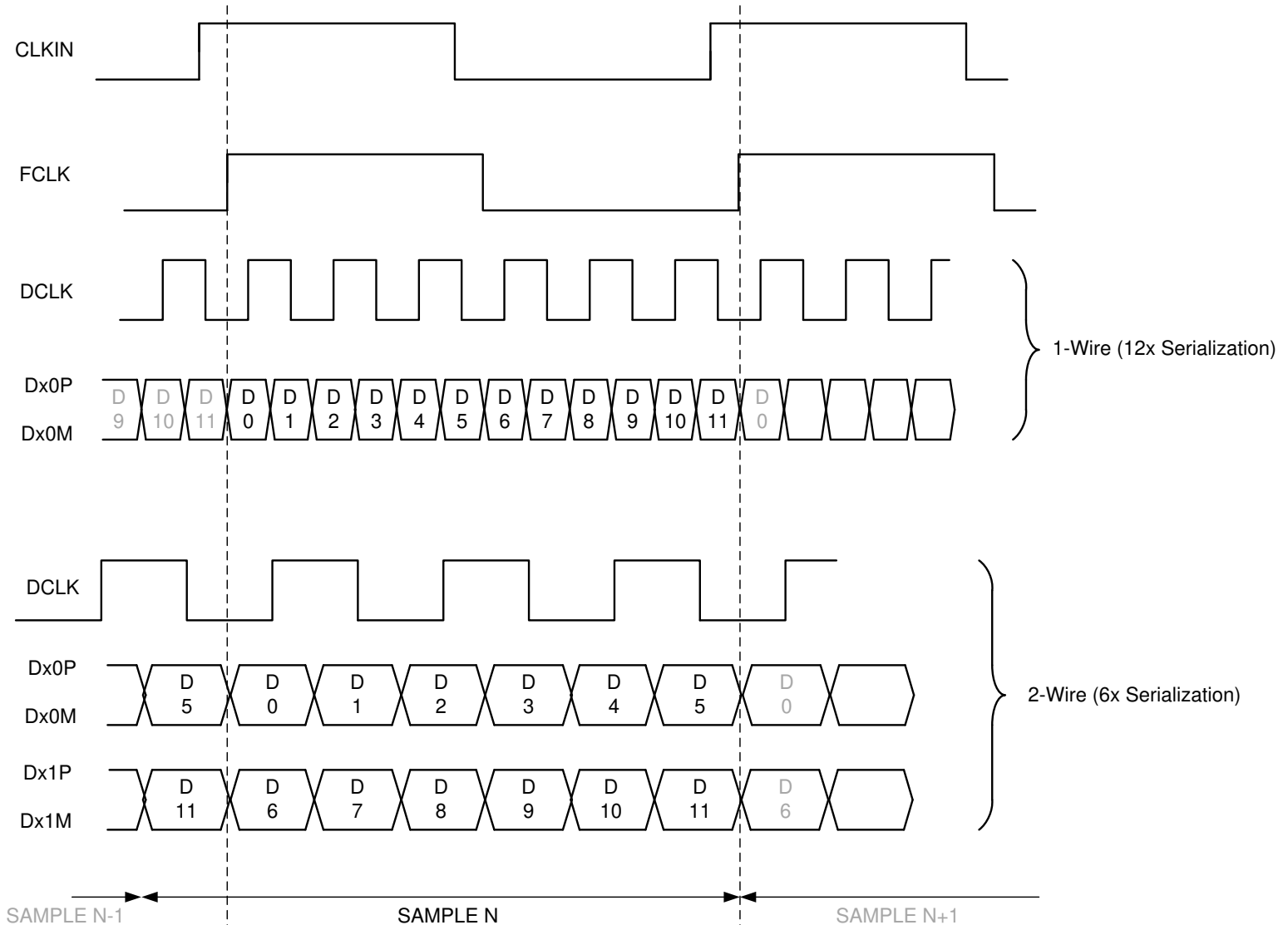
FIG 7-2. Output Timing Diagram
