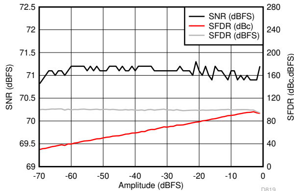
FIG 6-19. Performance vs Input Amplitude (30 MHz)
