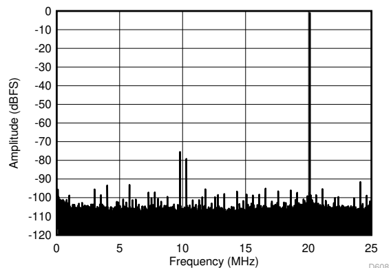
FIG 6-36. FFT for 170-MHz Input Signal (Dither Off)
