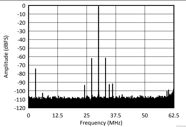
6-122. Common-Mode Rejection Ratio Spectrum
