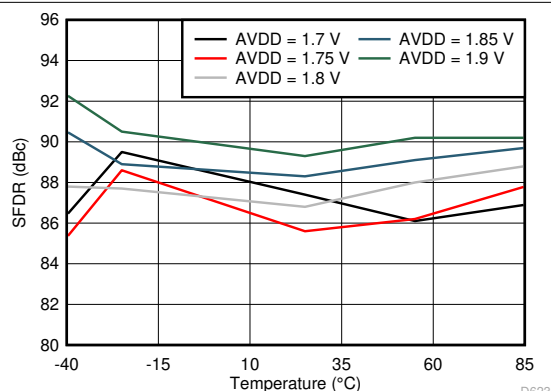
FIG 6-53. Spurious-Free Dynamic Range vs AVDD Supply and Temperature (30 MHz)
