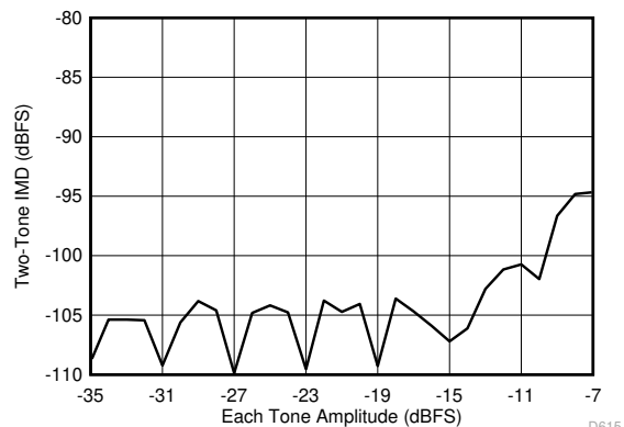
FIG 6-45. Intermodulation Distortion vs Input Amplitude (46 MHz and 50 MHz)
