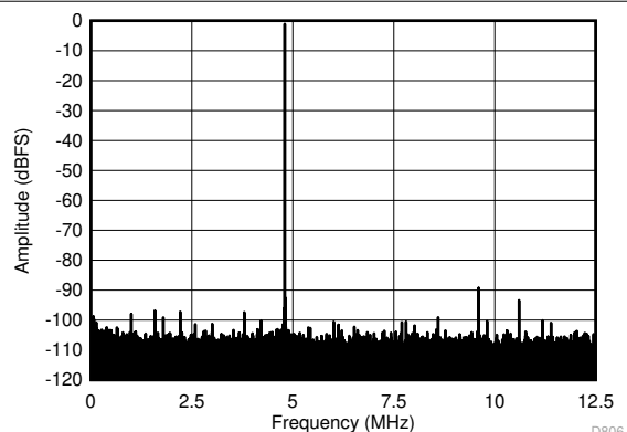
FIG 6-4. FFT for 70-MHz Input Signal (Dither Off)
