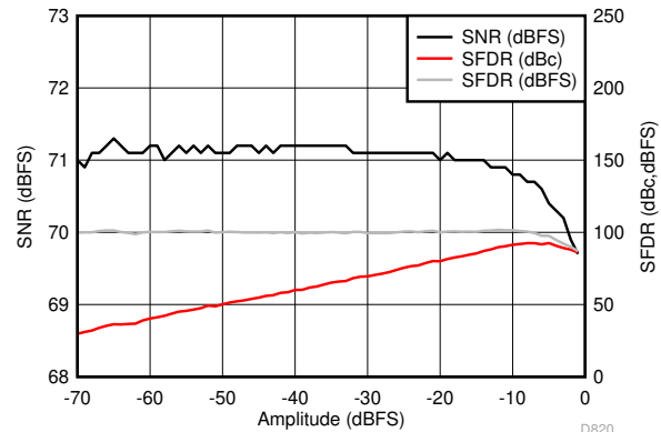
FIG 6-20. Performance vs Input Amplitude (170 MHz)
