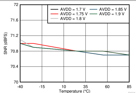
FIG 6-54. Signal-to-Noise Ratio vs AVDD Supply and Temperature (30 MHz)
