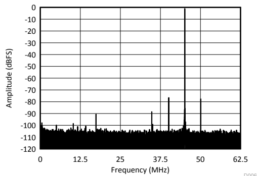
6-122. Common-Mode Rejection Ratio Spectrum
