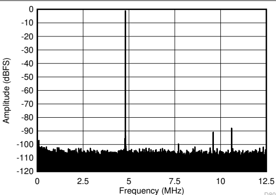
FIG 6-3. FFT for 70-MHz Input Signal (Dither On)
