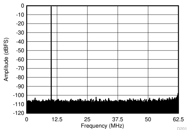
9-4. Performance FFT at 10 MHz (Low Input Frequency)
