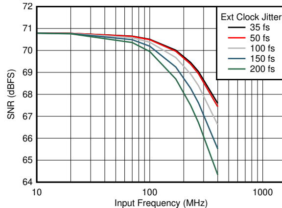
Figure 8-7. SNR vs Frequency for Different Clock Jitter
