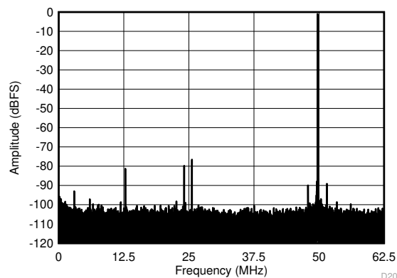
FIG 6-97. FFT for 270-MHz Input Signal (Dither On)
