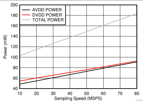
6-125. Power vs Sampling Speed (One-Wire Mode)
