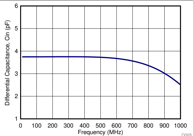
☒ 9-2. Differential Input Capacitance ( C_{IN} )
