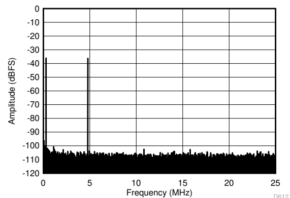
FIG 6-40. FFT for 450-MHz Input Signal (Dither Off)
