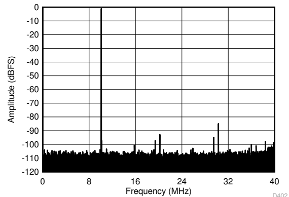
FIG 6-62. FFT for 10-MHz Input Signal (Dither Off)
