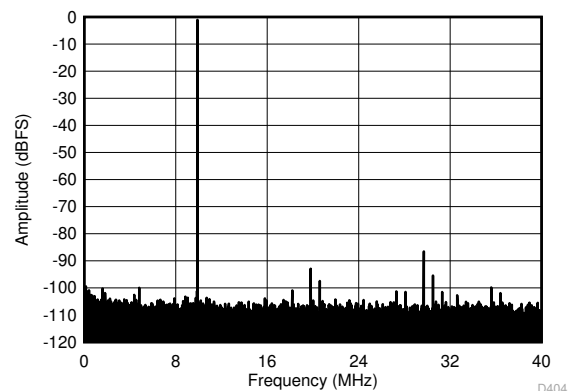
FIG 6-62. FFT for 10-MHz Input Signal (Dither Off)
