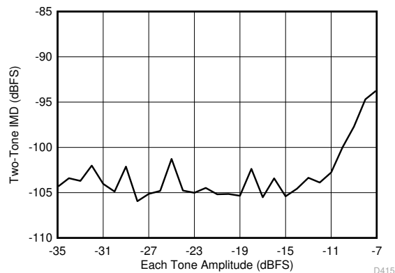
FIG 6-75. Intermodulation Distortion vs Input Amplitude (46 MHz and 50 MHz)
