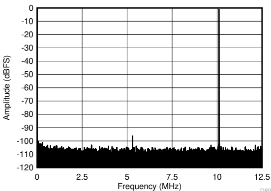
FIG 6-1. FFT for 10-MHz Input Signal (Dither On)
