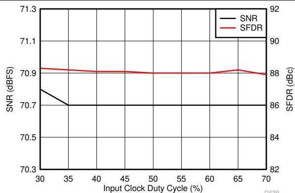
FIG 6-89. Performance vs Clock Duty Cycle (30 MHz)
