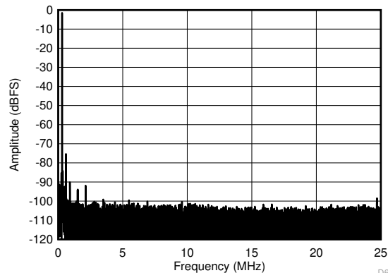
FIG 6-39. FFT for 450-MHz Input Signal (Dither On)
