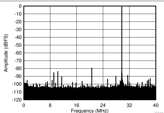
FIG 6-68. FFT for 270-MHz Input Signal (Dither Off)
