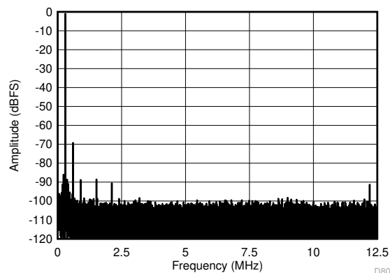
FIG 6-7. FFT for 270-MHz Input Signal (Dither On)
