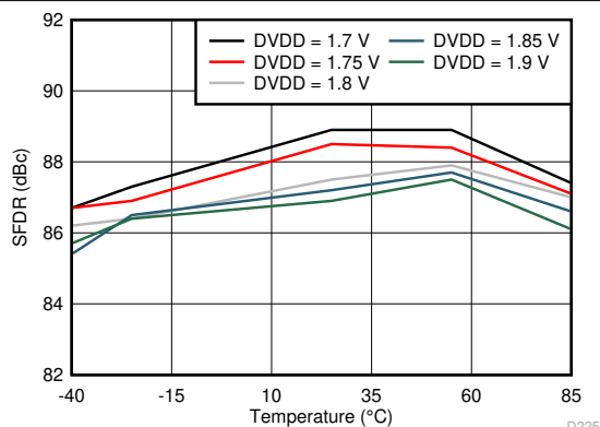
FIG 6-115. Spurious-Free Dynamic Range vs DVDD Supply and Temperature (170 MHz)
