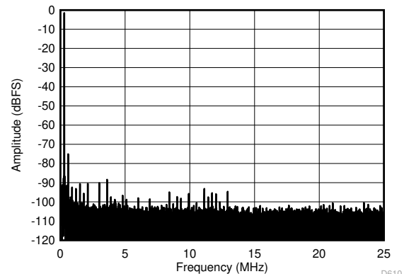
FIG 6-40. FFT for 450-MHz Input Signal (Dither Off)
