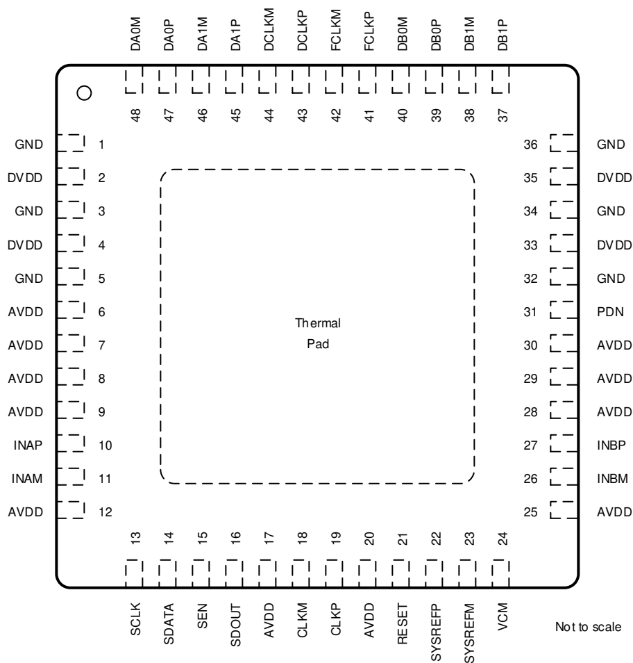
5-1. RGZ Package, 48-Pin VQFN (Top View)
