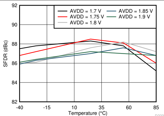
FIG 6-113. Spurious-Free Dynamic Range vs AVDD Supply and Temperature (170 MHz)
