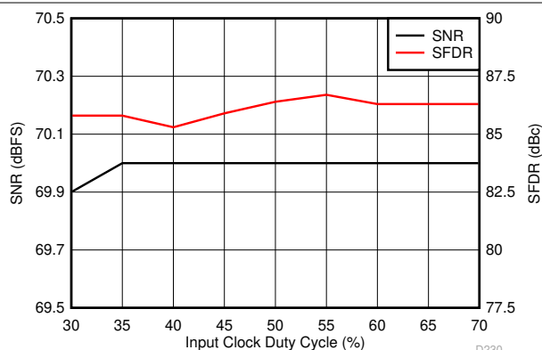
FIG 6-120. Performance vs Clock Duty Cycle (150 MHz)
