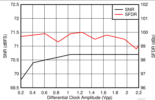
FIG 6-87. Performance vs Differential Clock Amplitude (40 MHz)
