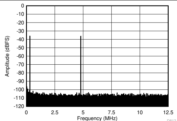
FIG 6-10. FFT for 450-MHz Input Signal (Dither Off)
