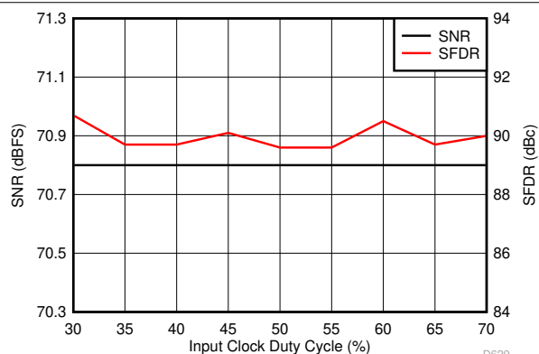
Figure 6-59. Performance vs Clock Duty Cycle (30 MHz)
