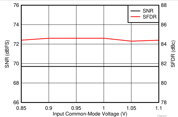
FIG 6-22. Performance vs Input Common-Mode Voltage (170 MHz)
