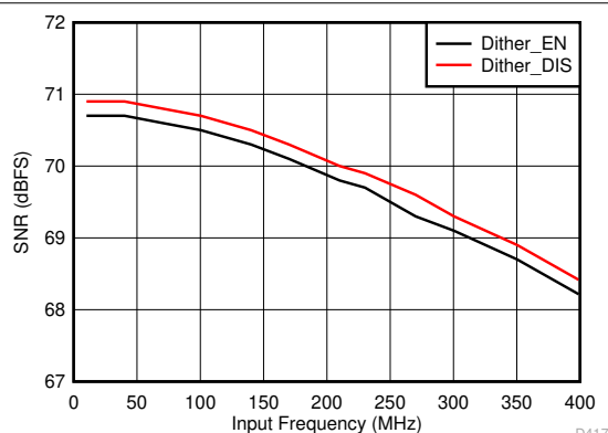
FIG 6-77. Signal-to-Noise Ratio vs Input Frequency
