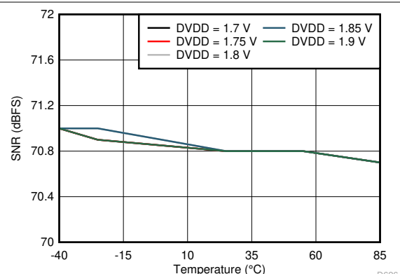
FIG 6-56. Signal-to-Noise Ratio vs DVDD Supply and Temperature (30 MHz)
