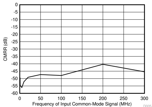
6-121. Common-Mode Rejection Ratio vs Common-Mode Signal Frequency
