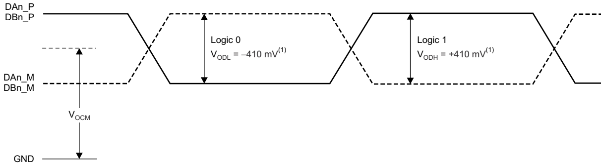
FIG 7-1. Serial LVDS Output Voltage Levels
