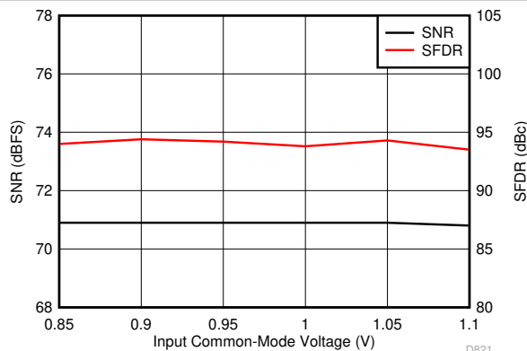
FIG 6-21. Performance vs Input Common-Mode Voltage (30 MHz)
