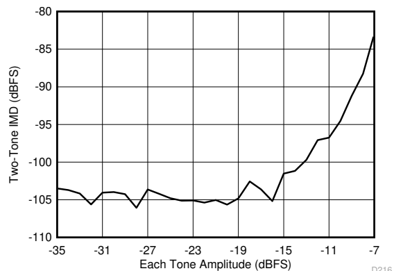
FIG 6-106. Intermodulation Distortion vs Input Amplitude (185 MHz and 190 MHz)
