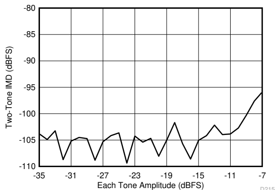
FIG 6-105. Intermodulation Distortion vs Input Amplitude (46 MHz and 50 MHz)
