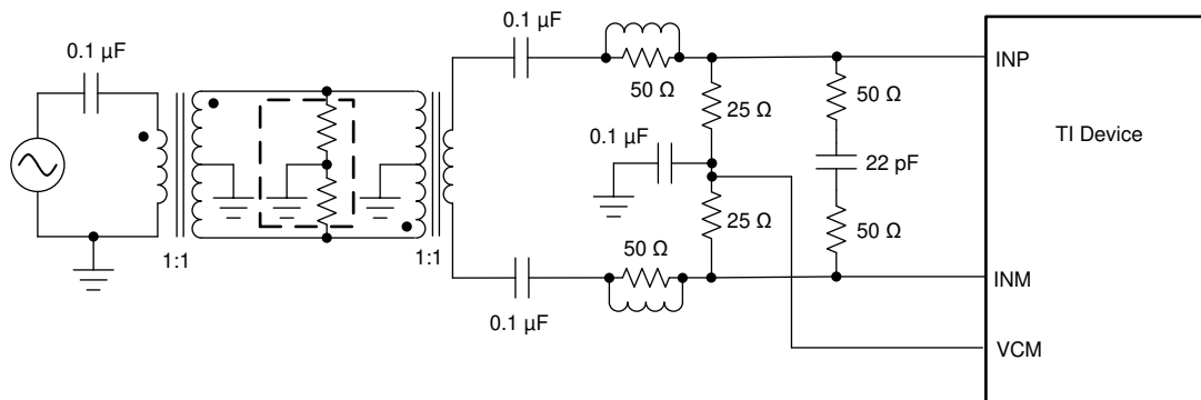
9-3. Driving Circuit for Low Input Frequencies
