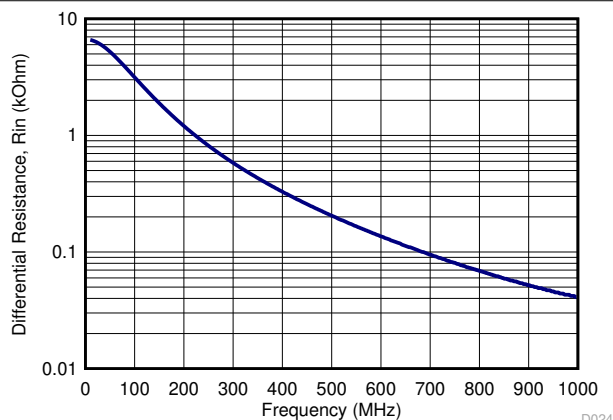
☒ 9-1. Differential Input Resistance ( R_{IN} )
