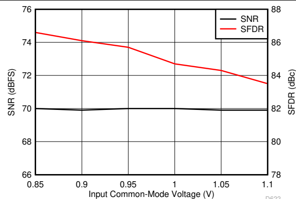
FIG 6-52. Performance vs Input Common-Mode Voltage (170 MHz)
