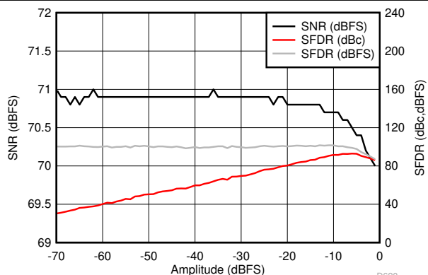
FIG 6-50. Performance vs Input Amplitude (170 MHz)
