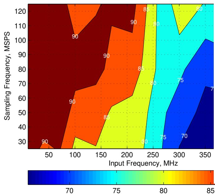
Figure 6-126. Spurious-Free Dynamic Range (SFDR)
