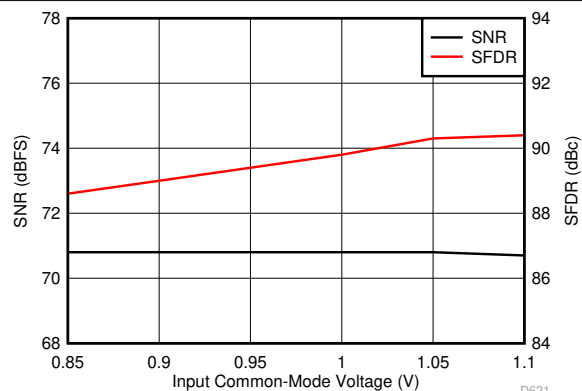
FIG 6-51. Performance vs Input Common-Mode Voltage (30 MHz)
