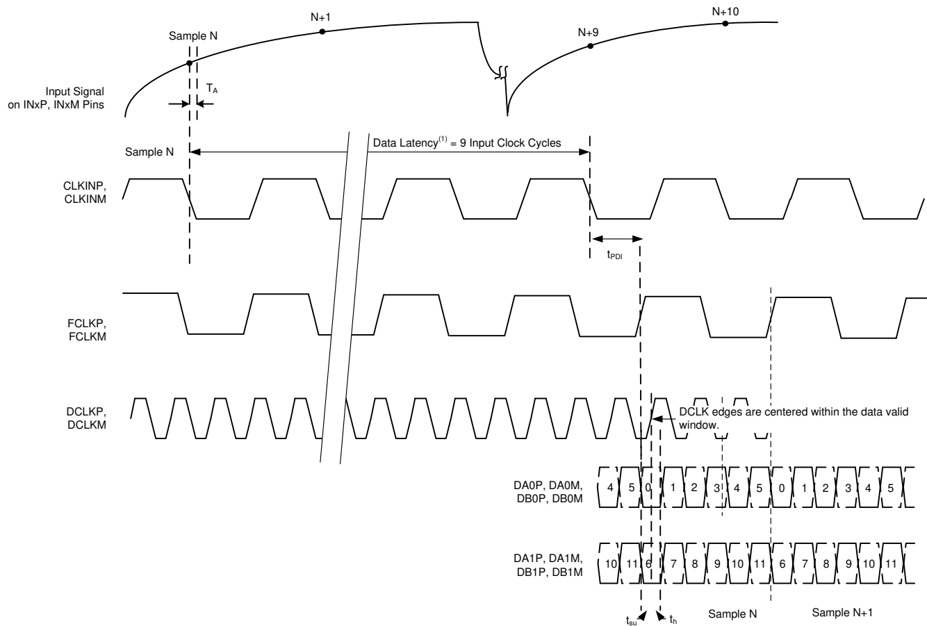
7-3. Setup and Hold Time
