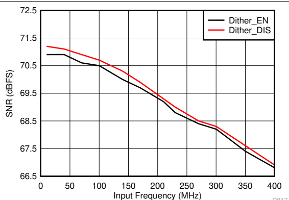
FIG 6-17. Signal-to-Noise Ratio vs Input Frequency
