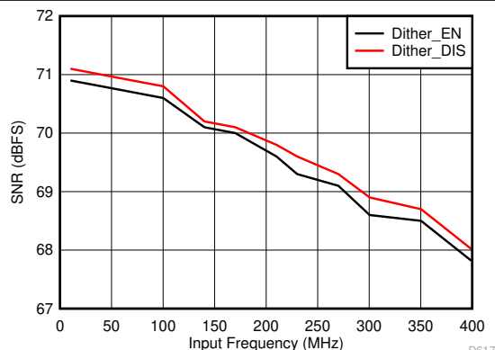
FIG 6-47. Signal-to-Noise Ratio vs Input Frequency
