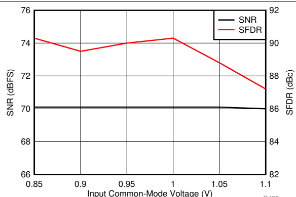
Figure 6-82. Performance vs Input Common-Mode Voltage (170 MHz)
