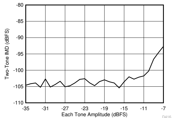
FIG 6-76. Intermodulation Distortion vs Input Amplitude (185 MHz and 190 MHz)
