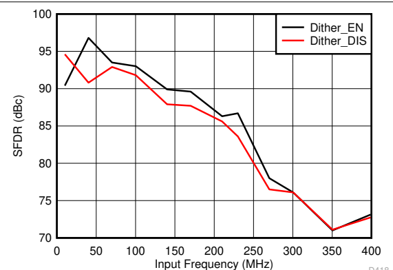
FIG 6-78. Spurious-Free Dynamic Range vs Input Frequency
