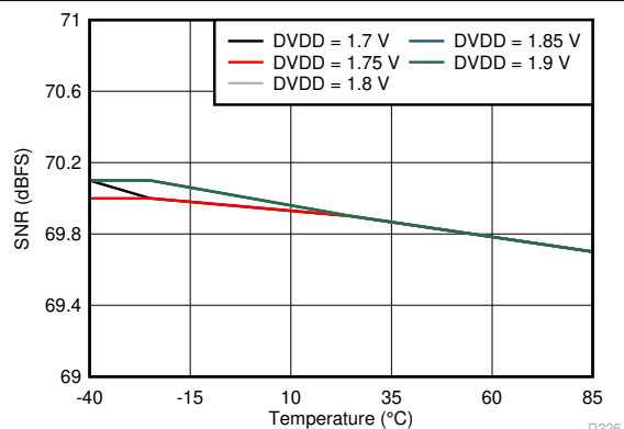
FIG 6-116. Signal-to-Noise Ratio vs DVDD Supply and Temperature (170 MHz)
