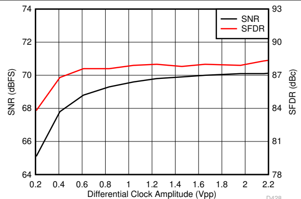
FIG 6-88. Performance vs Differential Clock Amplitude (150 MHz)
