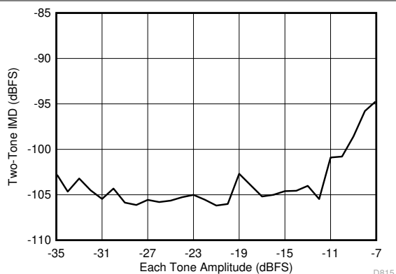
FIG 6-15. Intermodulation Distortion vs Input Amplitude (46 MHz and 50 MHz)
