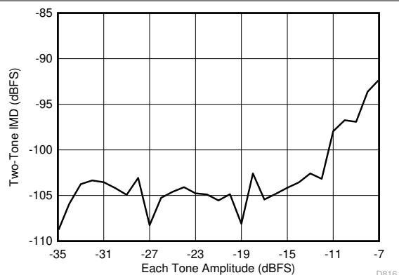
FIG 6-16. Intermodulation Distortion vs Input Amplitude (185 MHz and 190 MHz)
