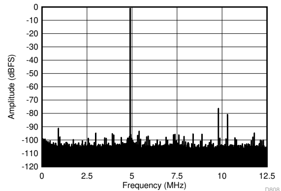
FIG 6-8. FFT for 270-MHz Input Signal (Dither Off)
