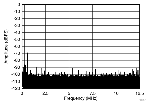
FIG 6-8. FFT for 270-MHz Input Signal (Dither Off)
