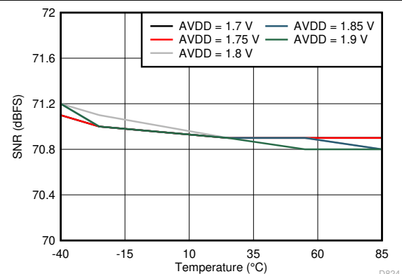
FIG 6-24. Signal-to-Noise Ratio vs AV_{DD} Supply and Temperature (30 MHz)
