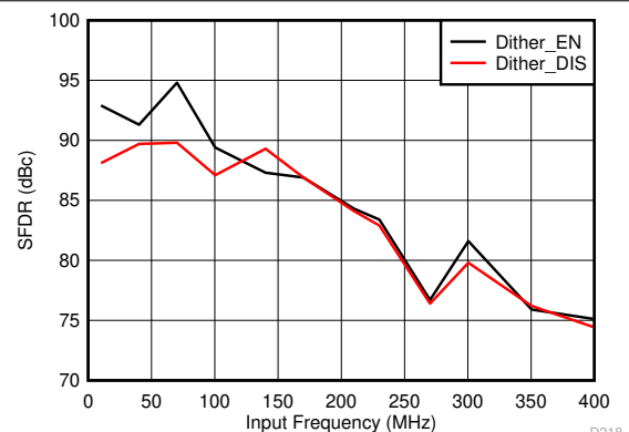
FIG 6-108. Spurious-Free Dynamic Range vs Input Frequency
