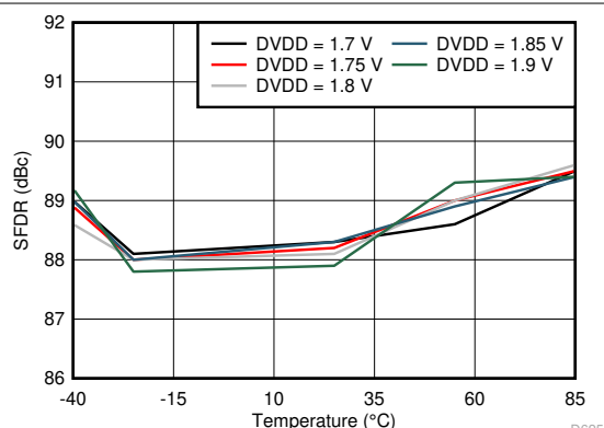
FIG 6-55. Spurious-Free Dynamic Range vs DVDD Supply and Temperature (30 MHz)
