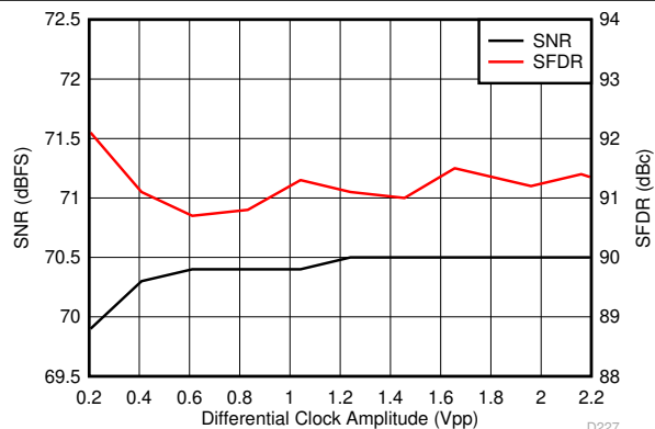
FIG 6-117. Performance vs Differential Clock Amplitude (40 MHz)
