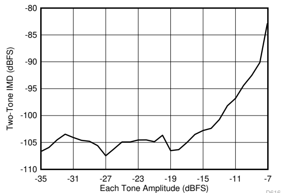
FIG 6-46. Intermodulation Distortion vs Input Amplitude (185 MHz and 190 MHz)
