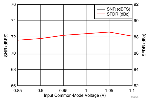
FIG 6-112. Performance vs Input Common-Mode Voltage (170 MHz)
