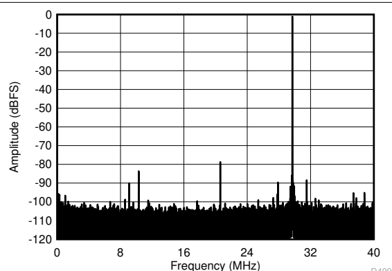
FIG 6-67. FFT for 270-MHz Input Signal (Dither On)
