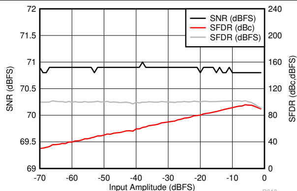
FIG 6-49. Performance vs Input Amplitude (30 MHz)
