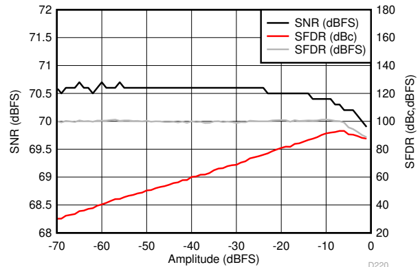
FIG 6-110. Performance vs Input Amplitude (170 MHz)
