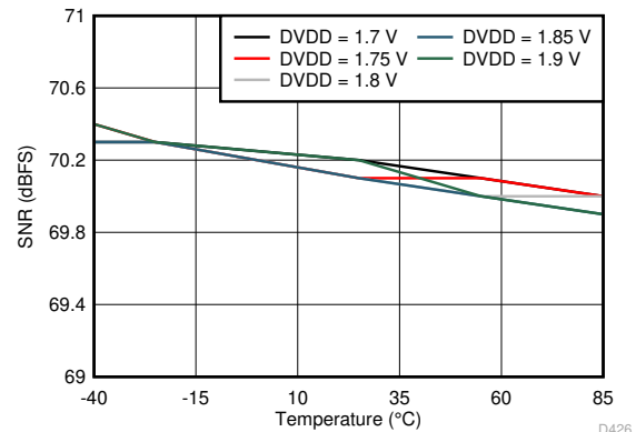
FIG 6-86. Signal-to-Noise Ratio vs DVDD Supply and Temperature (170 MHz)
