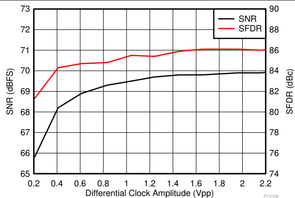
FIG 6-118. Performance vs Differential Clock Amplitude (150 MHz)
