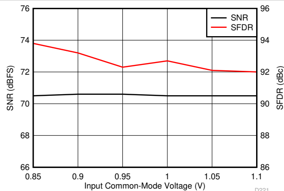
FIG 6-111. Performance vs Input Common-Mode Voltage (30 MHz)
