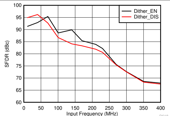
FIG 6-48. Spurious-Free Dynamic Range vs Input Frequency
