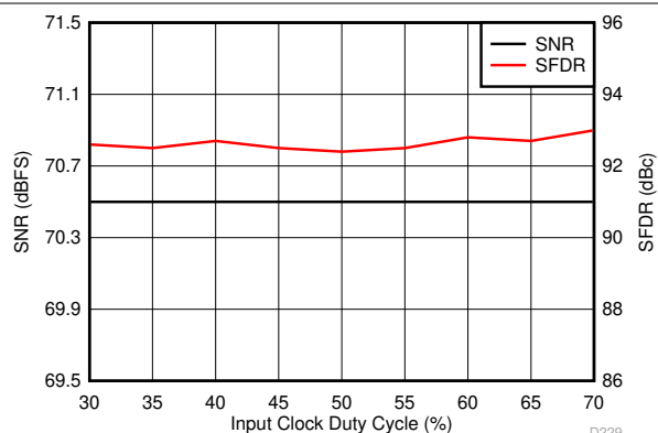
FIG 6-119. Performance vs Clock Duty Cycle (30 MHz)
