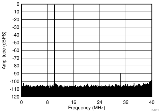
FIG 6-61. FFT for 10-MHz Input Signal (Dither On)
