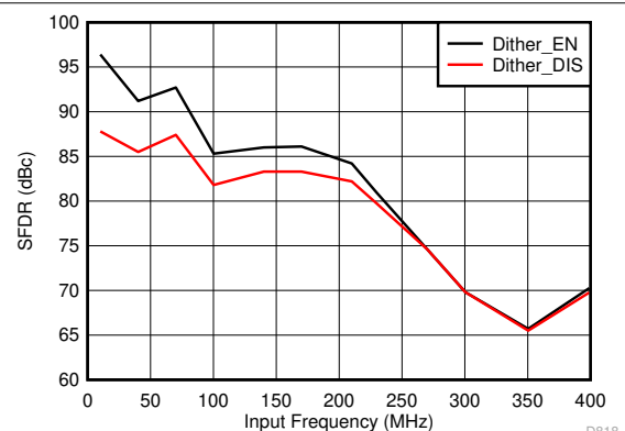
FIG 6-18. Spurious-Free Dynamic Range vs Input Frequency
