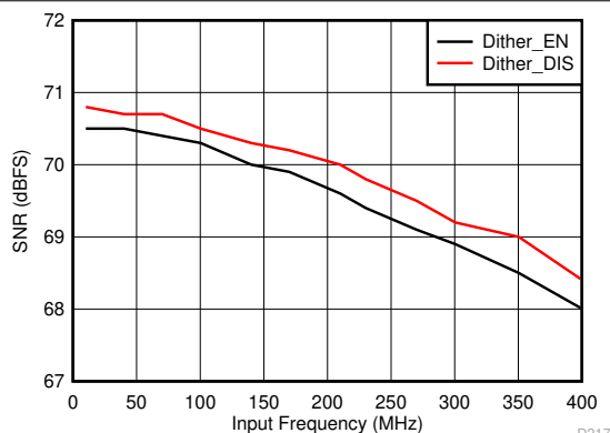
FIG 6-107. Signal-to-Noise Ratio vs Input Frequency
