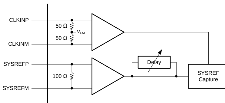
Figure 89. SYSREF Internal Circuit Diagram
