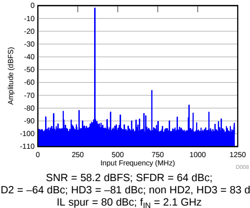
Figure 10. FFT for 2100-MHz Input Signal ( f_s = 2457.6 MSPS)
