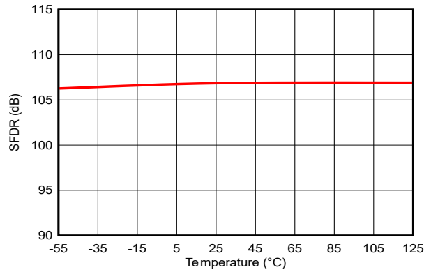
図 5-22. Spurious-Free Dynamic Range vs Temperature
