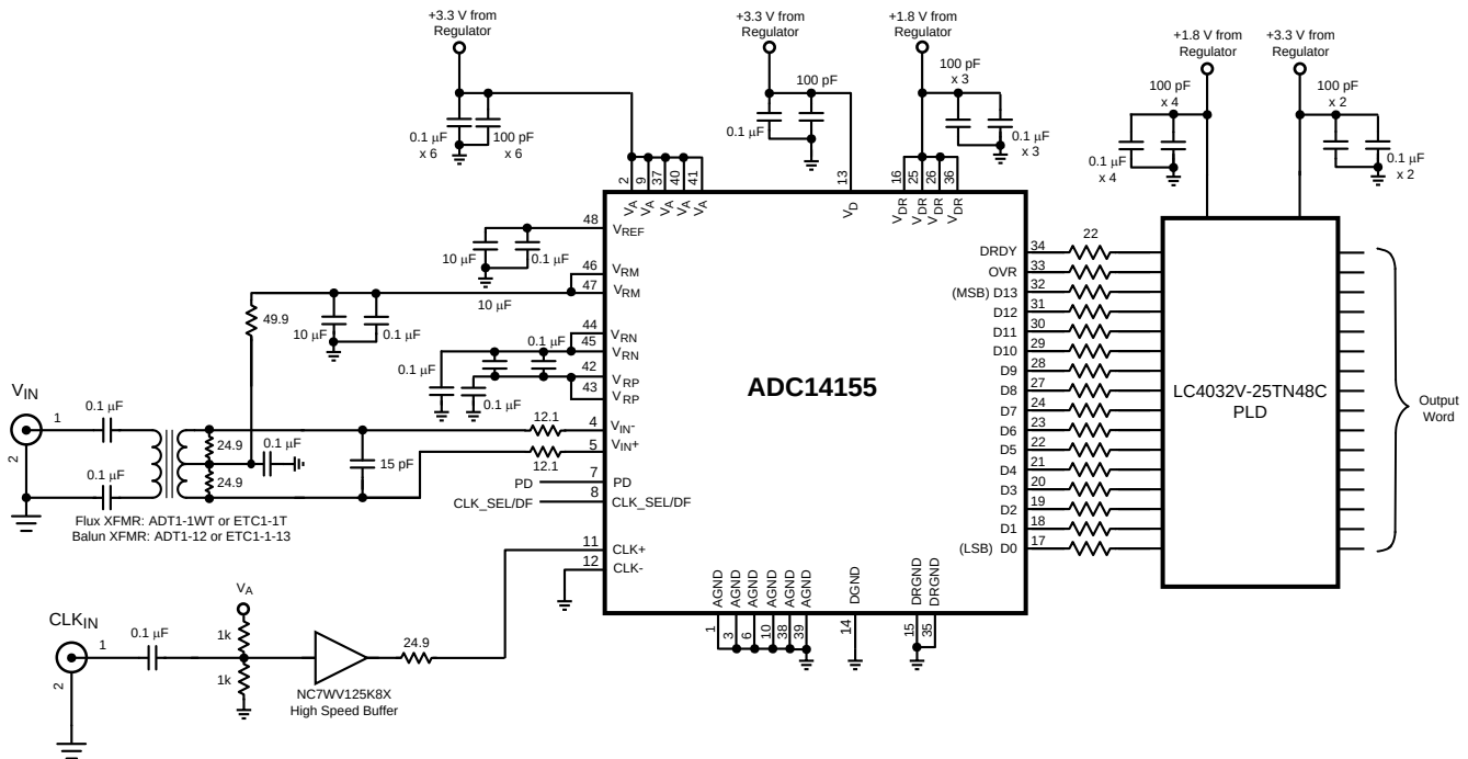
Figure 24. Application Circuit Using Transformer Drive Circuit
