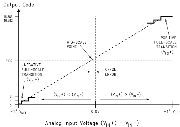
Figure 2. Transfer Characteristic
