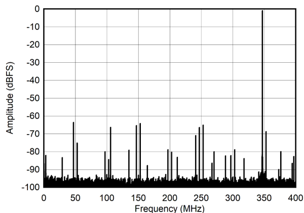
图 5-14. Single Tone FFT at 347 MHz and -1dBFS
