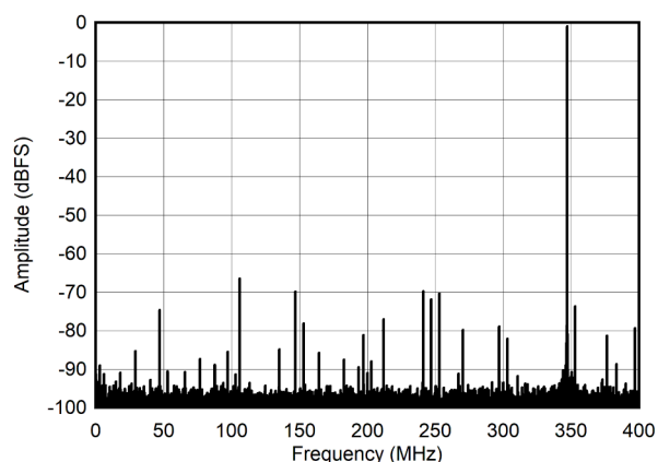
图 5-15. Single Tone FFT at 347 MHz and -1dBFS
