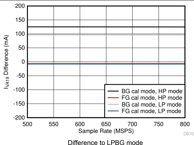
Figure 5-112. Single Channel, I_{VA19} vs F_S over Modes
