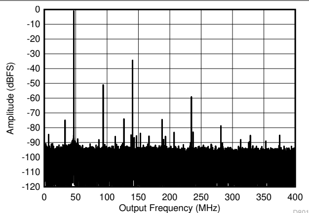
图 5-13. Single Tone FFT at 3247 MHz and -1dBFS
