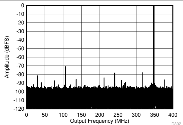
図 5-8. Single Tone FFT at 2097 MHz and -1dBFS
