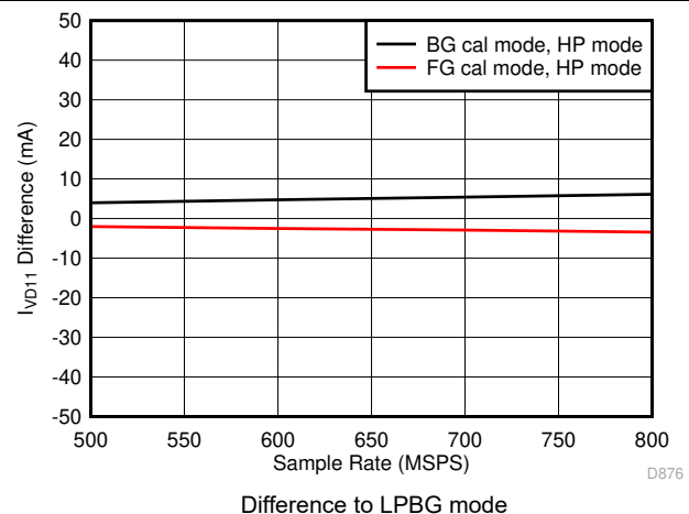
Figure 5-114. Single Channel, I_{VD11} vs F_S over Modes
