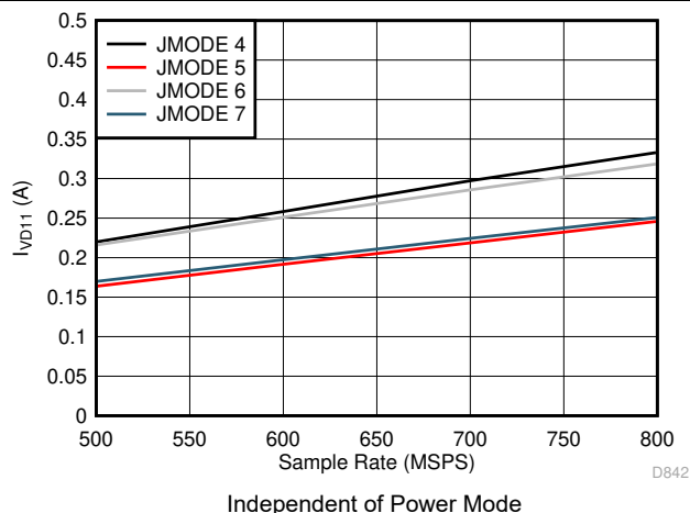
図 5-81. Quad Channel, I_{VD11} vs F_S for JMODES 4 - 7
