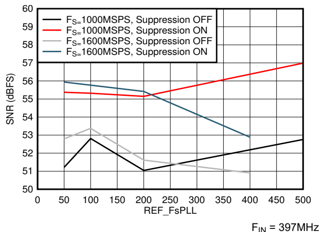
Figure 6-38. SNR vs F_{REF} and Suppression
