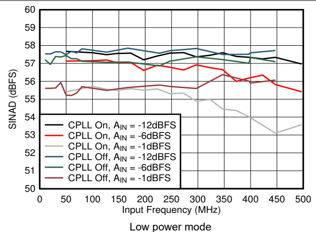
図 6-56. SINAD vs A_{IN} and C-PLL
