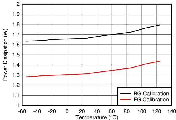
Figure 6-121. Quad Channel, Power Dissipation vs Temperature
