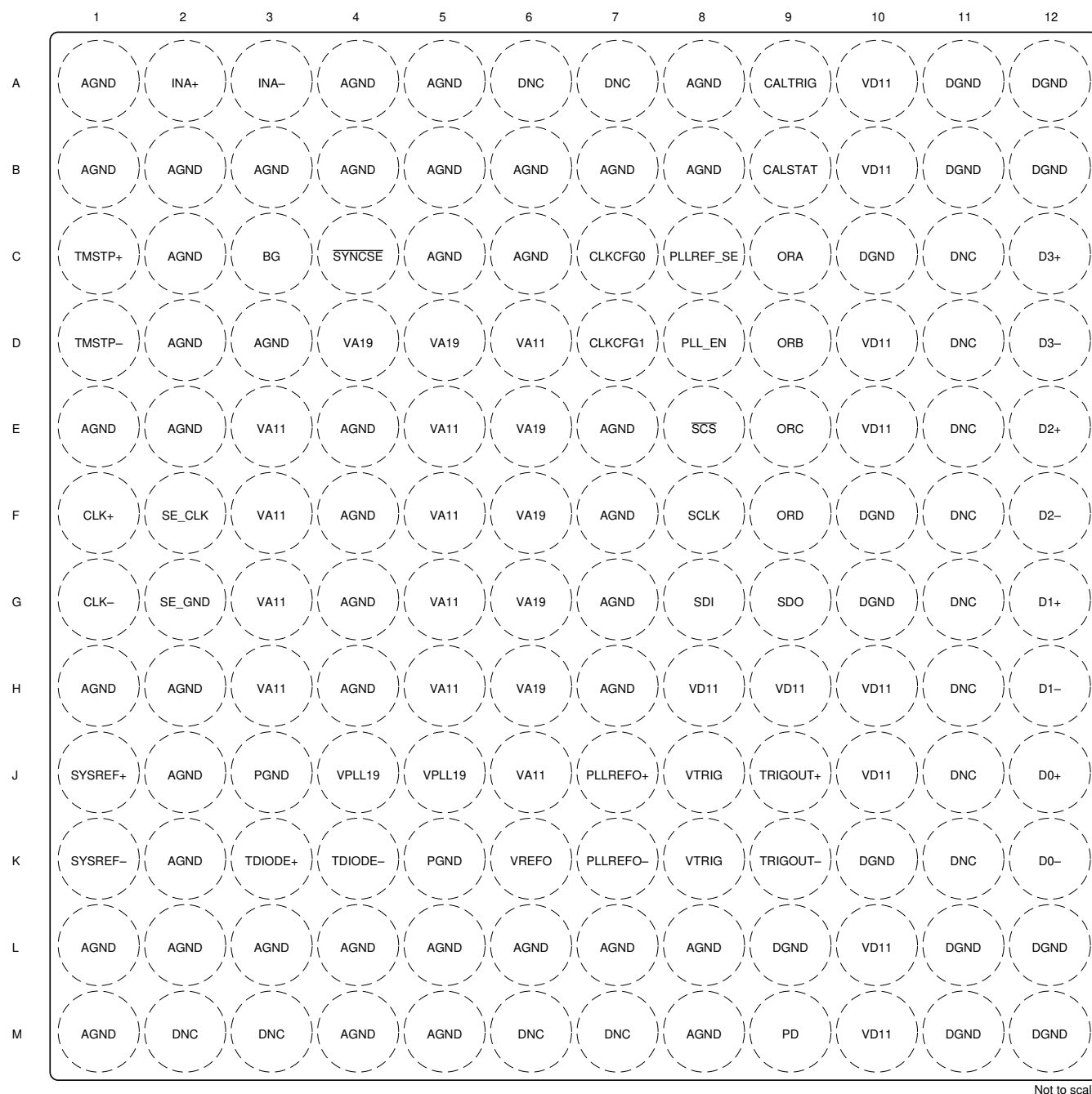
図 5-3. Single Channel AAV Package, 144-Ball Flip Chip BGA (Top View)
