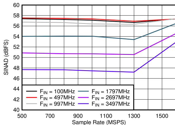
Figure 6-25. SINAD vs Sample Rate
