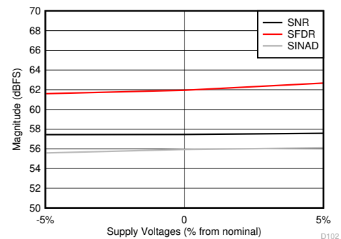
Figure 6-62. SNR, SFDR and SINAD vs Supply Voltages
