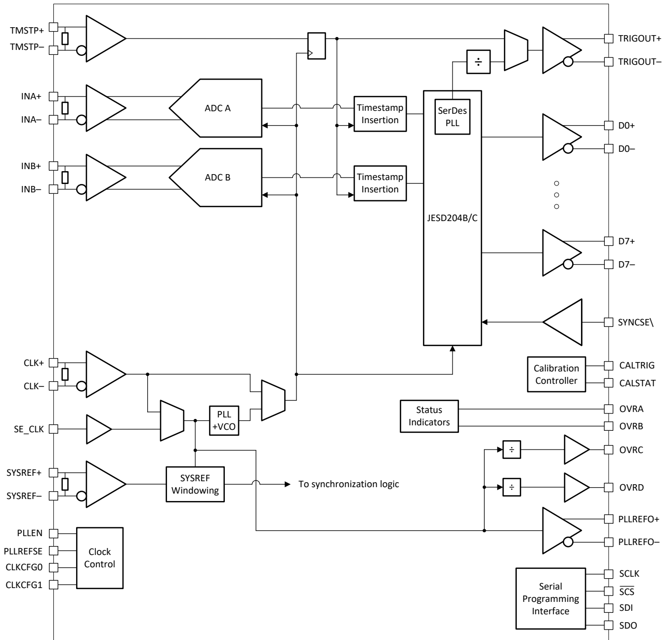
図 7-2. Dual Channel Functional Block Diagram
