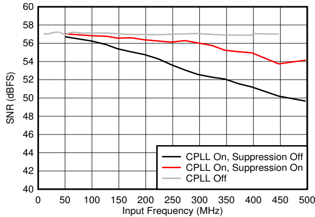
図 6-45. SNR vs F_{IN} and C-PLL modes
