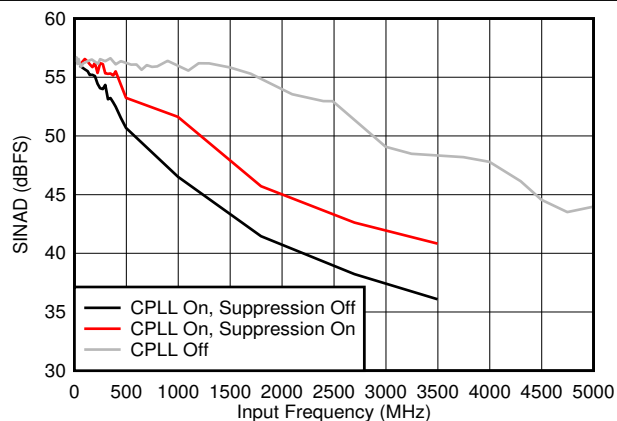
図 5-42. SINAD vs F_{IN} and C-PLL modes
