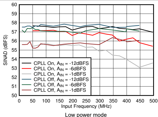
5-56. SINAD vs A_{IN} and C-PLL
