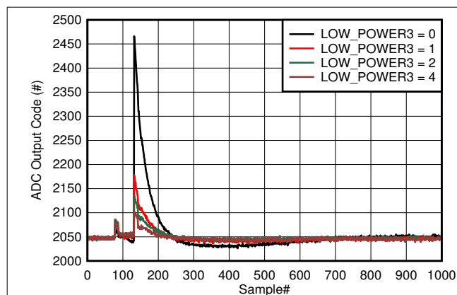
図 6-12. Background Calibration Core Transition In Low Power Mode
