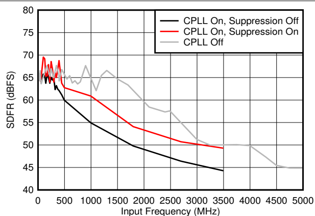
図 5-40. SFDR vs F_{IN} and C-PLL modes
