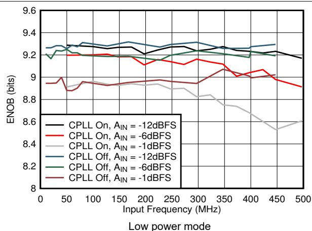
5-57. ENOB vs A_{IN} and C-PLL
