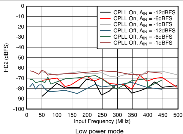
5-58. HD2 vs A_{IN} and C-PLL
