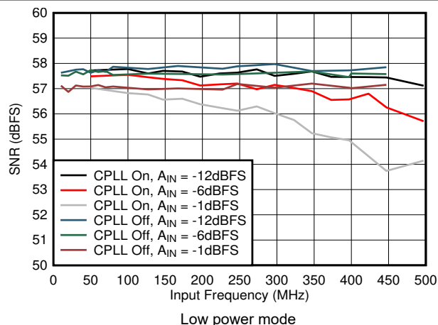
5-55. SNR vs A_{IN} and C-PLL
