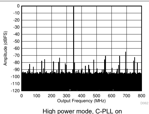
Figure 5-5. Single Tone FFT at 347MHz and -1dBFS
