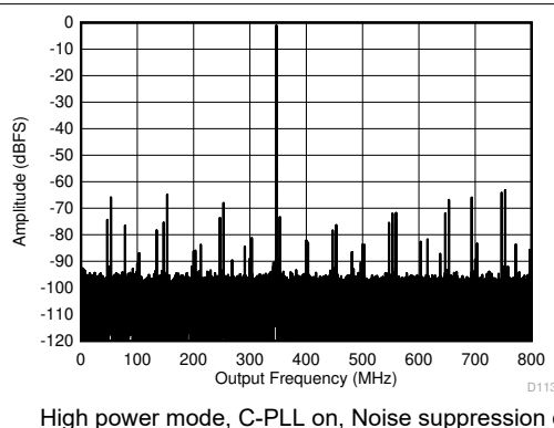
Figure 5-6. Single Tone FFT at 347MHz and -1dBFS
