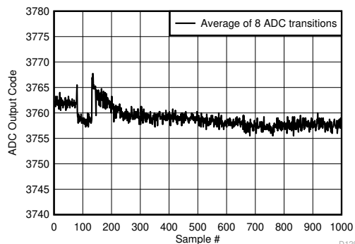
Figure 5-125. Background Calibration Core Transition (offset voltage)
