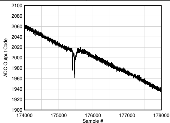
Figure 5-125. Background Calibration Core Transition (offset voltage)
