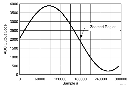
Figure 5-126. Background Calibration Core Transition (AC Signal)
