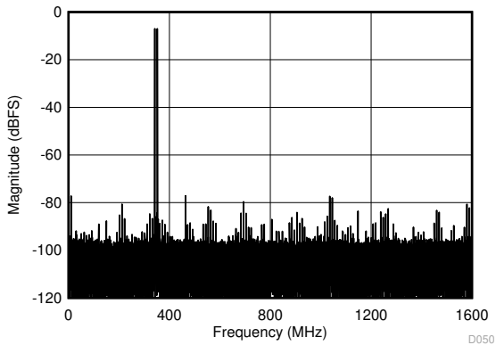
6-44. Single-Tone FFT at f_{\text{IN}} = 8197\text{ MHz} , A_{\text{IN}} = -1\text{ dBFS}
