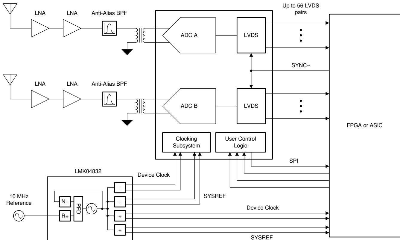
図 8-1. Typical Configuration for Wideband RF Sampling
