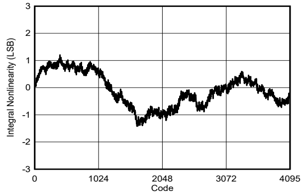
FIG 5-209. INL vs Code
