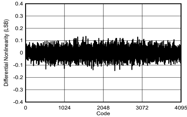
FIG 5-208. DNL vs Code
