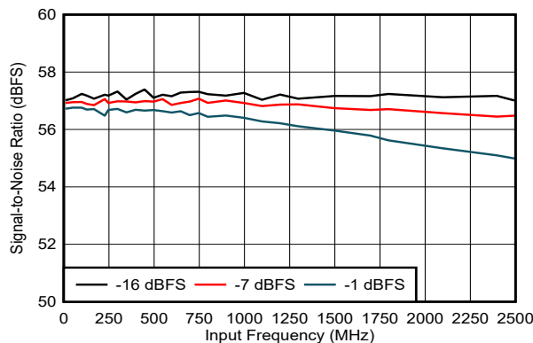
FIG 5-210. SNR vs Input Frequency
