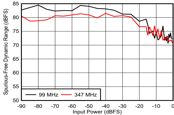
FIG 5-28. SFDR vs Input Power
