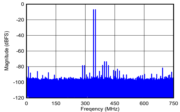
DES_EN = 0, f_S = 1500\text{MHz} , FG calibration, f_1 = 342\text{MHz} , f_2 = 352\text{MHz} , A_{IN} = -7\text{dBFS} per tone, SFDR = -74\text{dBFS} , IMD3 = -92\text{dBFS} , IMD2 = -81\text{dBFS}
