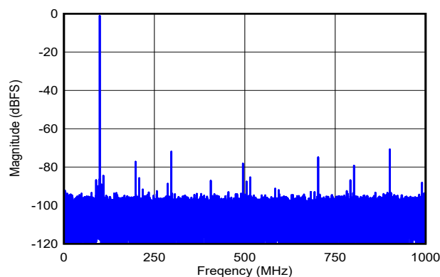
5-192. Single-Tone FFT at f_{IN} = 99\text{MHz} , A_{IN} = -1\text{dBFS}
