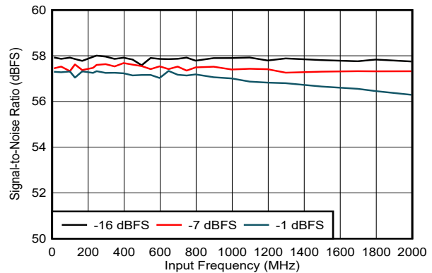
5-71. SNR vs Input Frequency
