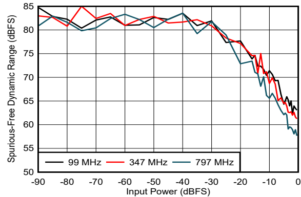
FIG 5-29. SFDR vs Input Power
