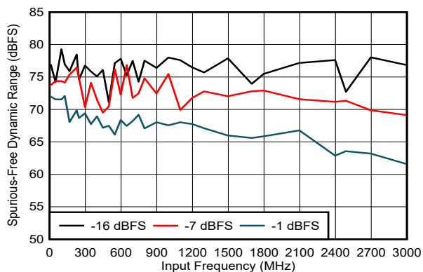
5-105. SFDR vs Input Frequency
