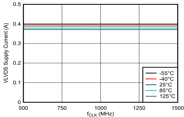
Figure 5-176. VLVD Supply Current vs Clock Rate
