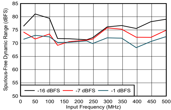
5-16. SFDR vs Input Frequency
