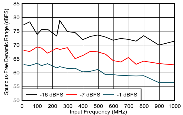
5-17. SFDR vs Input Frequency
