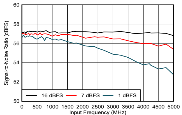
FIG 5-211. SNR vs Input Frequency
