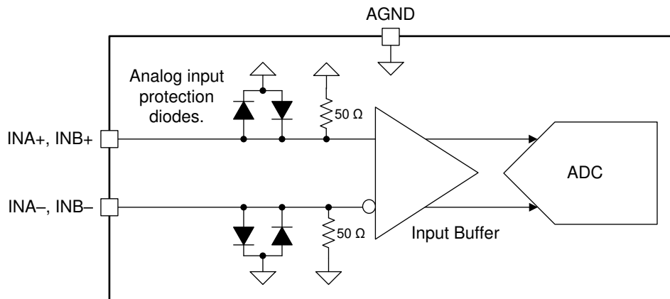
図 6-1. ADC12Dx500 Analog Input Internal Termination
