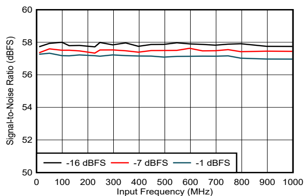
5-11. SNR vs Input Frequency
