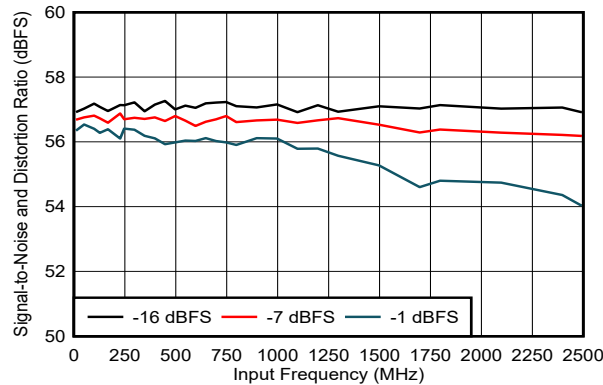
5-212. SINAD vs Input Frequency
