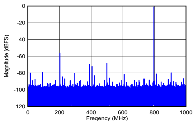
FIG 5-87. Single-Tone FFT at f_{IN} = 797\text{MHz} , A_{IN} = -1\text{dBFS}
