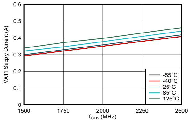
FIG 5-288. VA11 Supply Current vs Clock Rate
