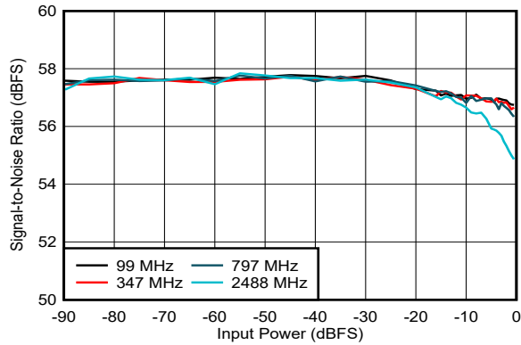
5-230. SNR vs Input Power
