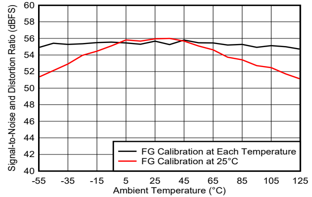
5-55. SINAD vs Temperature and Calibration Mode
