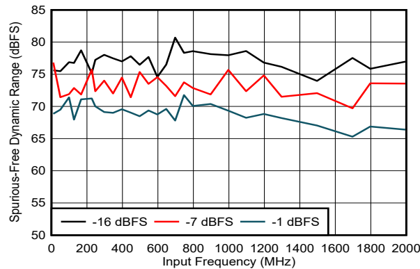
5-186. SFDR vs Input Frequency
