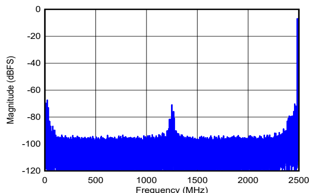
DES_EN = 1, f_S = 5000\text{MHz} , FG calibration, f_1 = 2483\text{MHz} , f_2 = 2493\text{MHz} , A_{IN} = -7\text{dBFS} per tone, SFDR = -67dBFS, IMD3 = -74dBFS, IMD2 = -73dBFS
