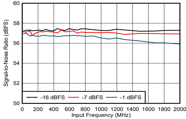
5-180. SNR vs Input Frequency
