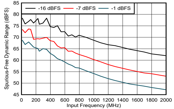
FIG 5-77. SFDR vs Input Frequency
