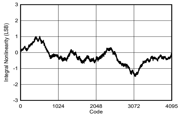
5-49. INL vs Code
