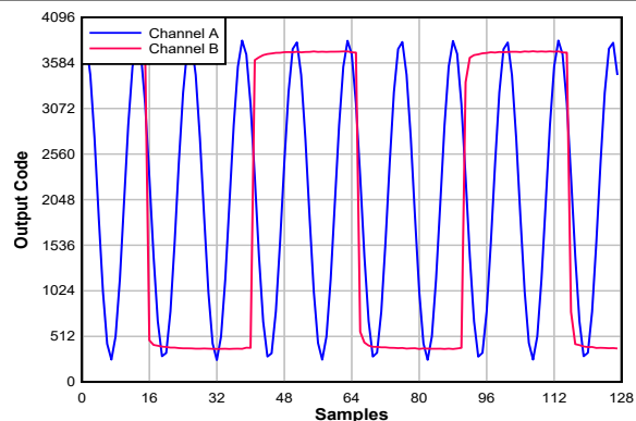
図 7-7. 200MHz, Sine-Wave (Channel A) and 50MHz, Square-Wave (Channel B) Time Domain for 2.5GSPS, Dual-Channel Oscilloscope
