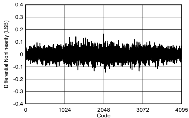
5-48. DNL vs Code
