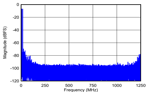
DES_EN = 0, f_S = 2500\text{MHz} , FG calibration, f_1 = 2483\text{MHz} , f_2 = 2493\text{MHz} , A_{IN} = -7\text{dBFS} per tone, SFDR = -70dBFS, IMD3 = -76dBFS, IMD2 = -74dBFS
