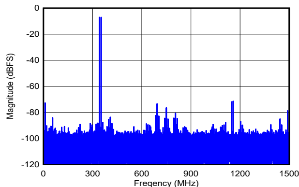
DES_EN = 1, f_S = 3000\text{MHz} , FG calibration, f_1 = 342\text{MHz} , f_2 = 352\text{MHz} , A_{IN} = -7\text{dBFS} per tone, SFDR = -71dBFS, IMD3 = -88dBFS, IMD2 = -73dBFS
