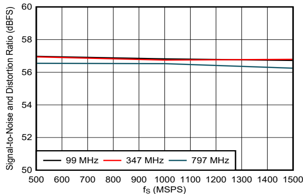
5-110. SNR vs Sampling Rate
