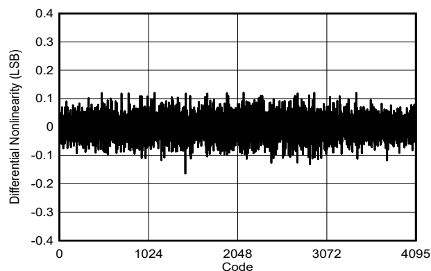
5-94. DNL vs Code
