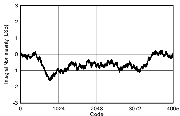
5-95. INL vs Code
