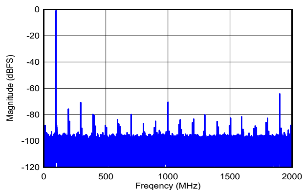
DES_EN = 1, f_S = 4000\text{MHz} , FG calibration, SNR = 57.3dBFS, SFDR = 64.4dBFS, ENOB = 9.0 bits
