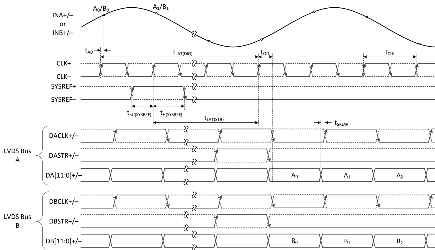
図 5-1. Dual-Channel, 2-Bus Mode Timing (LDEMUX = 0, DES_EN = 0, LALIGNED = 0 or 1)
