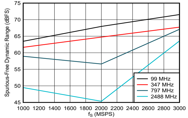
FIG 5-117. SFDR vs Sampling Rate
