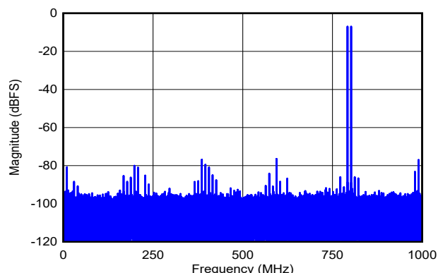
DES_EN = 0, f_S = 2000\text{MHz} , FG calibration, f_1 = 792\text{MHz} , f_2 = 802\text{MHz} , A_{IN} = -7\text{dBFS} per tone, SFDR = -76dBFS, IMD3 = -88dBFS, IMD2 = -81dBFS
