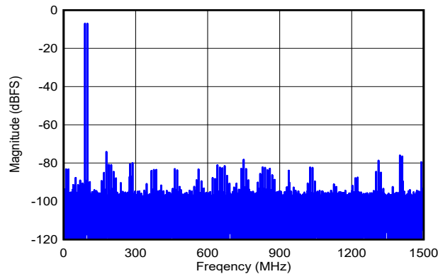
DES_EN = 1, f_S = 3000\text{MHz} , FG calibration, f_1 = 89\text{MHz} , f_2 = 99\text{MHz} , A_{IN} = -7\text{dBFS} per tone, SFDR = -74dBFS, IMD3 = -90dBFS, IMD2 = -82dBFS
