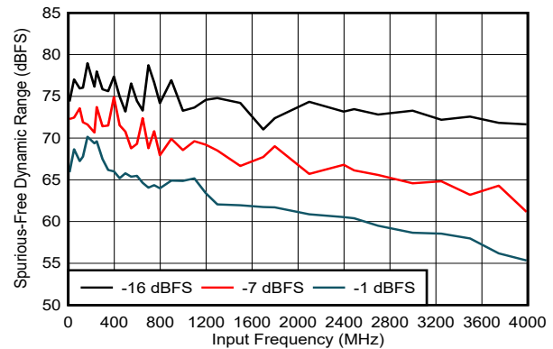
5-187. SFDR vs Input Frequency
