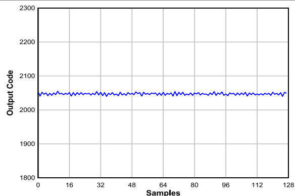
図 7-6. Idle-Channel Noise (No Input) for 5GSPS, Single-Channel Oscilloscope
