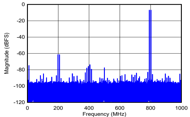
DES_EN = 1, f_S = 2000\text{MHz} , FG calibration, f_1 = 792\text{MHz} , f_2 = 802\text{MHz} , A_{IN} = -7\text{dBFS} per tone, SFDR = -62dBFS, IMD3 = -84dBFS, IMD2 = -74dBFS
