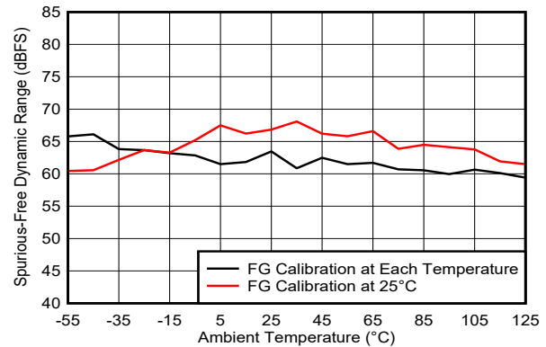
5-57. ENOB vs Temperature and Calibration Mode
