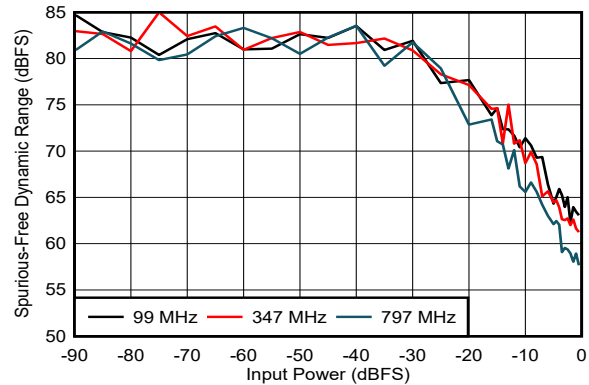
Figure 5-29. SFDR vs Input Power
