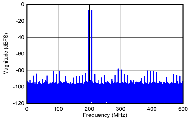
DES_EN = 0, f_S = 1000\text{MHz} , FG calibration, f_1 = 792\text{MHz} , f_2 = 802\text{MHz} , A_{IN} = -7\text{dBFS} per tone, SFDR = -78dBFS, IMD3 = -84dBFS, IMD2 = -85dBFS
