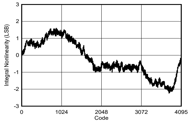
5-265. INL vs Code
