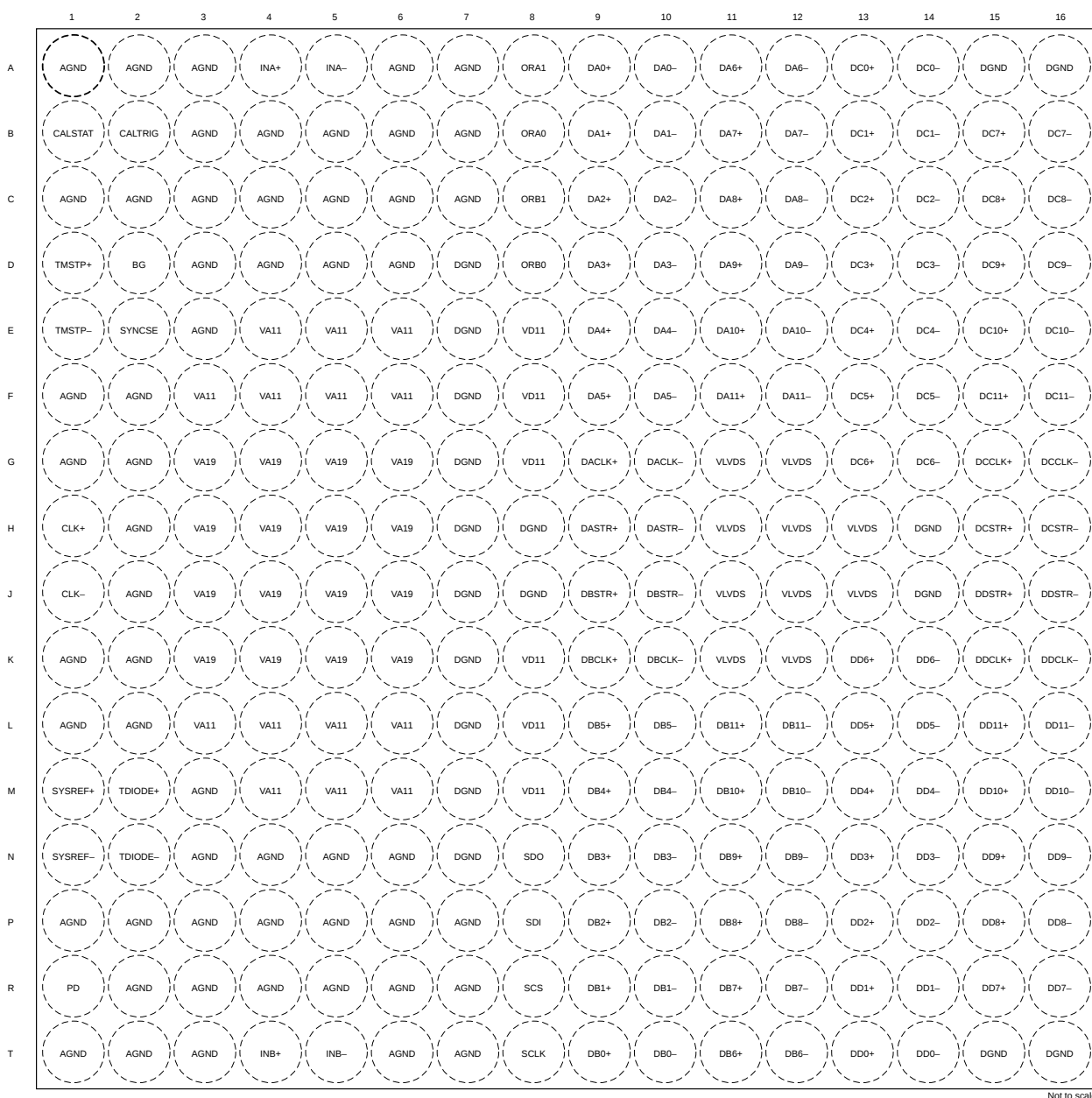
4-1. ACF Package, 256-Ball Flip Chip BGA (Top View)
