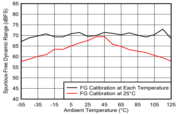
FIG 5-158. SFDR vs Temperature and Calibration Mode
