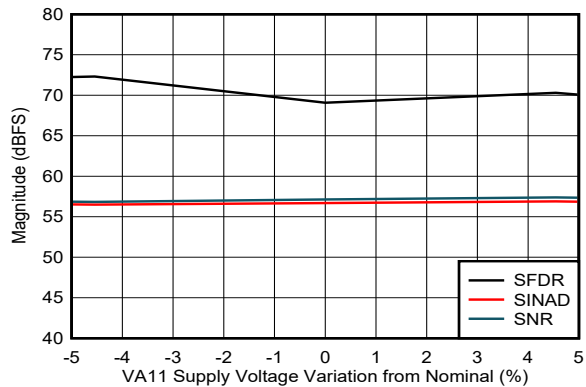
Figure 5-164. Performance vs VA11 Supply Voltage
