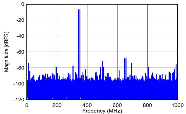
DES_EN = 1, f_S = 2000\text{MHz} , FG calibration, f_1 = 342\text{MHz} , f_2 = 352\text{MHz} , A_{IN} = -7\text{dBFS} per tone, SFDR = -68dBFS, IMD3 = -89dBFS, IMD2 = -74dBFS
