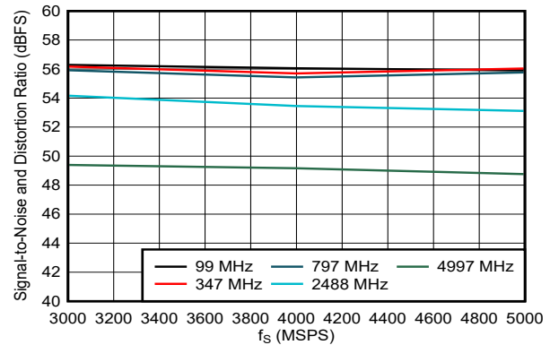
5-225. SINAD vs Sampling Rate
