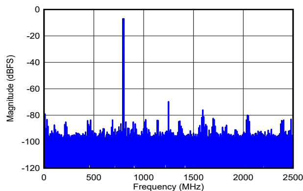
DES_EN = 1, f_S = 5000\text{MHz} , FG calibration, f_1 = 792\text{MHz} , f_2 = 802\text{MHz} , A_{IN} = -7\text{dBFS} per tone, SFDR = -76dBFS, IMD3 = -93dBFS, IMD2 = -77dBFS
