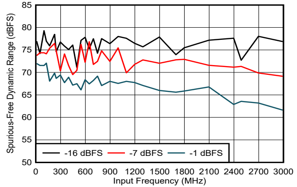
5-105. SFDR vs Input Frequency
