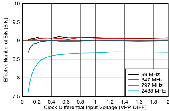
Figure 5-242. ENOB vs Clock Amplitude
