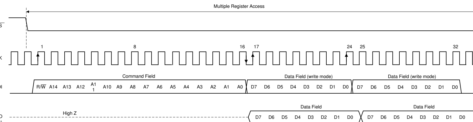
図 6-6. Serial Interface Protocol: Streaming Read/Write Operation
