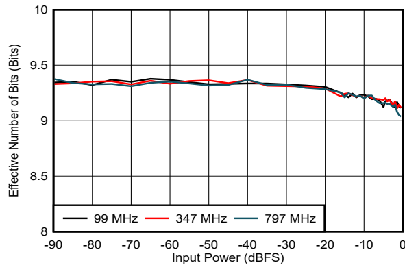
5-122. ENOB vs Input Power
