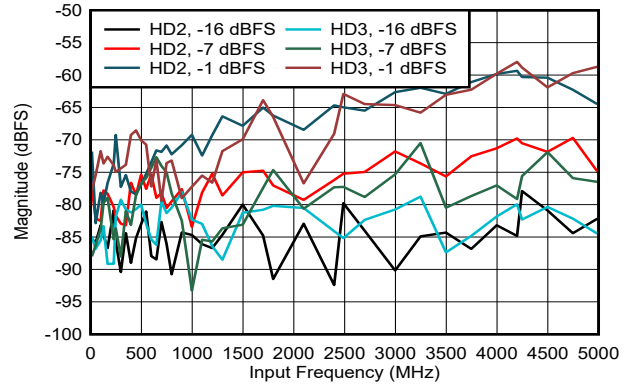
図 5-219. HD2 and HD3 vs Input Frequency
