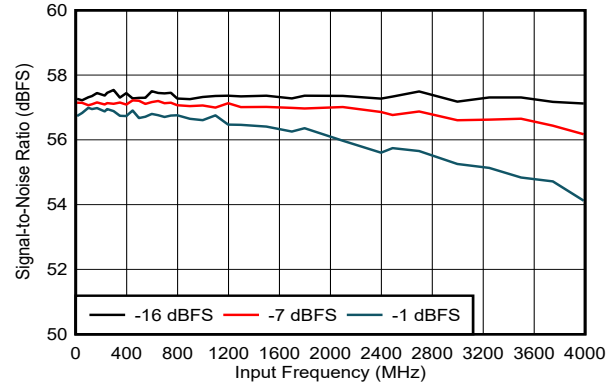
5-181. SNR vs Input Frequency
