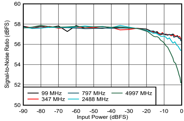
5-231. SNR vs Input Power
