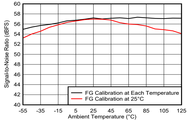
FIG 5-153. SNR vs Temperature and Calibration Mode
