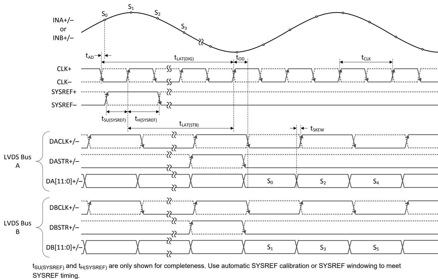
图 5-5. Single-Channel, 2-Bus, Aligned-Mode Timing (LDEMUX = 0, DES_EN = 1, LALIGNED = 1)
