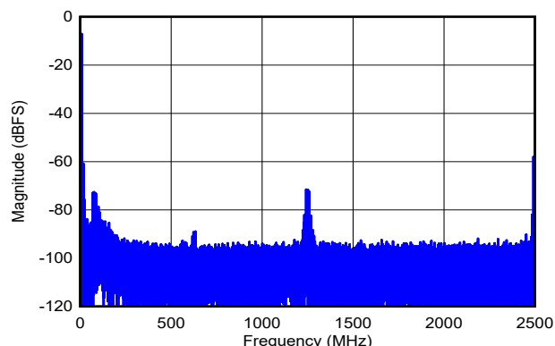
DES_EN = 1, f_S = 5000\text{MHz} , FG calibration, f_1 = 4992\text{MHz} , f_2 = 5002\text{MHz} , A_{IN} = -7\text{dBFS} per tone, SFDR = -58dBFS, IMD3 = -61dBFS, IMD2 = -78dBFS
