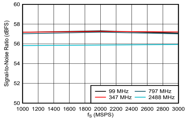
5-111. SNR vs Sampling Rate
