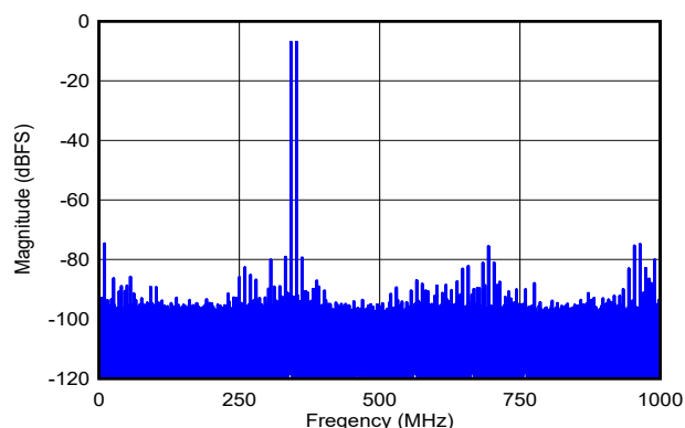
DES_EN = 0, f_S = 2000\text{MHz} , FG calibration, f_1 = 342\text{MHz} , f_2 = 352\text{MHz} , A_{IN} = -7\text{dBFS} per tone, SFDR = -75dBFS, IMD3 = -79dBFS, IMD2 = -75dBFS
