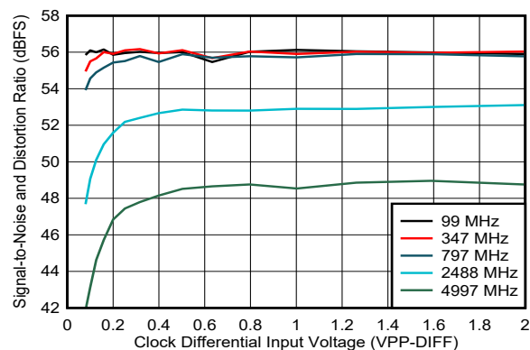
Figure 5-239. SNR vs Clock Amplitude
