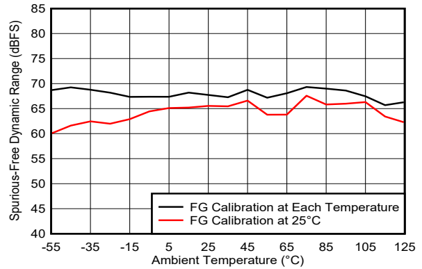
FIG 5-159. SFDR vs Temperature and Calibration Mode
