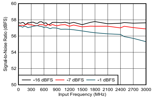
5-99. SNR vs Input Frequency
