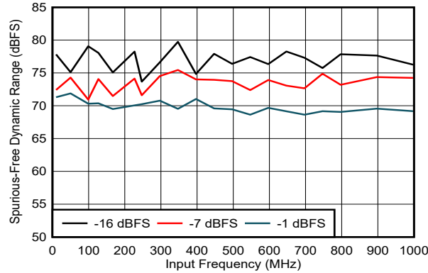
FIG 5-76. SFDR vs Input Frequency
