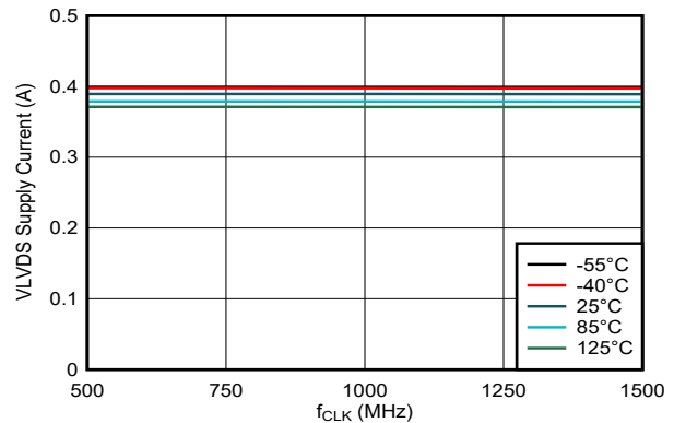
Figure 5-177. VLVDs Supply Current vs Clock Rate
