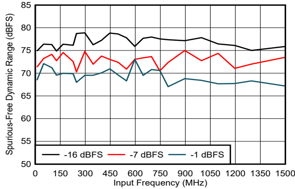
5-104. SFDR vs Input Frequency
