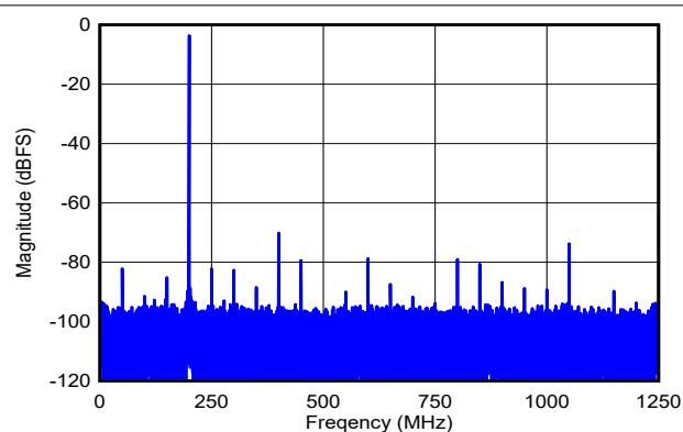
図 7-8. 200MHz, Sine-Wave (Channel A) Frequency Domain (FFT) for 2.5GSPS, Dual-Channel Oscilloscope
