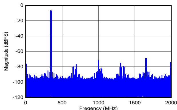
DES_EN = 1, f_S = 4000\text{MHz} , FG calibration, f_1 = 342\text{MHz} , f_2 = 352\text{MHz} , A_{IN} = -7\text{dBFS} per tone, SFDR = -69dBFS, IMD3 = -95dBFS, IMD2 = -77dBFS
