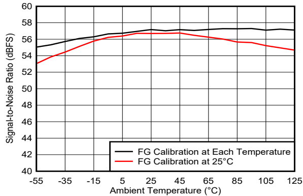
FIG 5-152. SNR vs Temperature and Calibration Mode
