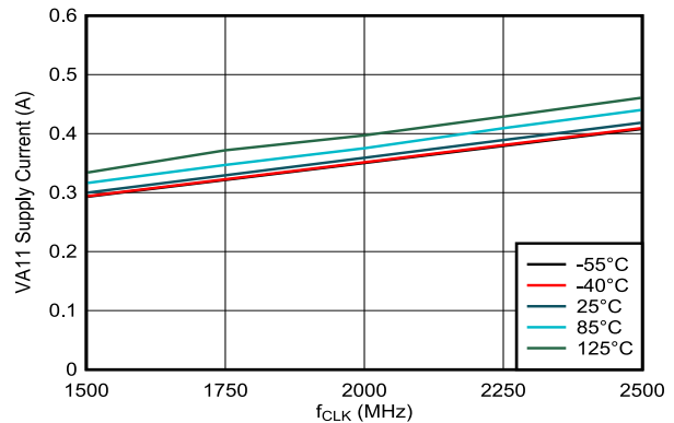
FIG 5-289. VA11 Supply Current vs Clock Rate
