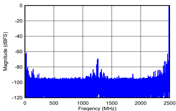
DES_EN = 1, f_S = 5000\text{MHz} , FG calibration, SNR = 55.7dBFS, SFDR = 61.5dBFS, ENOB = 8.5 bits
