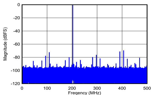
FIG 5-86. Single-Tone FFT at f_{IN} = 797\text{MHz} , A_{IN} = -1\text{dBFS}
