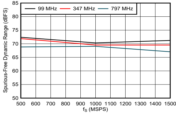
FIG 5-116. SFDR vs Sampling Rate
