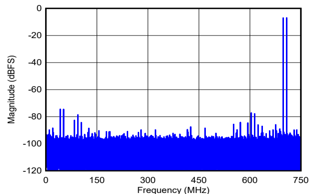
DES_EN = 0, f_S = 1500\text{MHz} , FG calibration, f_1 = 792\text{MHz} , f_2 = 802\text{MHz} , A_{IN} = -7\text{dBFS} per tone, SFDR = -74dBFS, IMD3 = -90dBFS, IMD2 = -82dBFS
