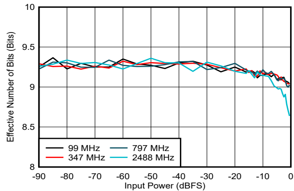
5-123. ENOB vs Input Power
