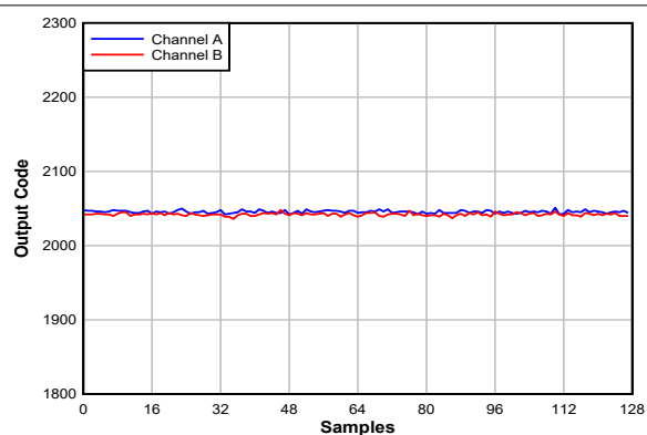
図 7-9. Idle-Channel Noise (No Input) for 2.5GSPS, Dual-Channel Oscilloscope
