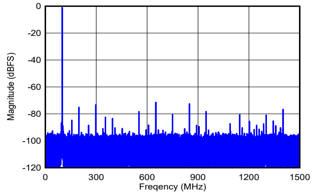
5-135. Single-Tone FFT at f_{IN} = 99\text{MHz} , A_{IN} = -1\text{dBFS}
