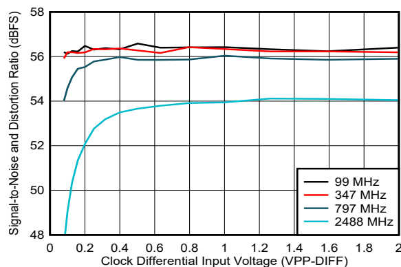
Figure 5-238. SNR vs Clock Amplitude
