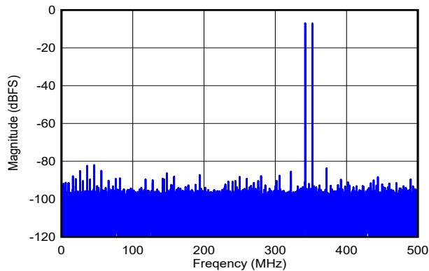
DES_EN = 0, f_S = 1000\text{MHz} , FG calibration, f_1 = 342\text{MHz} , f_2 = 352\text{MHz} , A_{IN} = -7\text{dBFS} per tone, SFDR = -82dBFS, IMD3 = -96dBFS, IMD2 = -89dBFS
