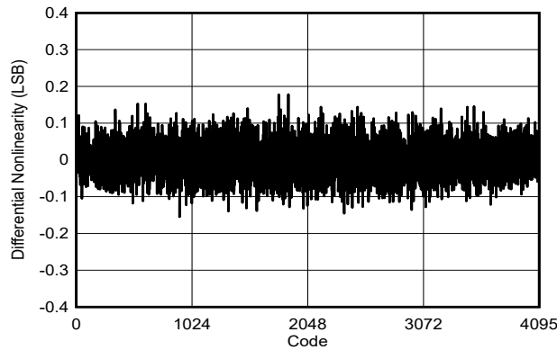
5-264. DNL vs Code
