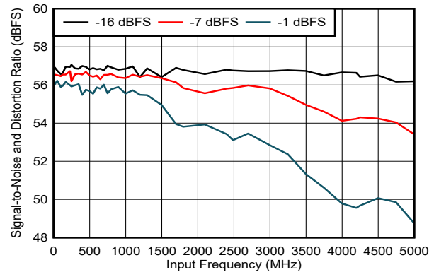
5-213. SINAD vs Input Frequency
