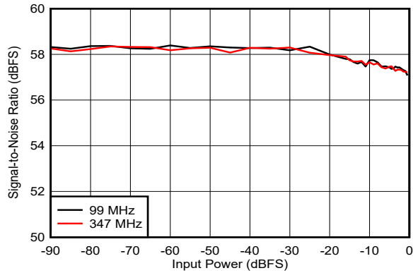
5-22. SNR vs Input Power
