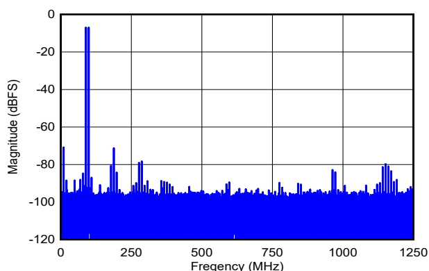
DES_EN = 0, f_S = 2500\text{MHz} , FG calibration, f_1 = 89\text{MHz} , f_2 = 99\text{MHz} , A_{IN} = -7\text{dBFS} per tone, SFDR = -71dBFS, IMD3 = -86dBFS, IMD2 = -71dBFS
