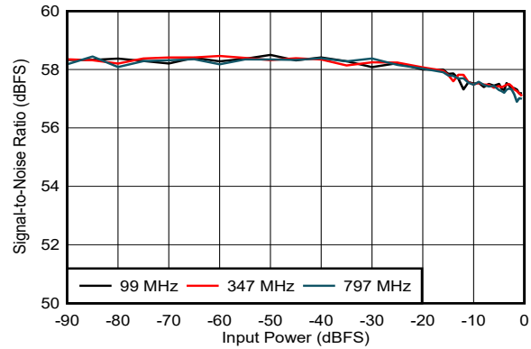
5-23. SNR vs Input Power
