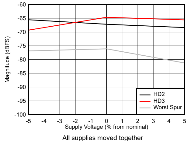
Figure 5-39. HD2, HD3 and worst non-HD vs Supply Voltage
