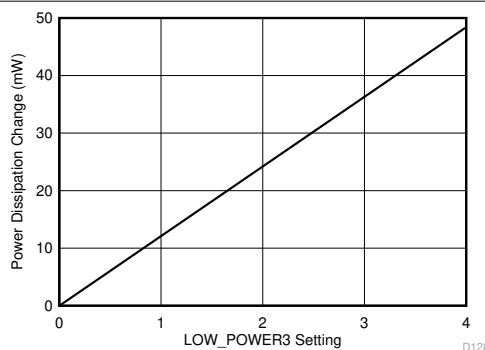
図 6-13. Power Dissipation Change vs LOW_POWER3 register setting
