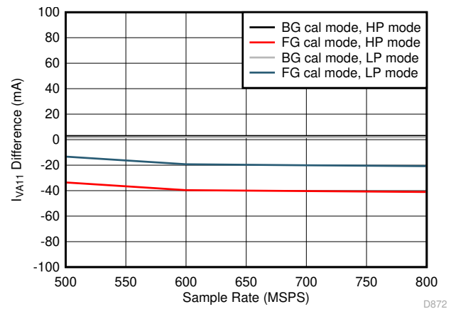
Figure 5-100. Dual Channel, I_{VA11} vs F_S over Modes
