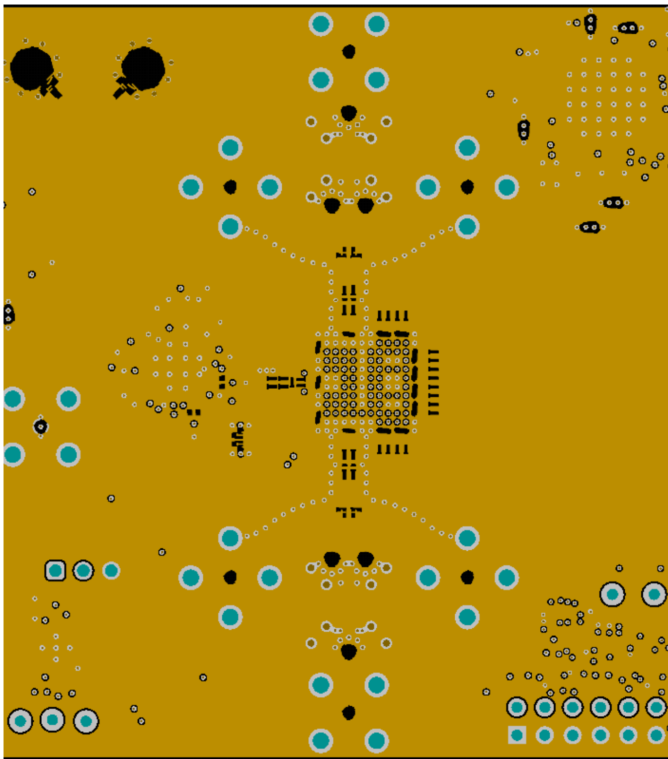
図 7-16. GND1 Cutouts to Optimize Impedance of Component Pads
