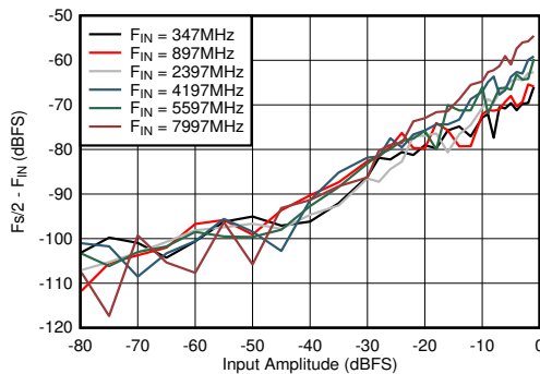
図 5-65. DES Mode: F_s/2 - F_{\text{IN}} vs Input Amplitude and Frequency
