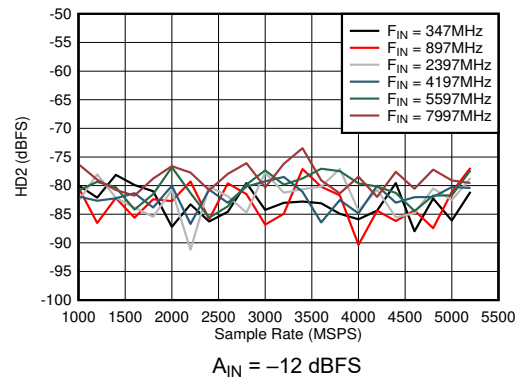
Figure 5-52. Dual Channel Mode: HD2 vs Sample Rate and Input Frequency
