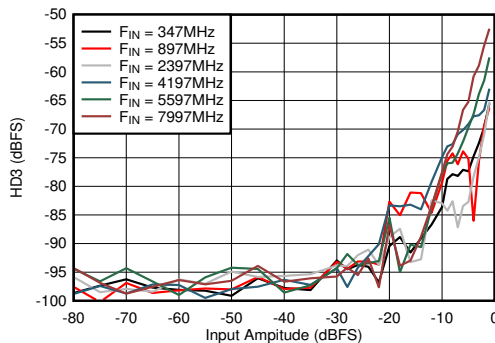
図 5-63. DES Mode: HD3 vs Input Amplitude and Frequency
