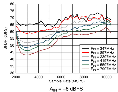
FIG 5-33. DES Mode: SFDR vs Sample Rate and Input Frequency
