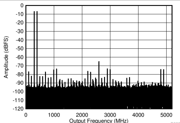
Figure 5-11. DES Mode: Two Tone FFT at 347 MHz
