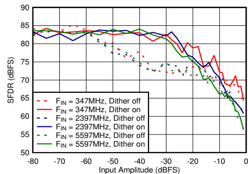
5-60. DES Mode: SFDR vs Input Amplitude and Dither
