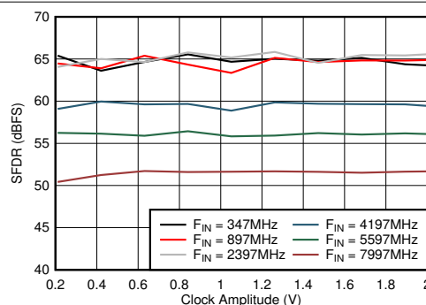
図 5-84. Dual Channel Mode: SFDR vs Clock Amplitude
