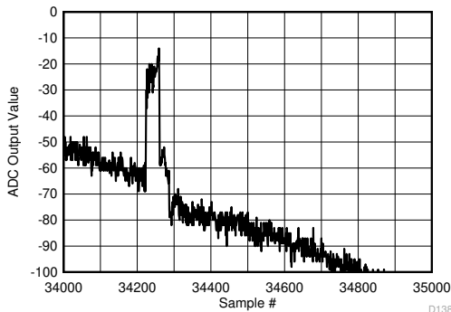
5-143. Background Calibration Core Transition (AC Signal - zoomed)
