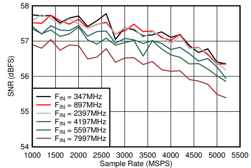
図 5-44. Dual Channel Mode: SNR vs Sample Rate and Input Frequency
