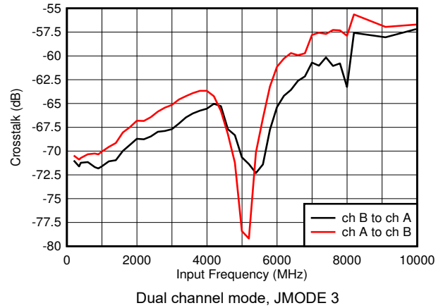
図 5-2. Crosstalk vs Input Frequency
