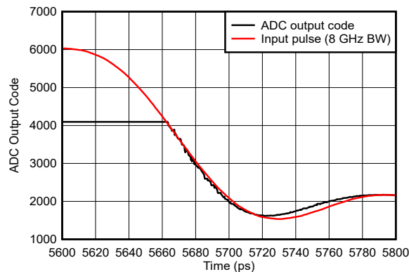
FIG 5-147. Pulse Overdrive Recovery Zoomed
