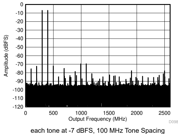
5-23. Dual Channel Mode: Two Tone FFT at 347 MHz
