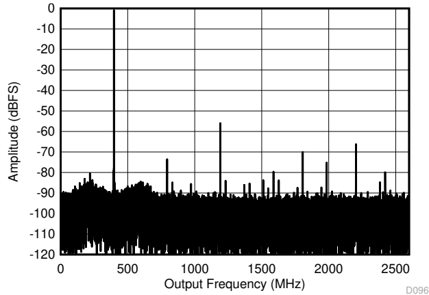
5-21. Dual Channel Mode: Single Tone FFT at 5597 MHz
