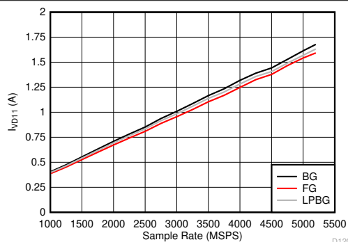
Figure 5-134. Dual Channel Mode: I_{VD11} vs Sample Rate
