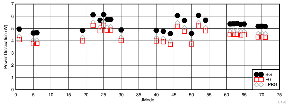
5-111. DES Mode: I_{VD11} vs JMODE at 10.4GSPS
