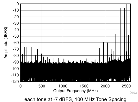
FIG 5-28. Dual Channel Mode: Two Tone FFT at 7997 MHz
