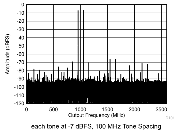
FIG 5-26. Dual Channel Mode: Two Tone FFT at 4197 MHz
