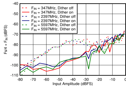
図 5-66. DES Mode: F_s/2 - F_{\text{IN}} vs Input Amplitude and Dither
