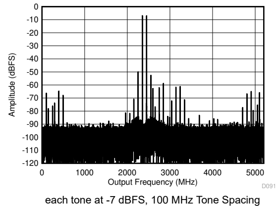
FIG 5-16. DES Mode: Two Tone FFT at 7997 MHz
