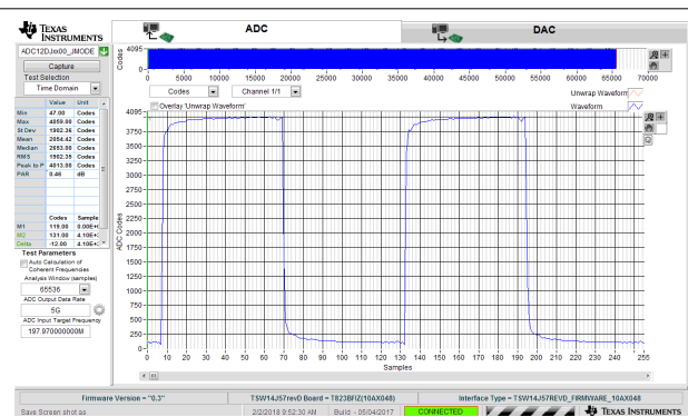
図 7-7. 40-MHz, Square-Wave Time Domain for 5-GSPS, Single-Channel Oscilloscope
