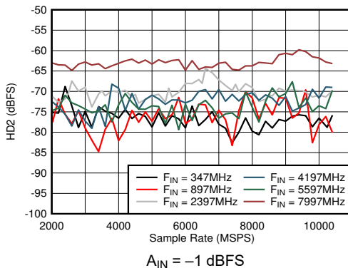
FIG 5-35. DES Mode: HD2 vs Sample Rate and Input Frequency
