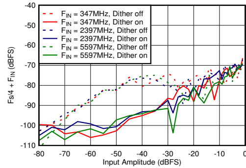
図 5-68. DES Mode: F_s/4 + F_{\text{IN}} vs Input Amplitude and Dither
