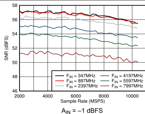
FIG 5-29. DES Mode: SNR vs Sample Rate and Input Frequency
