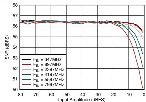
図 5-71. Dual Channel Mode: SNR vs Input Amplitude and Frequency
