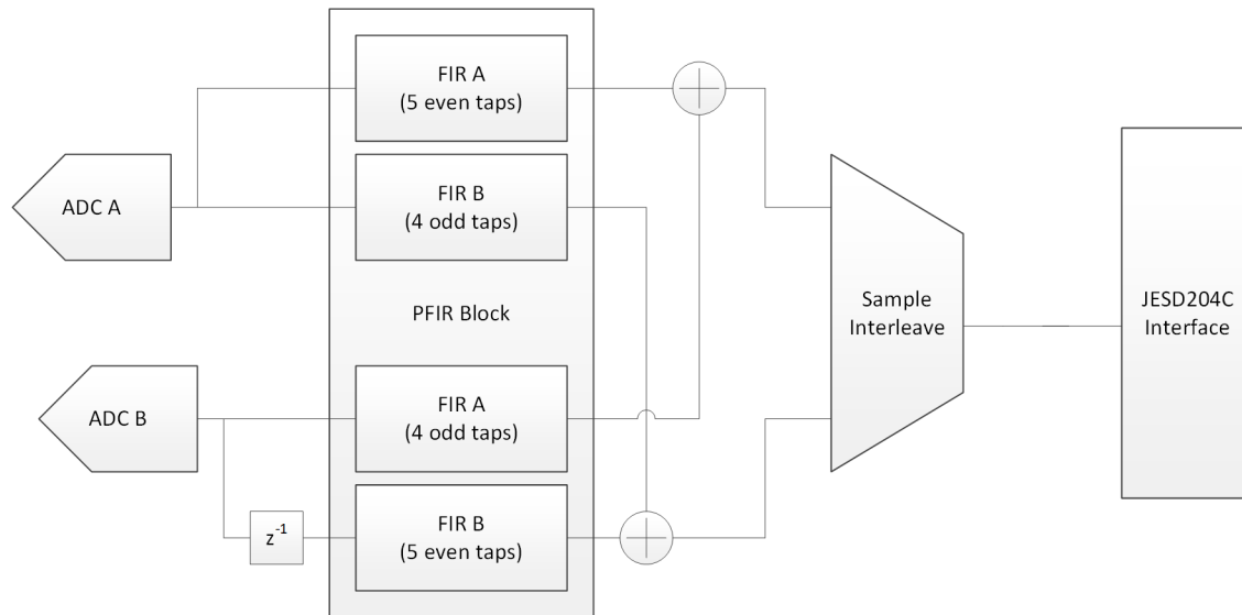
✎ 6-7. Alternate I/Q Correction-Type Filter Block Diagram
