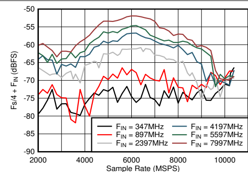
図 5-42. DES Mode: \text{Fs}/4 + F_{\text{IN}} vs Sample Rate and Input Frequency
