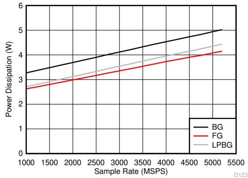
5-139. Dual Channel Mode: Power Dissipation vs Sample Rate
