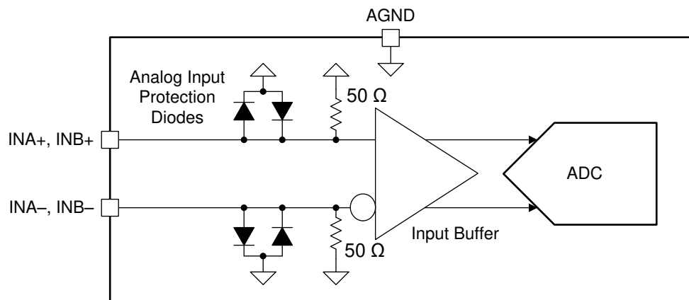
図 6-1. ADC12DJ5200RF Analog Input Internal Termination and Protection Diagram
