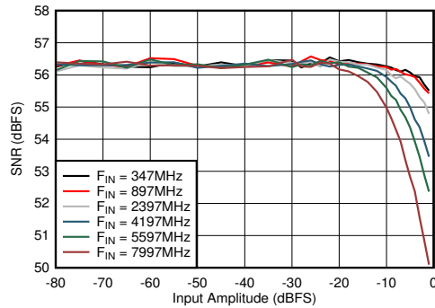
5-57. DES Mode: SNR vs Input Amplitude and Frequency
