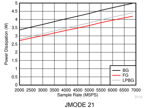
FIG 5-128. DES Mode: Power Dissipation vs Sample Rate
