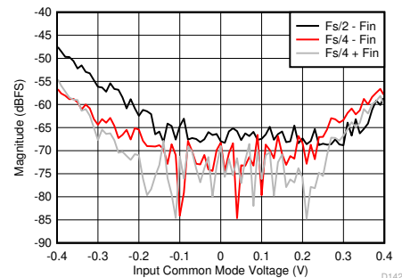
Figure 5-98. F_s/2 - F_{\text{IN}} and F_s/4 \pm F_{\text{IN}} vs Input Common Mode Voltage
