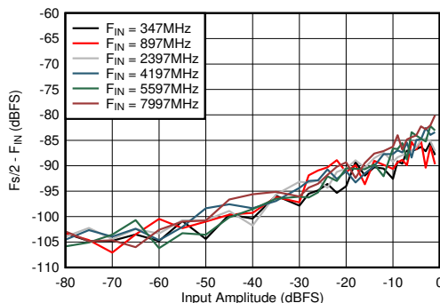
図 5-79. Dual Channel Mode: F_s/2 - F_{\text{IN}} vs Input Amplitude and Frequency
