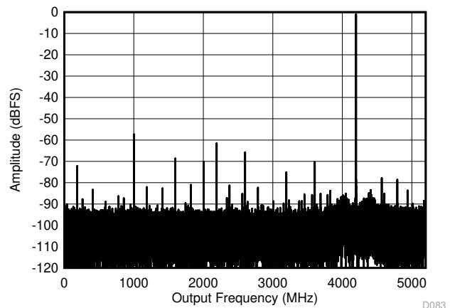
5-8. DES Mode: Single Tone FFT at 4197 MHz
