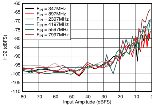
図 5-61. DES Mode: HD2 vs Input Amplitude and Frequency
