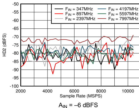
FIG 5-36. DES Mode: HD2 vs Sample Rate and Input Frequency
