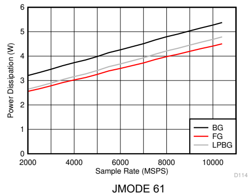
FIG 5-130. DES Mode: Power Dissipation vs Sample Rate
