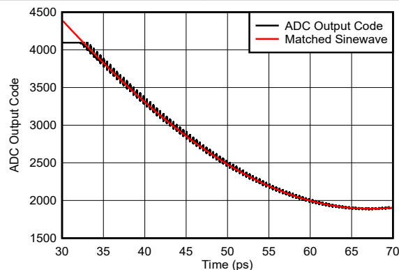
FIG 5-149. Sinewave Overdrive Recovery
