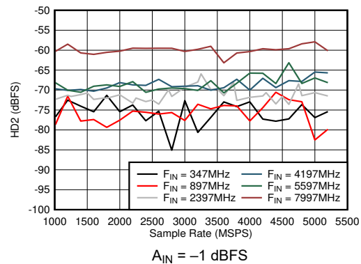
Figure 5-50. Dual Channel Mode: HD2 vs Sample Rate and Input Frequency
