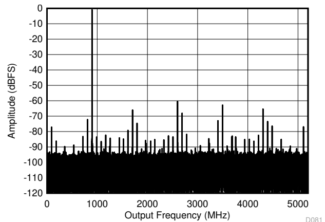
5-6. DES Mode: Single Tone FFT at 897 MHz
