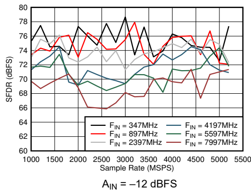
Figure 5-49. Dual Channel Mode: SFDR vs Sample Rate and Input Frequency
