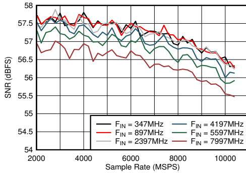
FIG 5-31. DES Mode: SNR vs Sample Rate and Input Frequency
