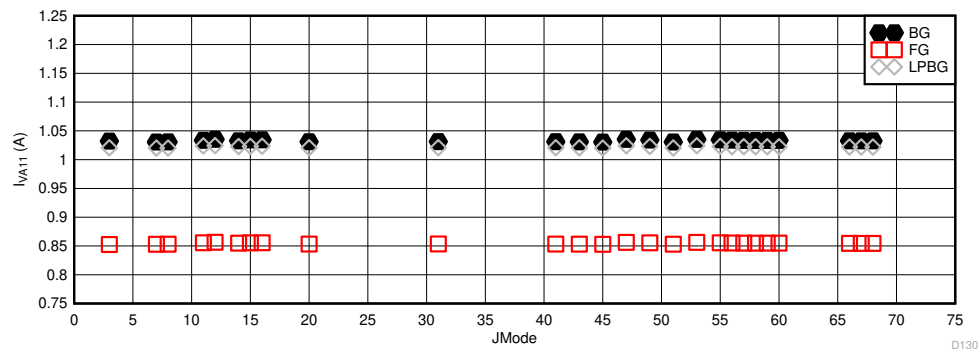
図 5-113. Dual Channel Mode: I_{VA19} vs JMODE at 5.2GSPS
