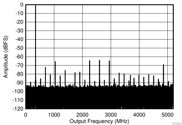
5-5. DES Mode: Single Tone FFT at 347 MHz
