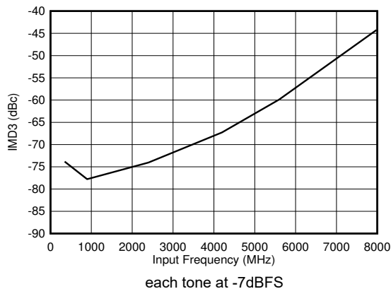
Figure 5-99. DES Mode: IMD3 vs Input Frequency
