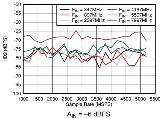
Figure 5-51. Dual Channel Mode: HD2 vs Sample Rate and Input Frequency
