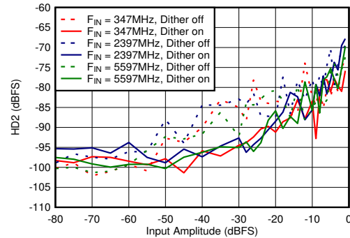
図 5-62. DES Mode: HD2 vs Input Amplitude and Dither
