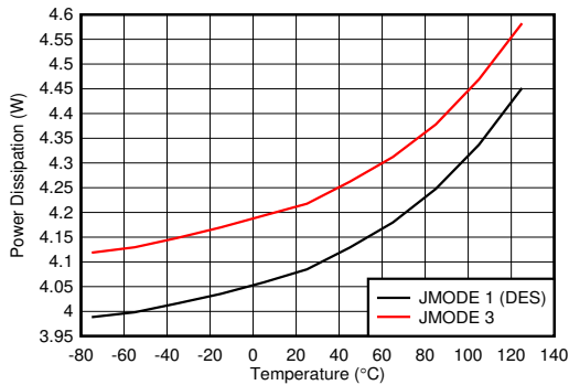
5-141. Power Dissipation vs Temperature
