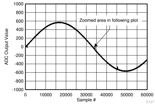
5-142. Background Calibration Core Transition (AC Signal)
