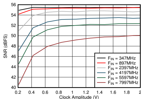
図 5-81. DES Mode: SNR vs Clock Amplitude
