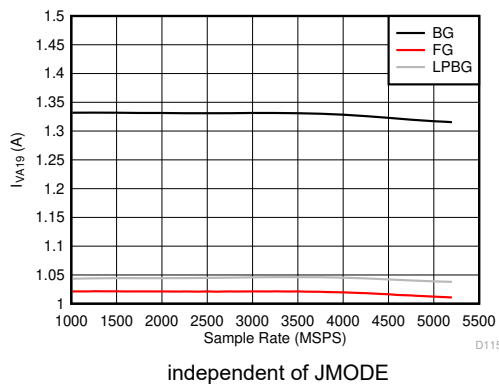
FIG 5-131. Dual Channel Mode: I_{VA19} vs Sample Rate
