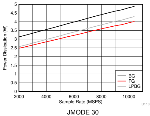
FIG 5-129. DES Mode: Power Dissipation vs Sample Rate
