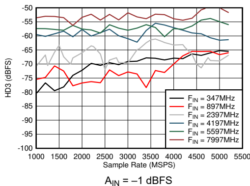
Figure 5-53. Dual Channel Mode: HD3 vs Sample Rate and Input Frequency
