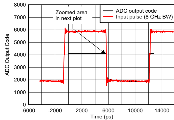
FIG 5-146. Pulse Overdrive Recovery
