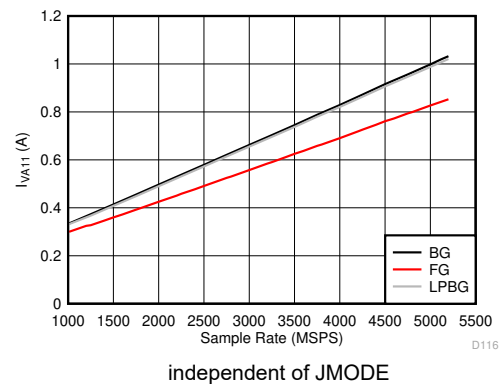
FIG 5-132. Dual Channel Mode: I_{VA11} vs Sample Rate
