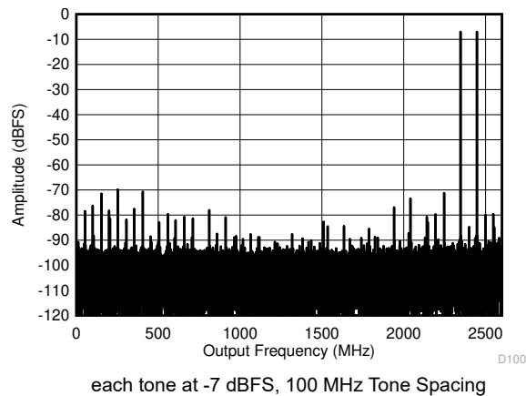
FIG 5-25. Dual Channel Mode: Two Tone FFT at 2397 MHz
