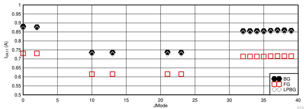
図 5-117. Other Modes with Lower Maximum F_S : I_{VA19} vs JMODE
