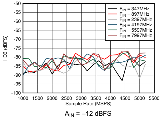
5-55. Dual Channel Mode: HD3 vs Sample Rate and Input Frequency
