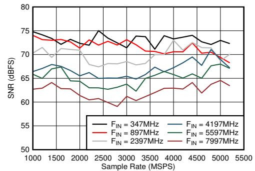
図 5-46. Dual Channel Mode: SNR vs Sample Rate and Input Frequency
