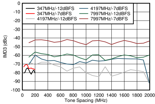
Figure 5-101. DES Mode: IMD3 vs Tone Spacing
