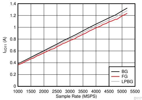
Figure 5-133. Dual Channel Mode: I_{VD11} vs Sample Rate
