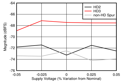
Figure 5-96. Dual Channel Mode: HD2, HD3 and Worst non-HD Spur vs Supply Voltage
