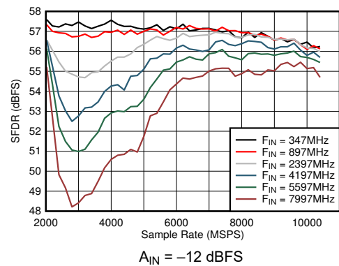
FIG 5-34. DES Mode: SFDR vs Sample Rate and Input Frequency
