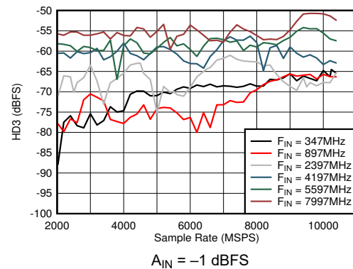
図 5-38. DES Mode: HD3 vs Sample Rate and Input Frequency
