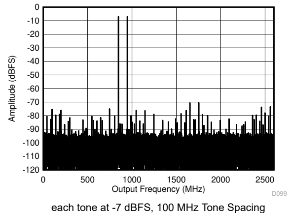
5-24. Dual Channel Mode: Two Tone FFT at 897 MHz
