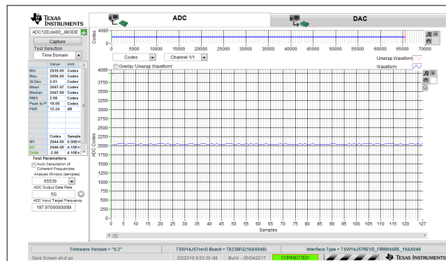
図 7-6. Idle-Channel Noise (No Input) for 5-GSPS, Single-Channel Oscilloscope
