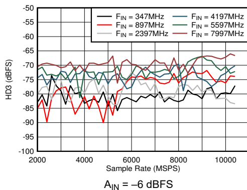
図 5-39. DES Mode: HD3 vs Sample Rate and Input Frequency
