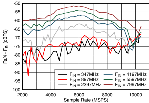
図 5-43. DES Mode: F_s/4 - F_{\text{IN}} vs Sample Rate and Input Frequency
