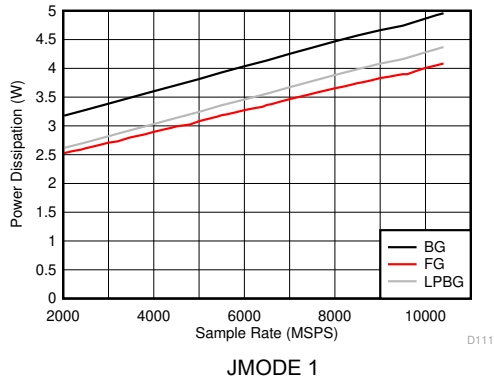
FIG 5-127. DES Mode: Power Dissipation vs Sample Rate
