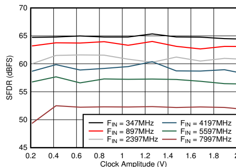
図 5-82. DES Mode: SFDR vs Clock Amplitude
