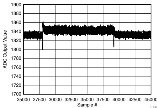
FIG 5-145. Background Calibration Core Transition (DC Signal - zoomed)
