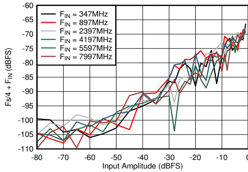
図 5-67. DES Mode: F_s/4 + F_{\text{IN}} vs Input Amplitude and Frequency
