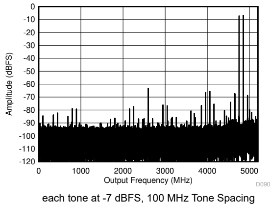
FIG 5-15. DES Mode: Two Tone FFT at 5597 MHz
