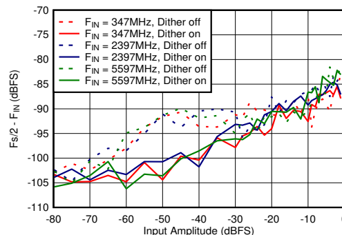
図 5-80. Dual Channel Mode: F_s/2 - F_{\text{IN}} vs Input Amplitude and Dither
