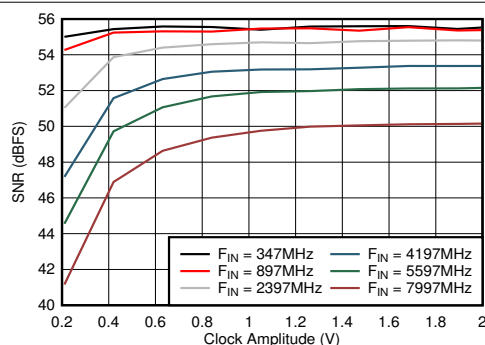
図 5-83. Dual Channel Mode: SNR vs Clock Amplitude
