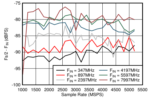
5-56. Dual Channel Mode: F_s/2 - F_{\text{IN}} vs Sample Rate and Input Frequency
