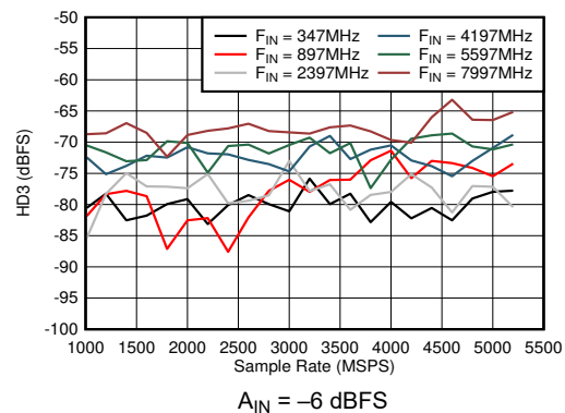
Figure 5-54. Dual Channel Mode: HD3 vs Sample Rate and Input Frequency
