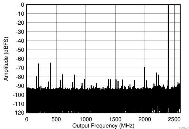
FIG 5-19. Dual Channel Mode: Single Tone FFT at 2397 MHz
