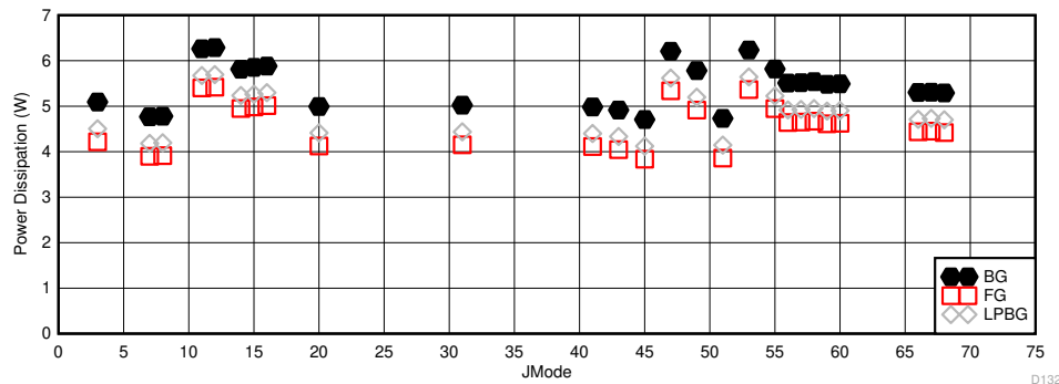
5-115. Dual Channel Mode: I_{VD11} vs JMODE at 5.2GSPS
