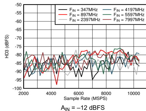
図 5-40. DES Mode: HD3 vs Sample Rate and Input Frequency
