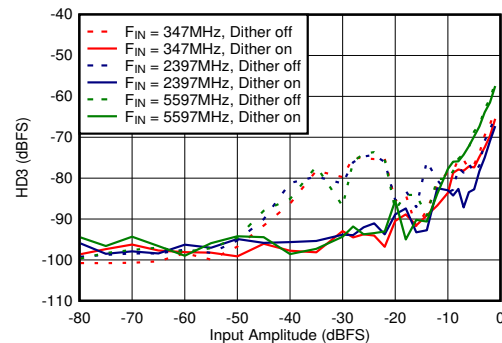
図 5-64. DES Mode: HD3 vs Input Amplitude and Dither
