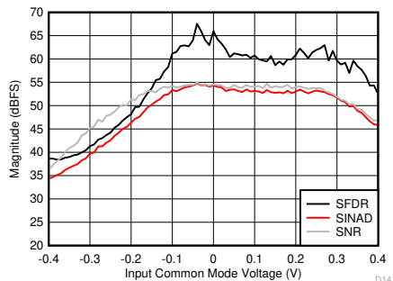
Figure 5-97. SNR, SFDR and SINAD vs Input Common Mode Voltage
