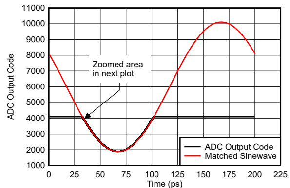
FIG 5-148. Sinewave Overdrive Recovery
