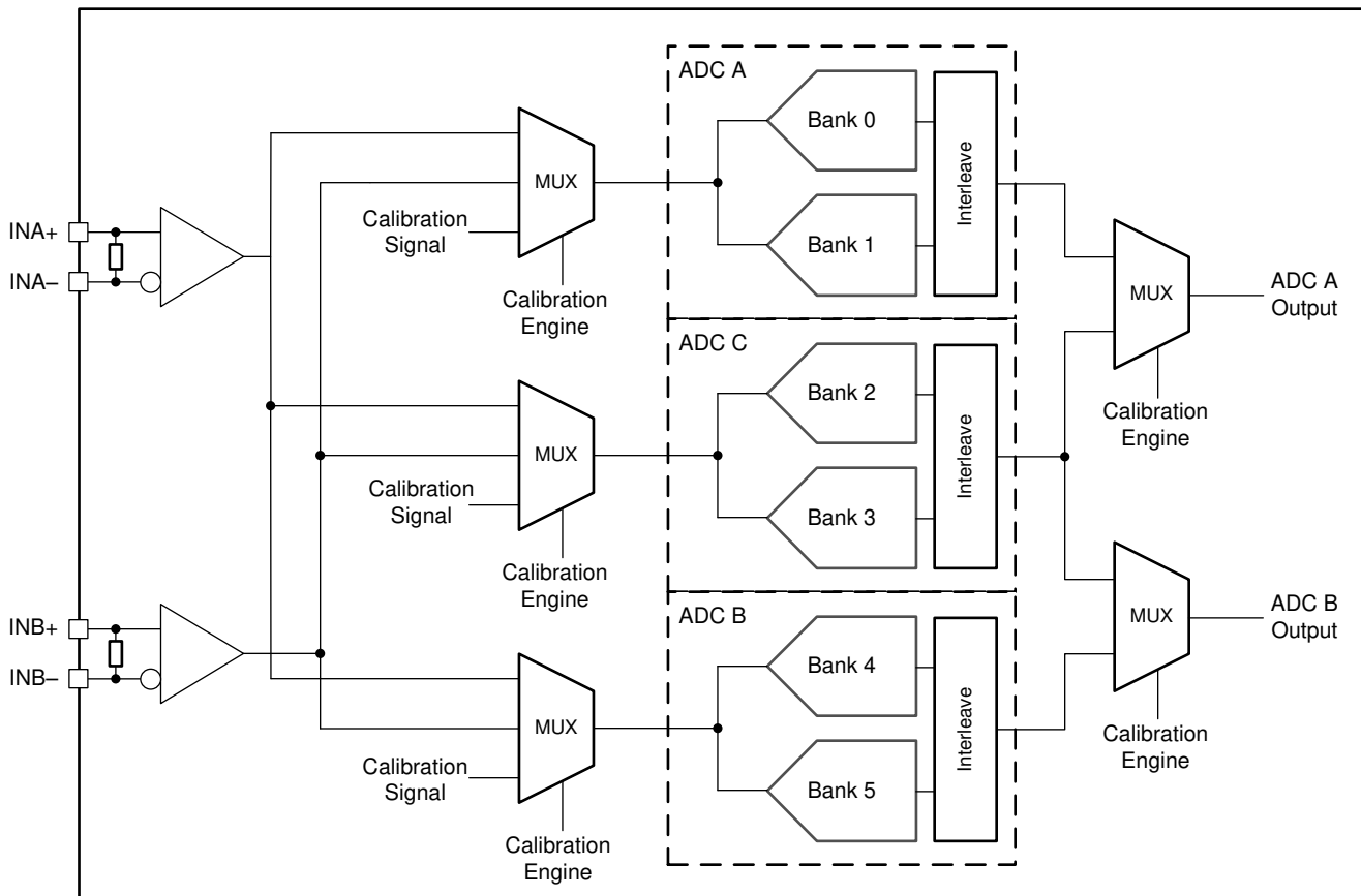
図 6-26. ADC12DJ5200RF Calibration System Block Diagram
