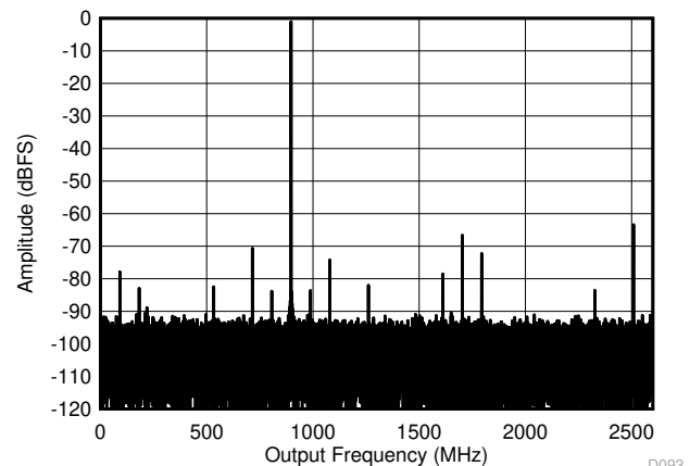
FIG 5-18. Dual Channel Mode: Single Tone FFT at 897 MHz
