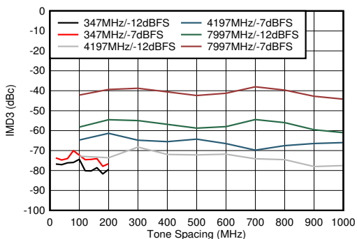
Figure 5-106. Dual Channel Mode: IMD3 vs Tone Spacing
