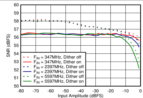
図 5-72. Dual Channel Mode: SNR vs Input Amplitude and Dither
