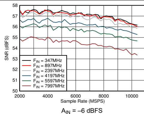
FIG 5-30. DES Mode: SNR vs Sample Rate and Input Frequency
