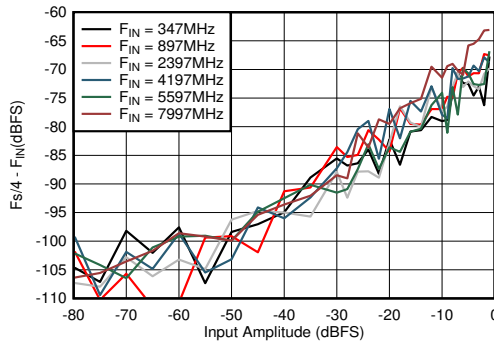
図 5-69. DES Mode: F_s/4 - F_{\text{IN}} vs Input Amplitude and Frequency
