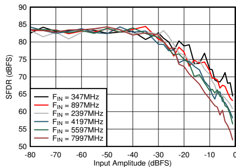
5-59. DES Mode: SFDR vs Input Amplitude and Frequency
