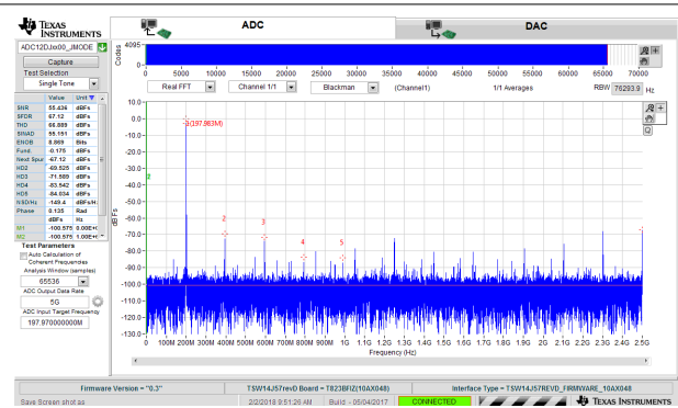
図 7-9. 200-MHz, Sine-Wave Frequency Domain (FFT) for 5-GSPS, Single-Channel Oscilloscope
