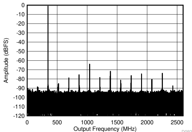
FIG 5-17. Dual Channel Mode: Single Tone FFT at 347 MHz
