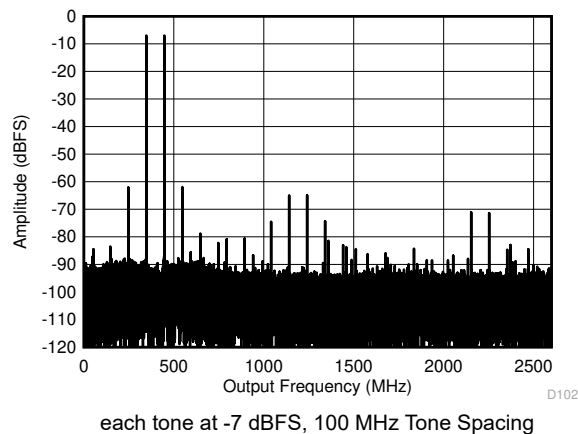
FIG 5-27. Dual Channel Mode: Two Tone FFT at 5597 MHz
