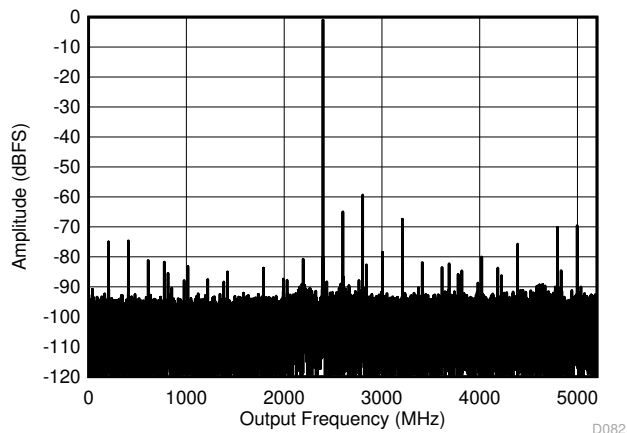
5-7. DES Mode: Single Tone FFT at 2397 MHz
