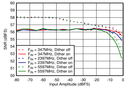
5-58. DES Mode: SNR vs Input Amplitude and Dither
