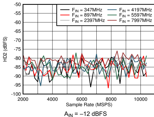
図 5-37. DES Mode: HD2 vs Sample Rate and Input Frequency
