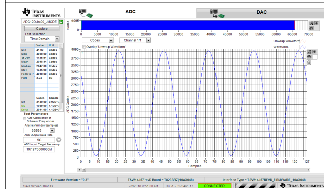
図 7-8. 200-MHz, Sine-Wave Time Domain for 5-GSPS, Single-Channel Oscilloscope
