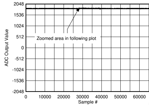
5-144. Background Calibration Core Transition (DC Signal)
