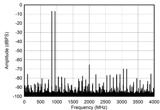
図 6-12. DES Mode: Single Tone FFT at 5597 MHz
