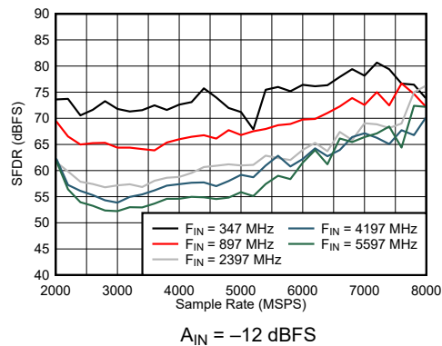
図 6-33. DES Mode: SFDR vs Sample Rate and Input Frequency
