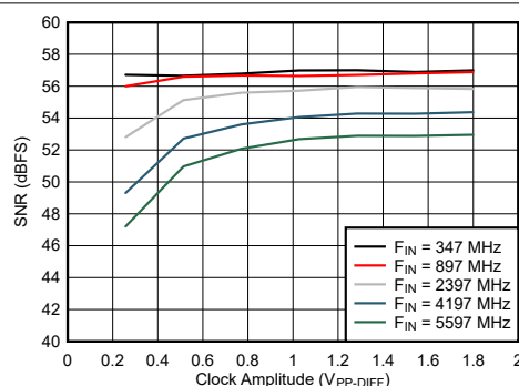
図 6-90. Dual Channel Mode: SNR vs Clock Amplitude
