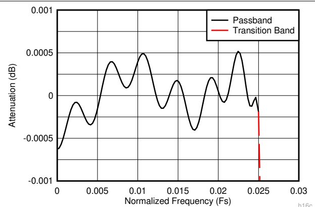
7-16. Decimate-by-16 Composite Zoomed Pass-Band Response
