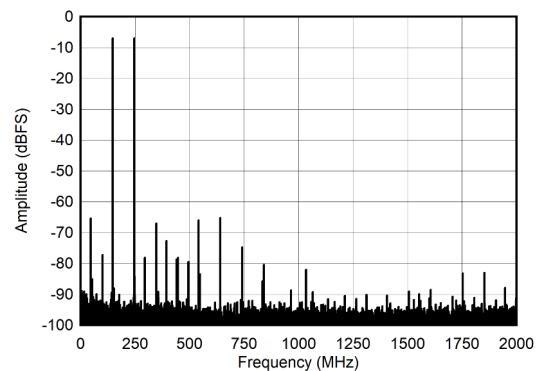
FIG 6-24. Dual Channel Mode: Two Tone FFT at 897 MHz
