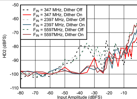
FIG 6-60. DES Mode: HD2 vs Input Amplitude and Dither
