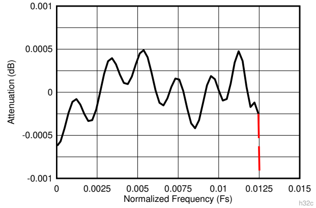
図 7-18. Decimate-by-32 Composite Zoomed Pass-Band Response
