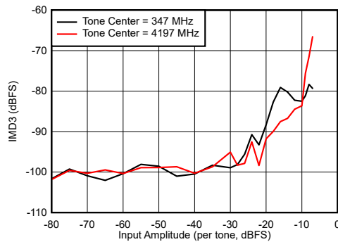
図 6-107. Dual Channel Mode: IMD3 vs Input Amplitude
