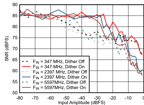
FIG 6-58. DES Mode: SFDR vs Input Amplitude and Dither
