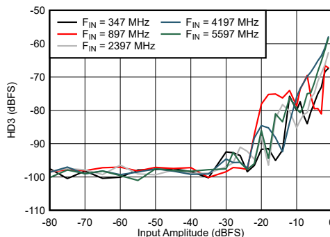
FIG 6-61. DES Mode: HD3 vs Input Amplitude and Frequency
