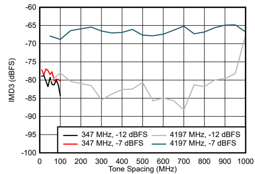
図 6-108. DES Mode: IMD3 vs Tone Spacing
