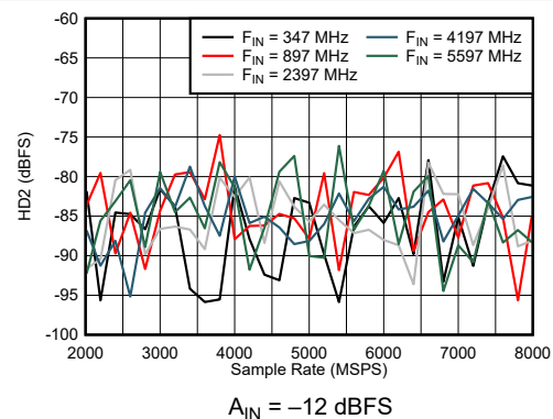
図 6-36. DES Mode: HD2 vs Sample Rate and Input Frequency
