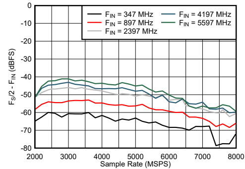
Figure 6-40. DES Mode: F_S/2 - F_{\text{IN}} vs Sample Rate and Input Frequency
