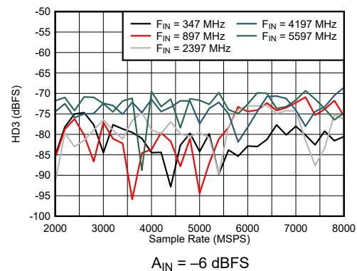
図 6-38. DES Mode: HD3 vs Sample Rate and Input Frequency
