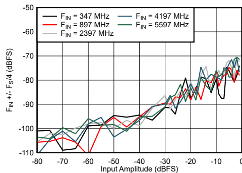
図 6-65. DES Mode: F_{\text{IN}} \pm F_S/4 vs Input Amplitude and Frequency
