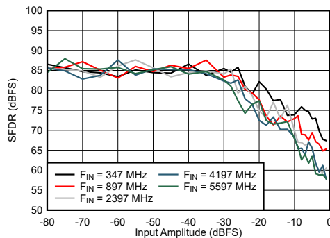
FIG 6-57. DES Mode: SFDR vs Input Amplitude and Frequency
