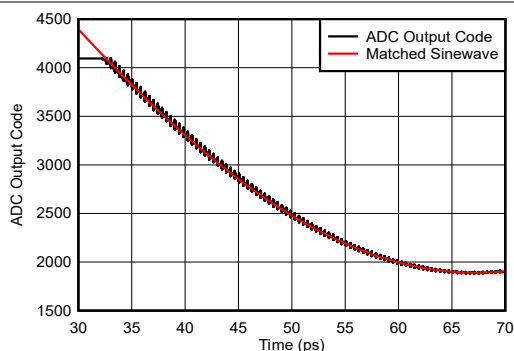
6-144. Sinewave Overdrive Recovery
