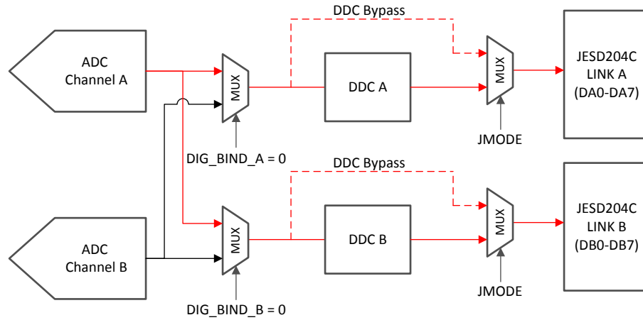
7-24. Dual DDC Mode or Redundant Data Mode for Channel A
