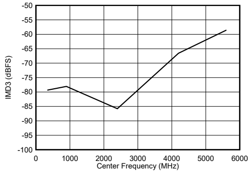
図 6-105. Dual Channel Mode: IMD3 vs Input Frequency
