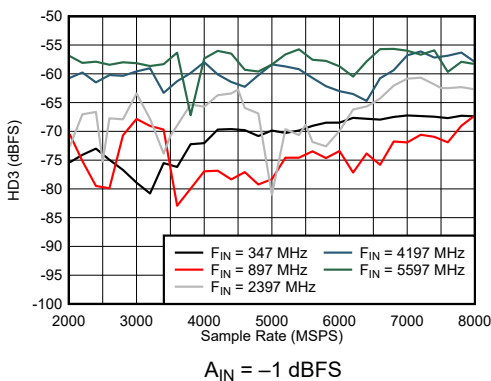
図 6-37. DES Mode: HD3 vs Sample Rate and Input Frequency
