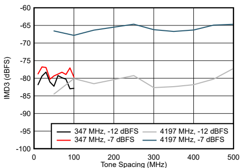
図 6-109. Dual Channel Mode: IMD3 vs Tone Spacing
