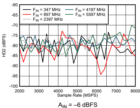
図 6-35. DES Mode: HD2 vs Sample Rate and Input Frequency
