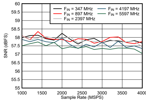
Figure 6-42. Dual Channel Mode: SNR vs Sample Rate and Input Frequency
