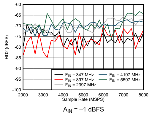
図 6-34. DES Mode: HD2 vs Sample Rate and Input Frequency
