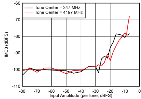
図 6-106. DES Mode: IMD3 vs Input Amplitude
