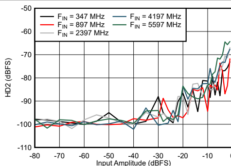
FIG 6-59. DES Mode: HD2 vs Input Amplitude and Frequency
