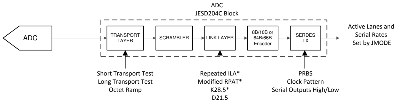
7-25. Test Mode Insertion Points
