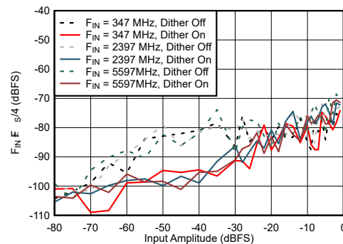
図 6-66. DES Mode: F_{\text{IN}} \pm F_S/4 vs Input Amplitude and Dither
