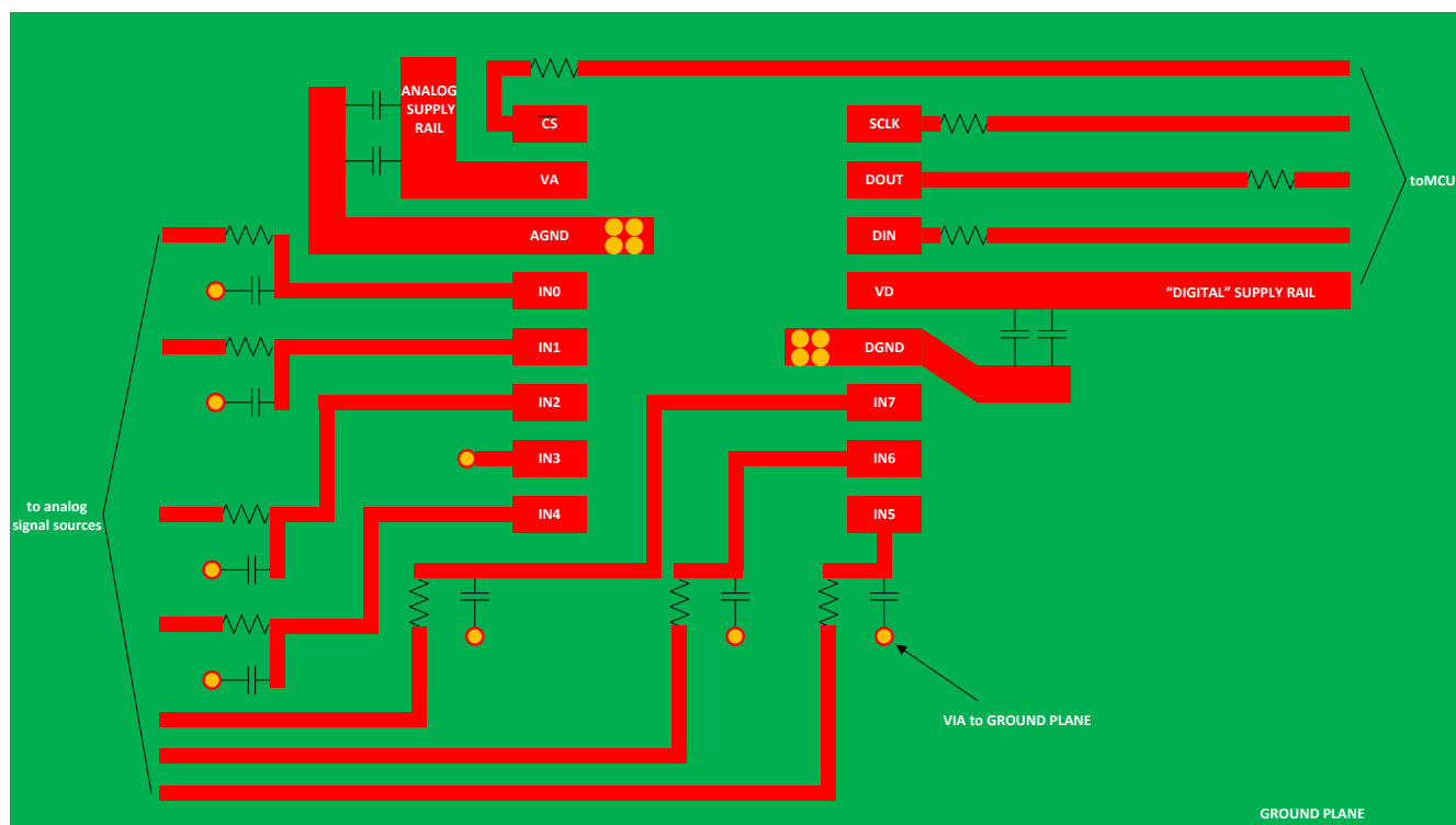
✎ 10-1. Layout Diagram
