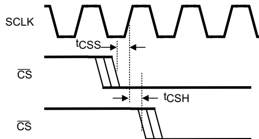
Figure 6-3. SCLK and \overline{CS} Timing Parameters
