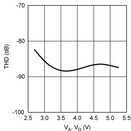
FIG 6-11. THD vs Supply
