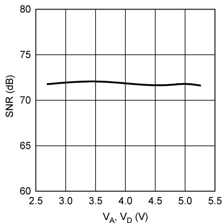
FIG 6-10. SNR vs Supply
