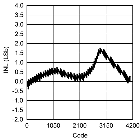
Figure 10. INL vs. Code (External VREF = 5 V, V_+ = 5\text{ V} for 1 Unit)
