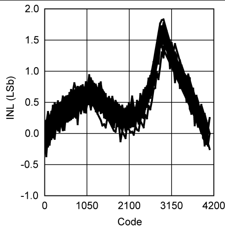
Figure 11. INL vs. Code (External VREF = 5 V, V_+ = 5\text{ V} for 28 Units)
