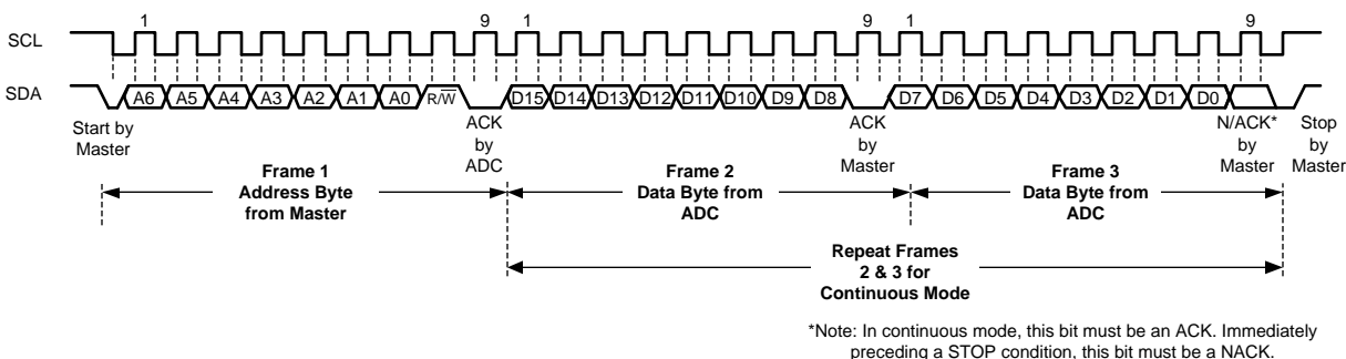
Figure 26. Typical Read from a 2-Byte ADC Register with Preset Pointer
