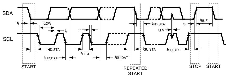
Figure 1. Serial Timing Diagram
