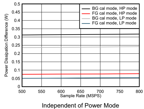
Figure 5-102. Dual Channel, Power Dissipation Change with Calibration Mode
