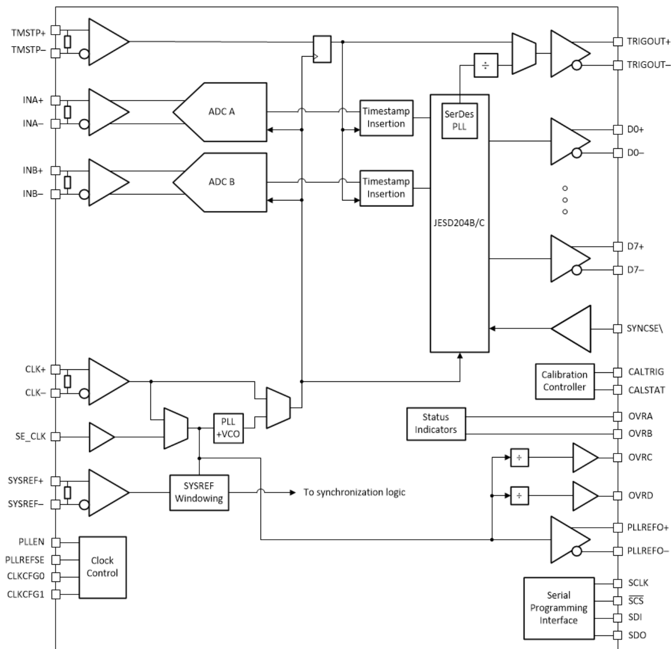
図 6-2. Dual Channel Functional Block Diagram
