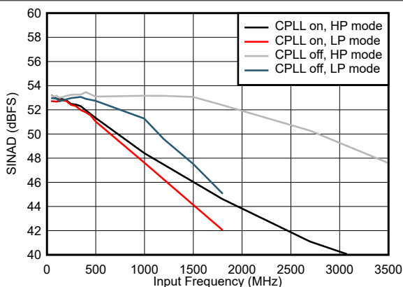
FIG 5-67. SINAD vs Input Frequency and CPLL and Power Mode
