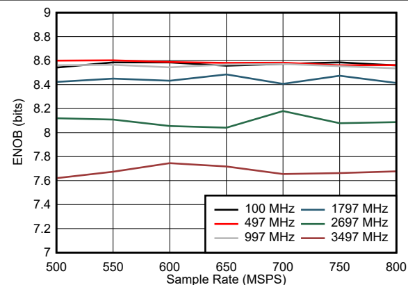
图 5-23. ENOB vs Sample Rate
