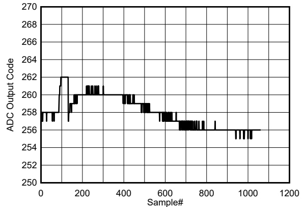
5-116. Background Core Transition (DC midscale input)
