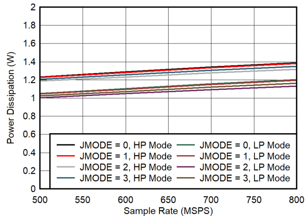
図 5-81. Dual Channel, Power Dissipation vs F_S for JMODES 0 - 3
