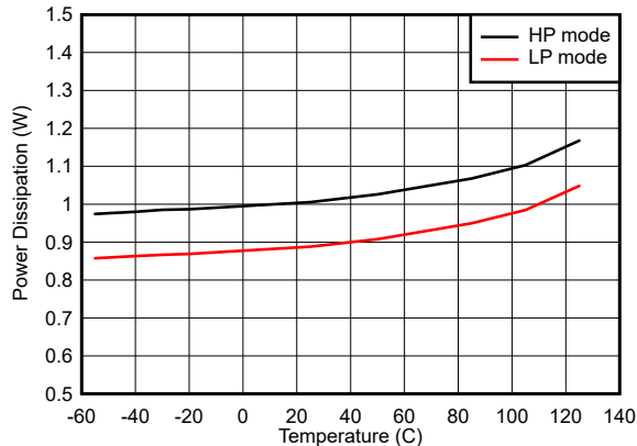
5-113. Quad Channel, Power Dissipation vs Temperature
