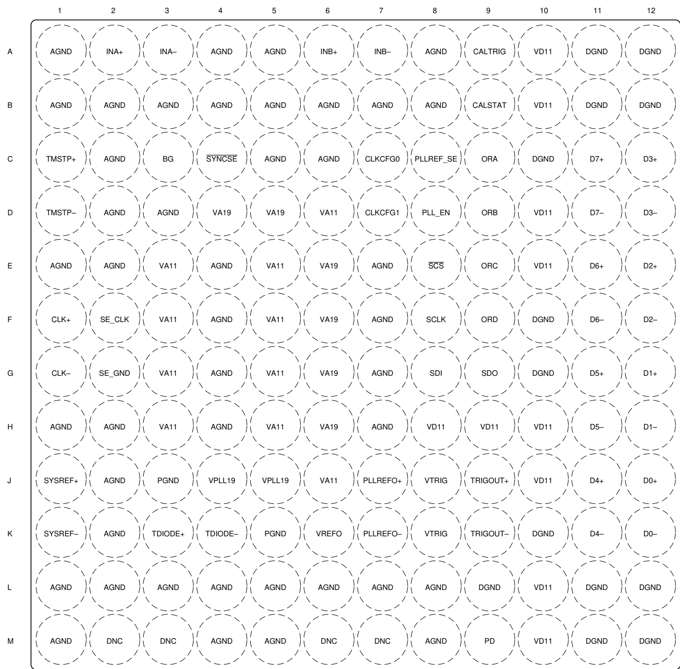
図 4-2. Dual Channel AAV Package, 144-Ball Flip Chip BGA (Top View)
