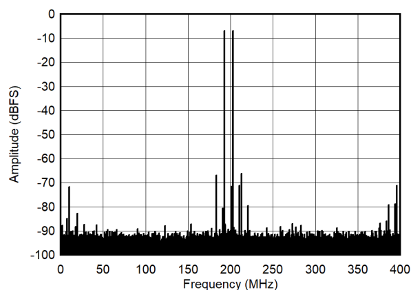
図 5-53. Dual Tone FFT at 1798 MHz
