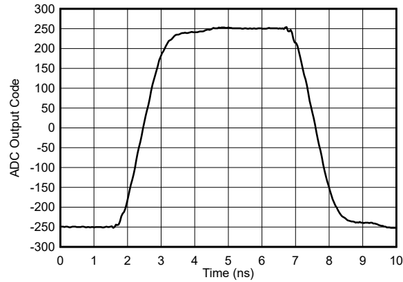
図 7-2. Measured Pulse using Sub-Sampling Technique for Equivalent 25.6 GSPS Measurement
