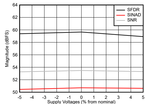
Figure 5-48. SNR, SFDR and SINAD vs Supply Voltage
