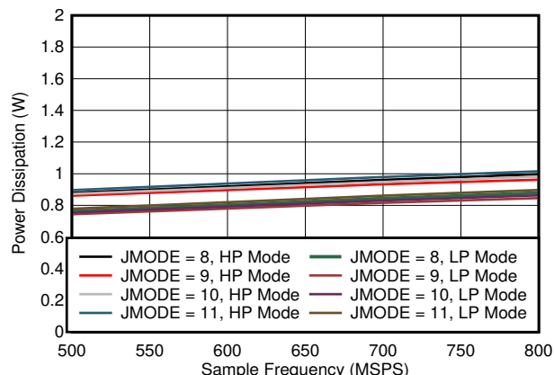
図 5-93. Single Channel, Power Dissipation vs F_S for JMODES 8 - 11
