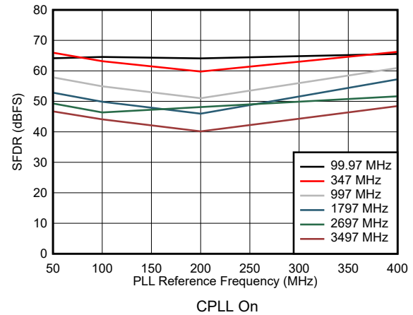
FIG 5-64. SFDR vs Reference Clock Frequency
