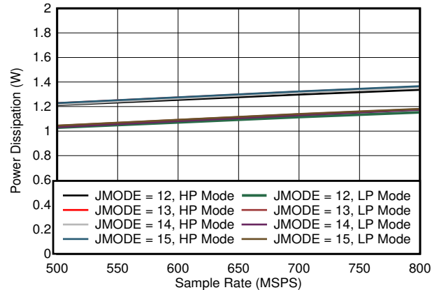
図 5-84. Dual Channel, Power Dissipation vs F_S for JMODES 12 - 15
