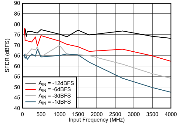
图 5-14. SFDR vs Input Frequency
