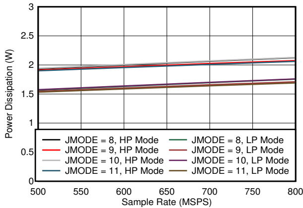
FIG 5-73. Quad Channel, Power Dissipation vs F_S for JMODES 8 - 11
