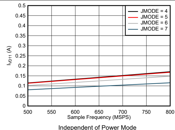
図 5-98. Single Channel, I_{VD11} vs F_S for JMODES 4 - 7
