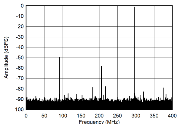
図 5-9. Single Tone FFT at 3497 MHz and -1dBFS
