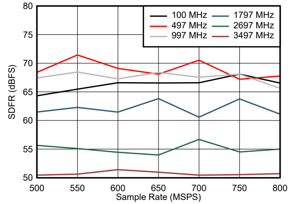
图 5-20. SFDR vs Sample Rate
