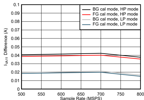
Figure 5-107. Quad Channel, I_{VA11} Change with Calibration Mode
