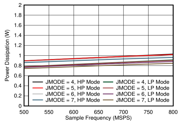
Figure 5-92. Single Channel, Power Dissipation vs F_S for JMODES 4 - 7
