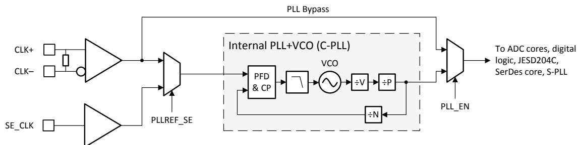
図 6-6. Converter PLL (C-PLL) Architecture
