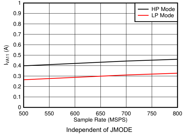
Figure 5-76. Quad Channel, I_{VA11} vs F_S
