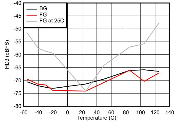
Figure 5-44. HD3 vs Temperature
