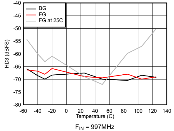
Figure 5-38. HD3 vs Temperature
