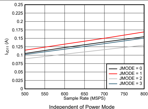
図 5-97. Single Channel, I_{VD11} vs F_S for JMODES 0 - 3
