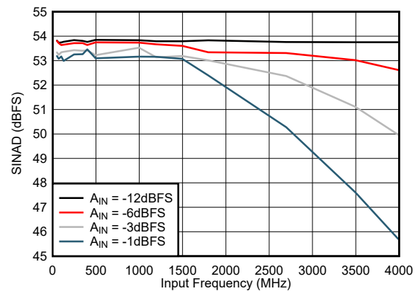
图 5-16. SINAD vs Input Frequency
