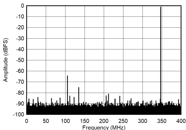
図 5-4. Single Tone FFT at 347 MHz and -1dBFS
