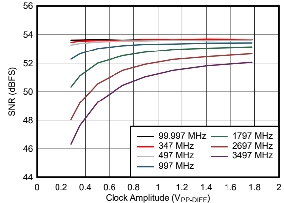
Figure 5-32. SNR vs Clock Amplitude
