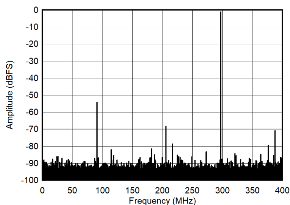
図 5-8. Single Tone FFT at 2697 MHz and -1dBFS
