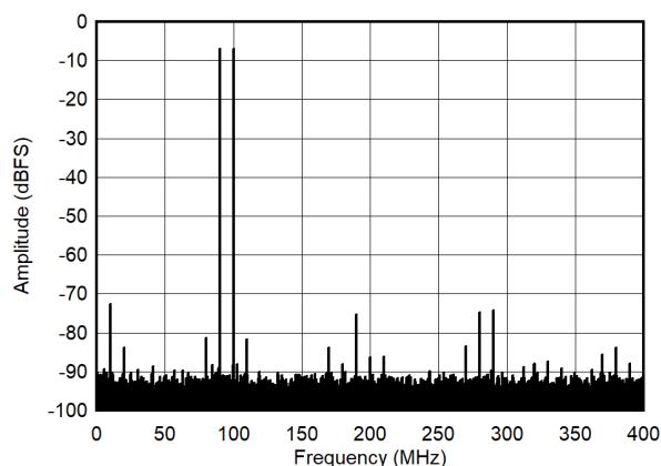
図 5-56. Dual Tone FFT at 95 MHz (LP Mode)
