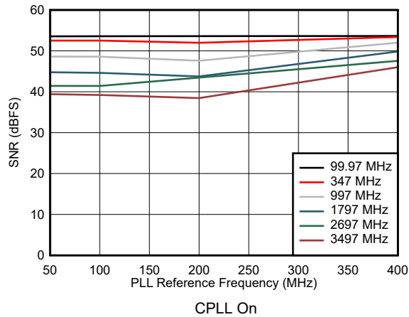
FIG 5-63. SNR vs Reference Clock Frequency
