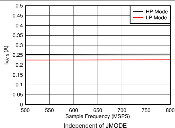
図 5-95. Single Channel, I_{VA19} vs F_S
