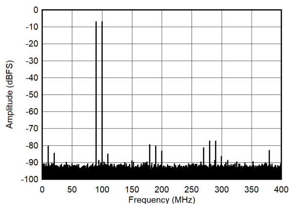
図 5-50. Dual Tone FFT at 95 MHz
