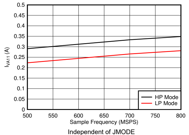
図 5-86. Dual Channel, I_{VA11} vs F_S
