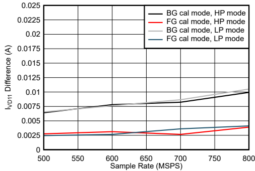
5-111. Dual Channel, I_{VD11} Change with Calibration Mode
