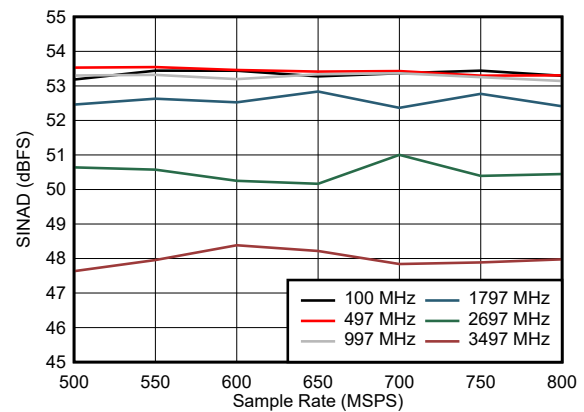
图 5-22. SINAD vs Sample Rate
