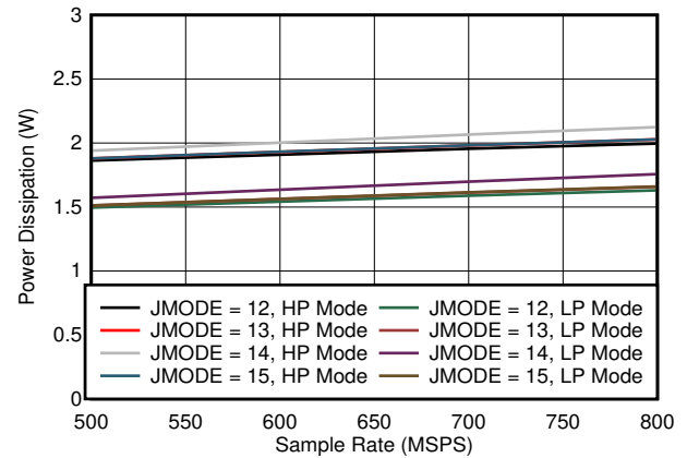
FIG 5-74. Quad Channel, Power Dissipation vs F_S for JMODES 12 - 15
