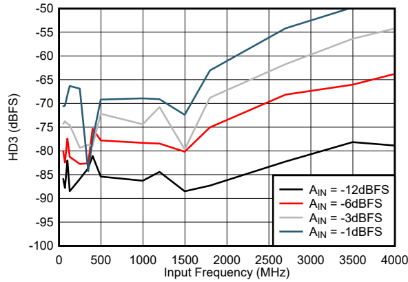
图 5-19. HD3 vs Input Frequency
