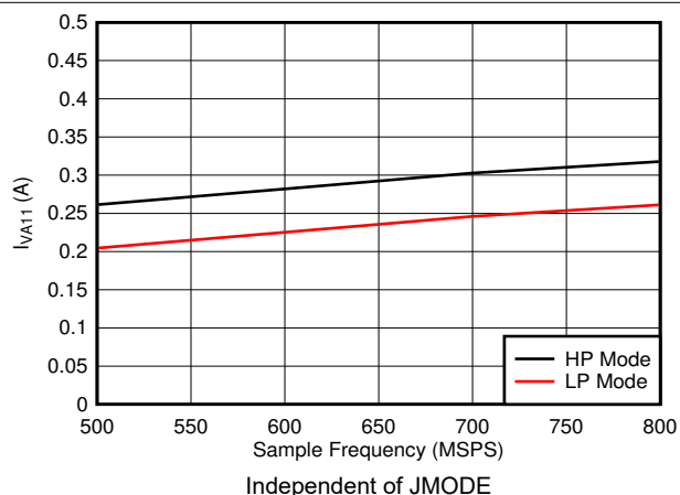
図 5-96. Single Channel, I_{VA11} vs F_S
