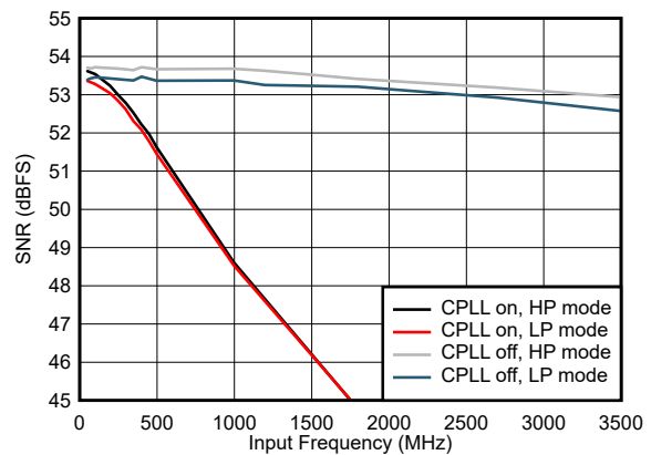
FIG 5-66. SNR vs Input Frequency and CPLL and Power Mode
