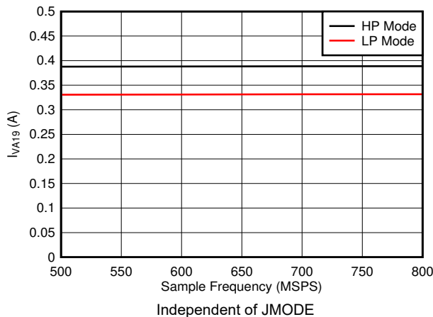
図 5-85. Dual Channel, I_{VA19} vs F_S
