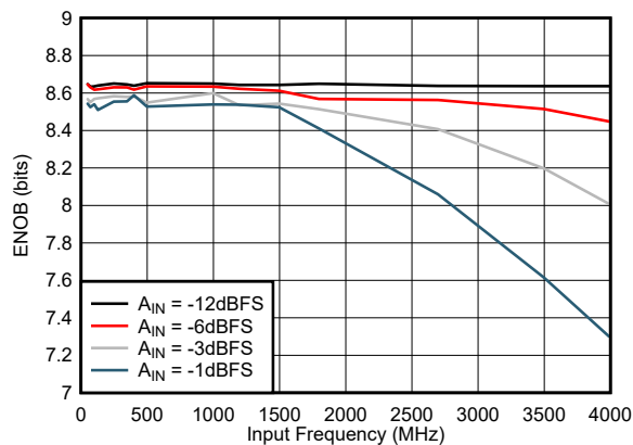
图 5-17. ENOB vs Input Frequency
