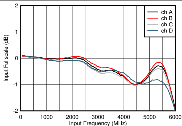
図 5-3. Input Fullscale vs Input Frequency
