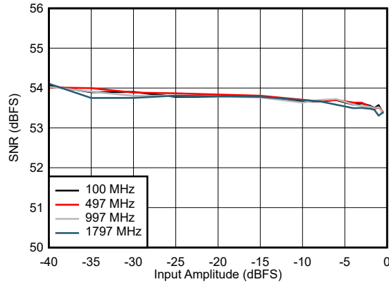
Figure 5-31. SNR vs Input Amplitude
