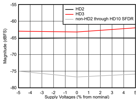
図 5-49. HD2, HD3 and Worst non-HD2/3 Spur vs Supply Voltage
