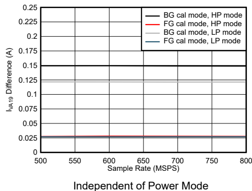
Figure 5-104. Quad Channel, I_{VA19} Change with Calibration Mode
