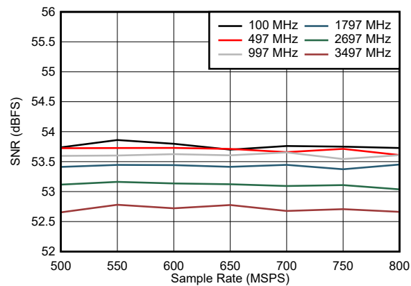
图 5-21. SNR vs Sample Rate
