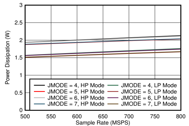
FIG 5-72. Quad Channel, Power Dissipation vs F_S for JMODES 4 - 7
