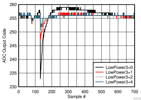
図 6-12. Background Calibration Core Transition In Low Power Mode
