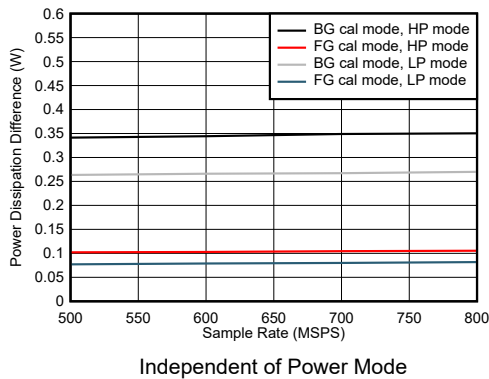
Figure 5-101. Quad Channel, Power Dissipation Change with Calibration Mode
