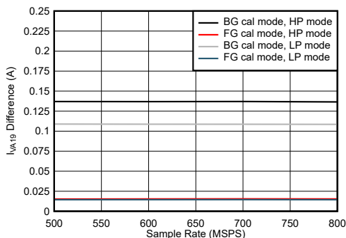
Figure 5-105. Dual Channel, I_{VA19} Change with Calibration Mode
