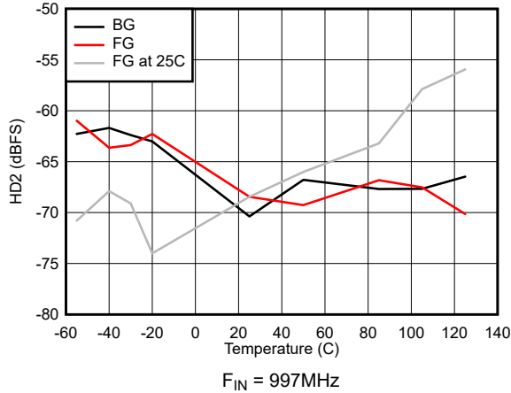
Figure 5-37. HD2 vs Temperature
