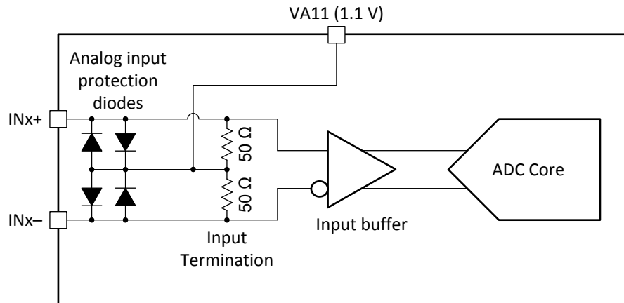
図 6-4. Analog Input Internal Termination and Protection Diagram
