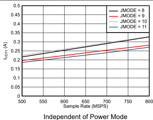
Figure 5-79. Quad Channel, I_{VD11} vs F_S for JMODES 8 - 11
