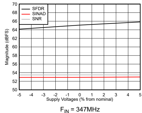
Figure 5-46. SNR, SFDR and SINAD vs Supply Voltage
