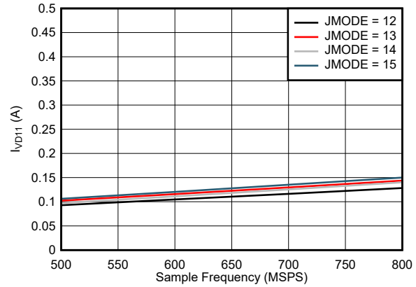
Figure 5-100. Single Channel, I_{VD11} vs F_S for JMODES 12 - 15
