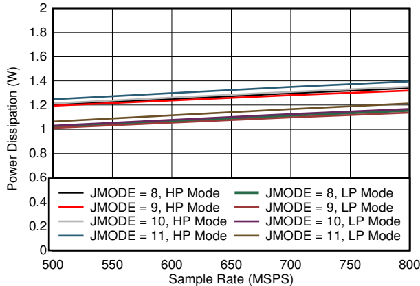
図 5-83. Dual Channel, Power Dissipation vs F_S for JMODES 8 - 11
