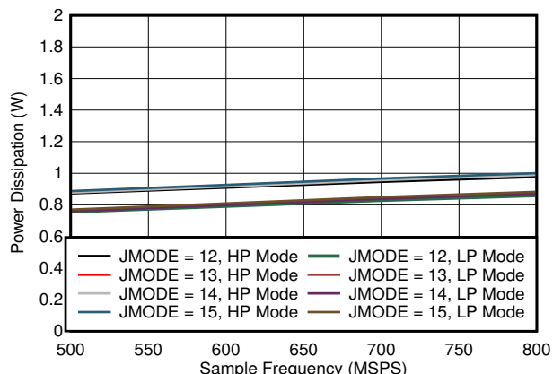
図 5-94. Single Channel, Power Dissipation vs F_S for JMODES 12 - 15
