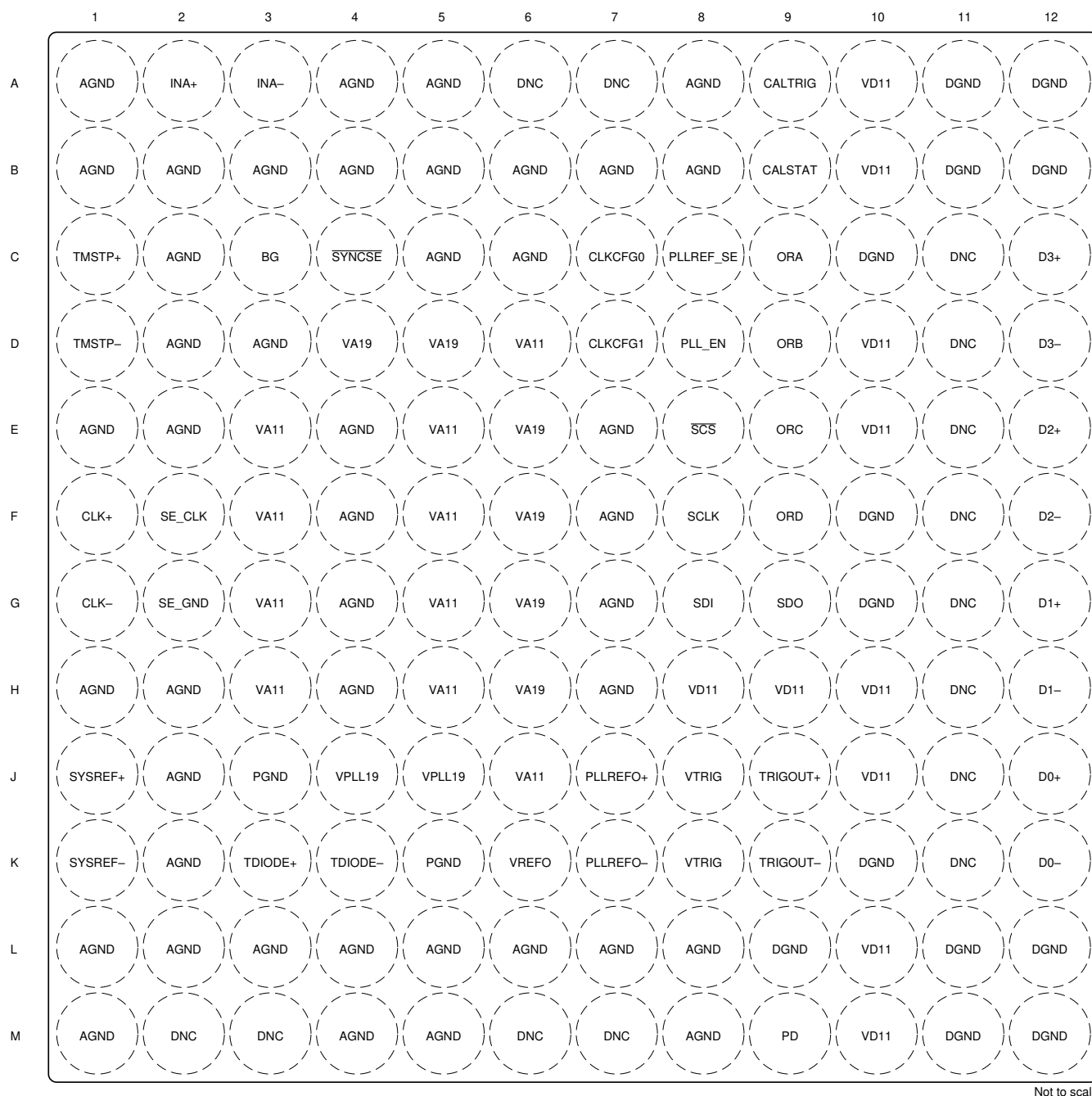
図 4-3. Single Channel AAV Package, 144-Ball Flip Chip BGA (Top View)
