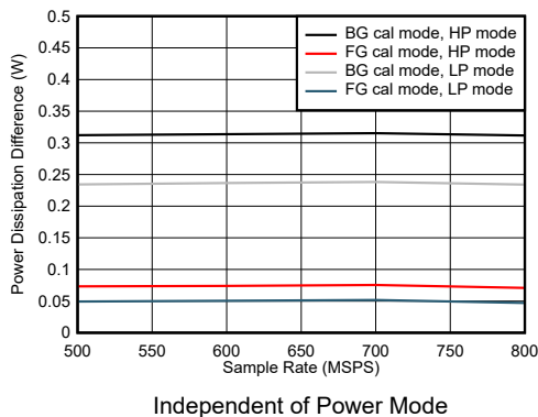
Figure 5-103. Single Channel, Power Dissipation Change with Calibration Mode
