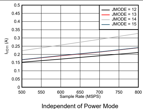
Figure 5-80. Quad Channel, I_{VD11} vs F_S for JMODES 12 - 15
