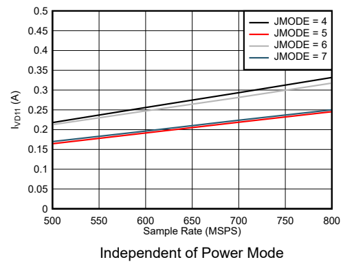
Figure 5-78. Quad Channel, I_{VD11} vs F_S for JMODES 4 - 7
