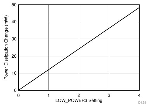
図 6-13. Power Dissipation Change vs LOW_POWER3 register setting
