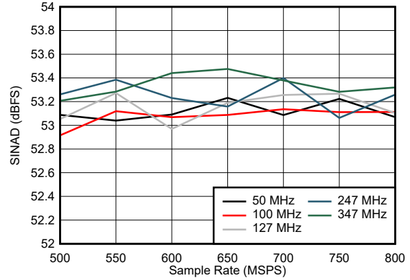
図 5-26. SINAD vs Sample Rate
