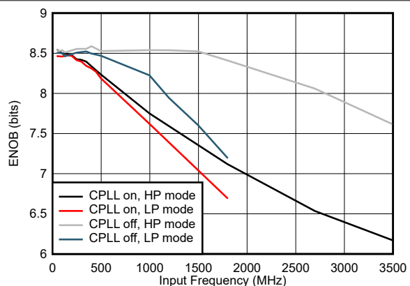
FIG 5-68. ENOB vs Input Frequency and CPLL and Power Mode
