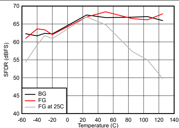
Figure 5-35. SFDR vs Temperature
