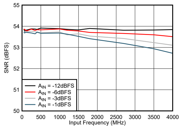
图 5-15. SNR vs Input Frequency
