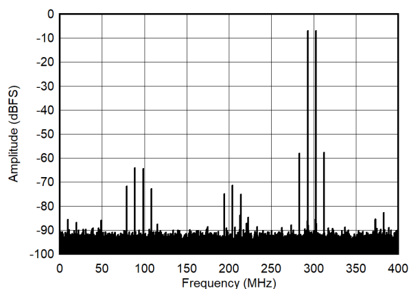
図 5-54. Dual Tone FFT at 2698 MHz
