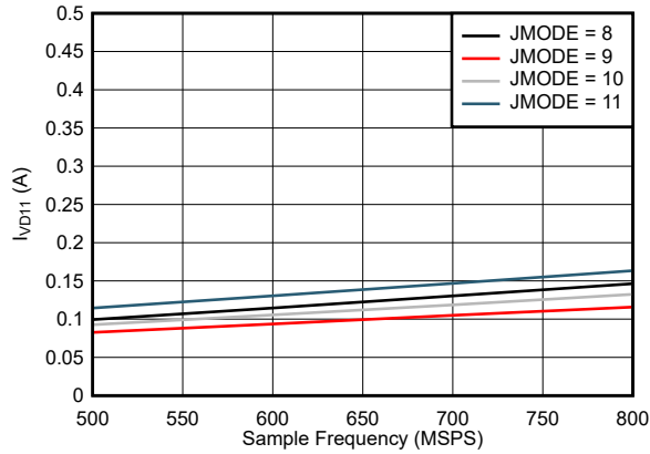
Figure 5-99. Single Channel, I_{VD11} vs F_S for JMODES 8 - 11
