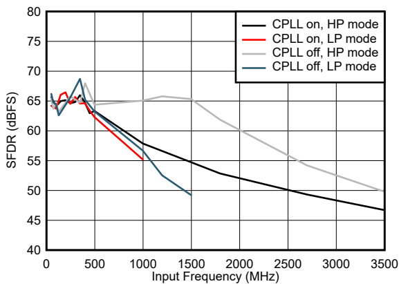
FIG 5-65. SFDR vs Input Frequency and CPLL and Power Mode
