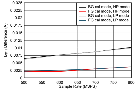
5-112. Single Channel, I_{VD11} Change with Calibration Mode
