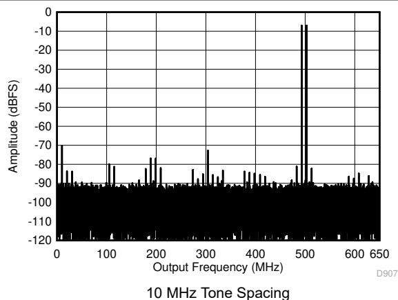
図 5-50. Two Tone FFT at 498 MHz Center
