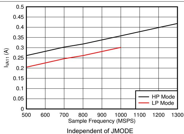
5-106. Single Channel, I_{VA11} vs FS
