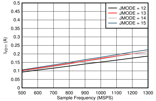
5-110. Single Channel, I_{VD11} vs FS and JMODE 12 - 15
