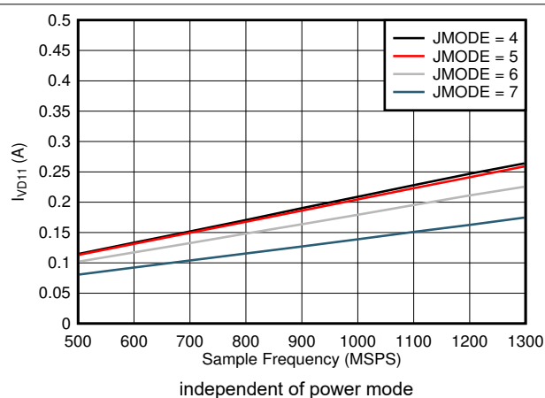
5-108. Single Channel, I_{VD11} vs FS and JMODE 4 - 7
