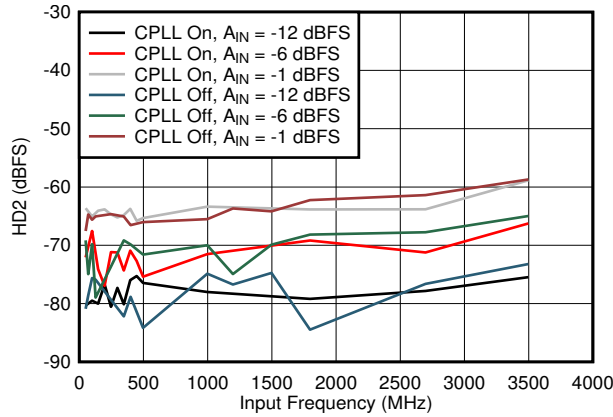
5-73. HD2 vs Input Frequency, CPLL and Input Amplitude
