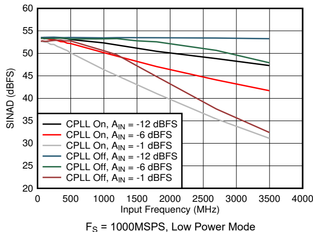
5-77. SINAD vs Input Frequency, CPLL and Input Amplitude
