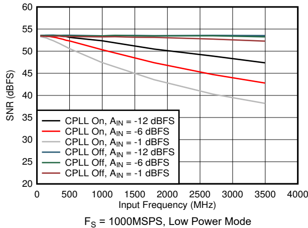
5-75. SNR vs Input Frequency, CPLL and Input Amplitude
