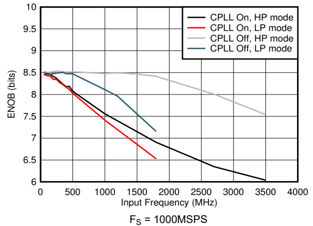
図 5-68. ENOB vs Input Frequency and CPLL
