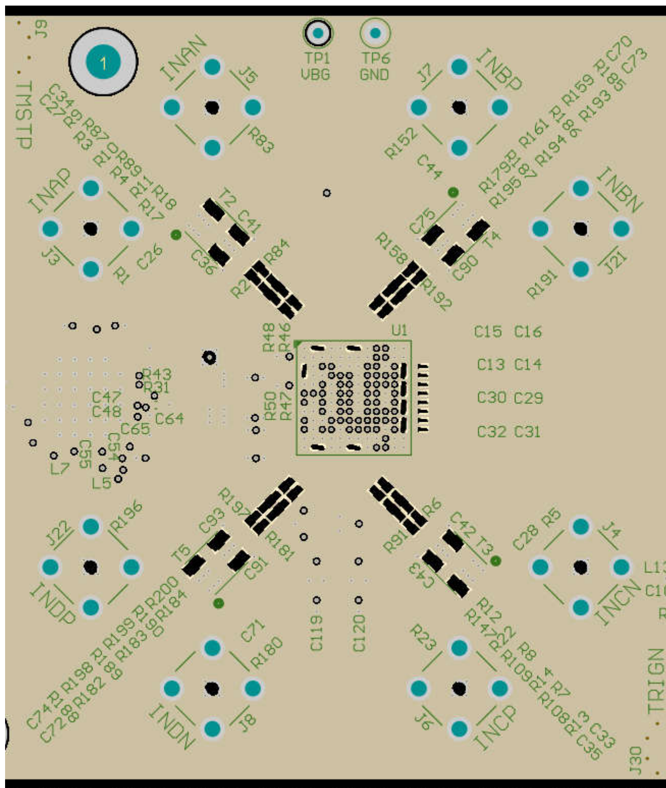
7-7. GND1 Cutouts to Optimize Impedance of Component Pads
