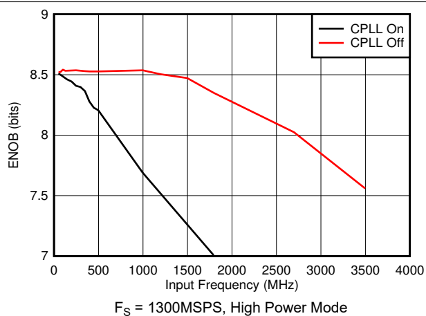
5-64. ENOB vs Input Frequency and CPLL
