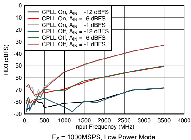
5-80. HD3 vs Input Frequency, CPLL and Input Amplitude
