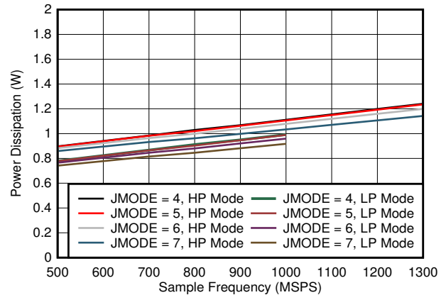
5-102. Single Channel, Power Dissipation vs FS for JMODES 4 - 7
