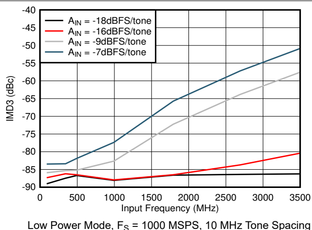
図 5-58. IMD3 vs Input Frequency
