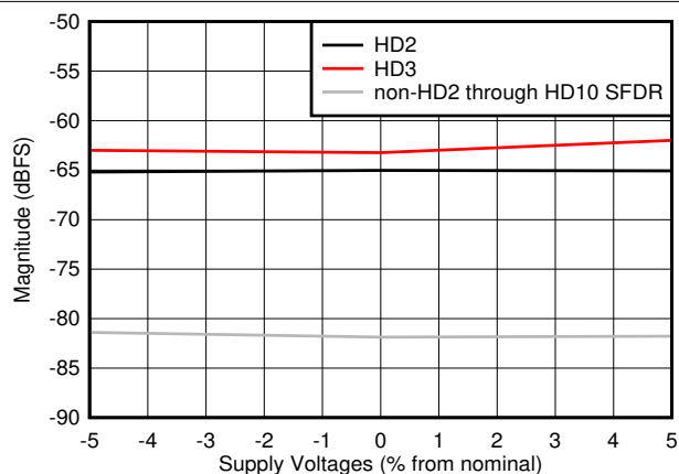
Figure 5-45. HD2, HD3 and Worst non-HD Spur vs Supply Voltage
