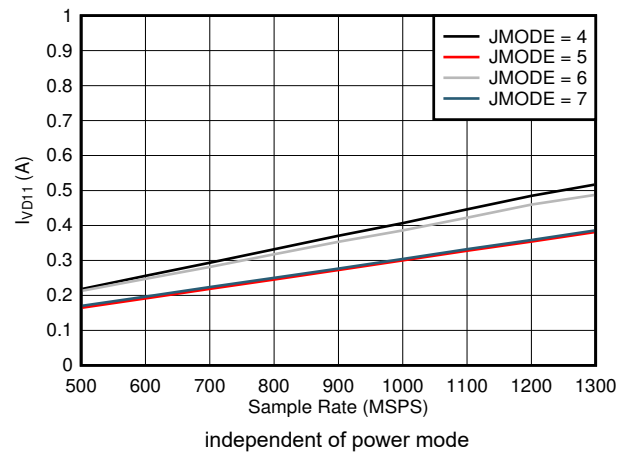
図 5-88. Quad Channel, I_{VD11} vs FS and JMODE 4 - 7
