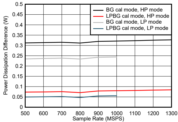
5-111. Quad Channel, Power Dissipation Change with Calibration Mode
