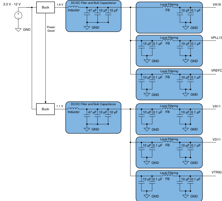
図 7-5. Switcher-Only Approach Example
