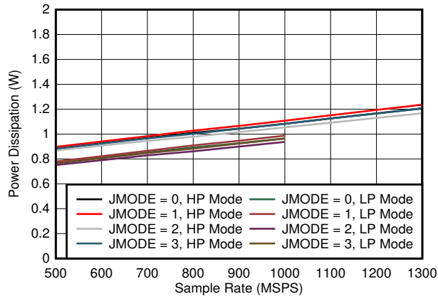
5-101. Single Channel, Power Dissipation vs FS for JMODES 0 - 3
