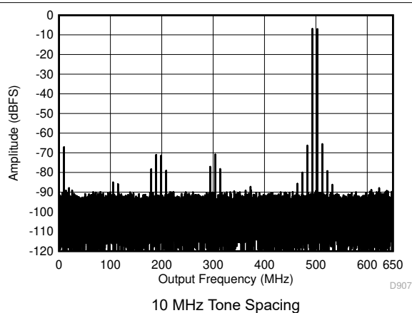
図 5-52. Two Tone FFT at 1798 MHz Center
