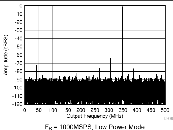
図 5-12. Single Tone FFT at 347 MHz and -1 dBFS
