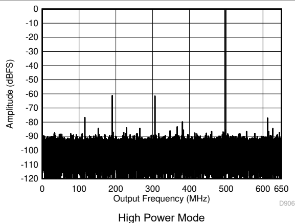
図 5-8. Single Tone FFT at 1797 MHz and -1 dBFS
