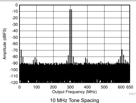
図 5-51. Two Tone FFT at 998 MHz Center
