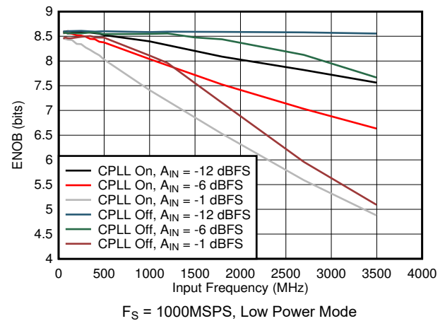
5-78. ENOB vs Input Frequency, CPLL and Input Amplitude
