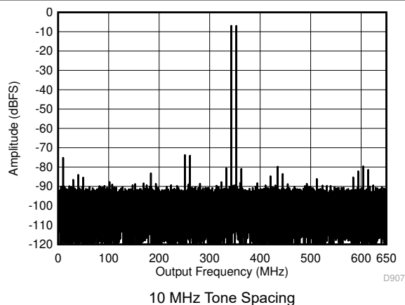
図 5-49. Two Tone FFT at 348 MHz Center
