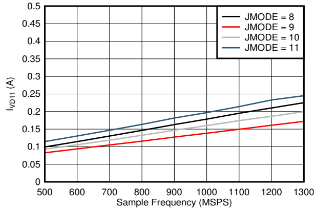
5-109. Single Channel, I_{VD11} vs FS and JMODE 8 - 11
