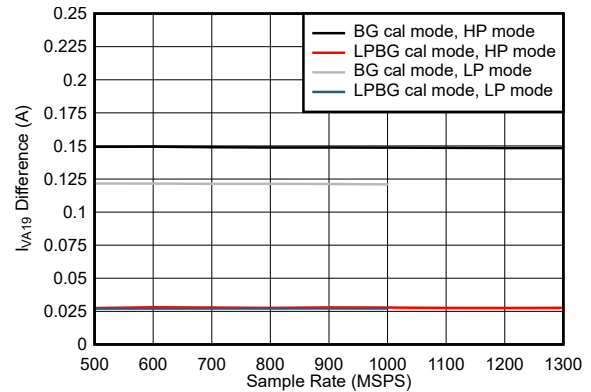
5-112. Dual Channel, Power Dissipation Change with Calibration Mode
