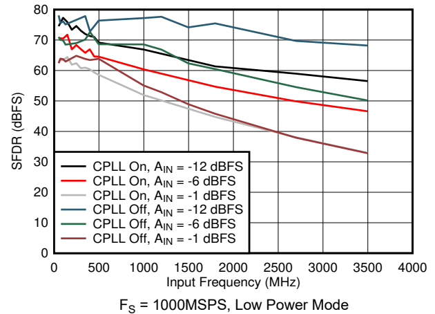
5-76. SFDR vs Input Frequency, CPLL and Input Amplitude
