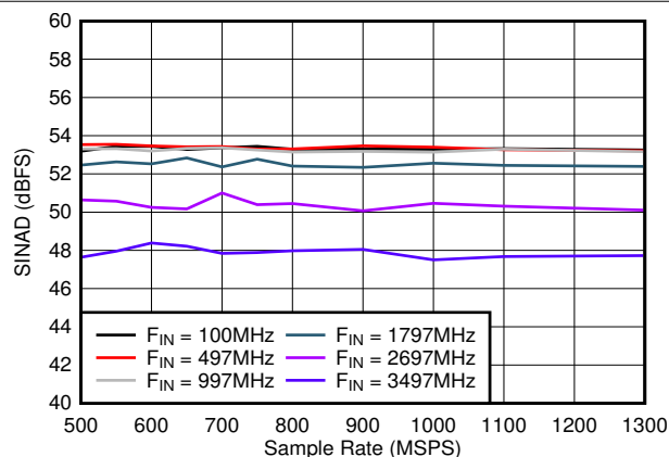
図 5-23. SINAD vs Sample Rate
