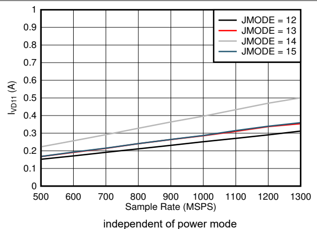
図 5-90. Quad Channel, I_{VD11} vs FS and JMODE 12 - 15
