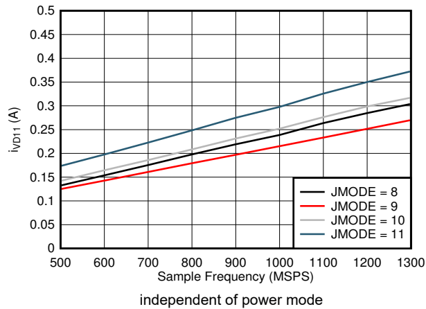
5-99. Dual Channel, I_{VD11} vs FS and JMODE 8 - 11
