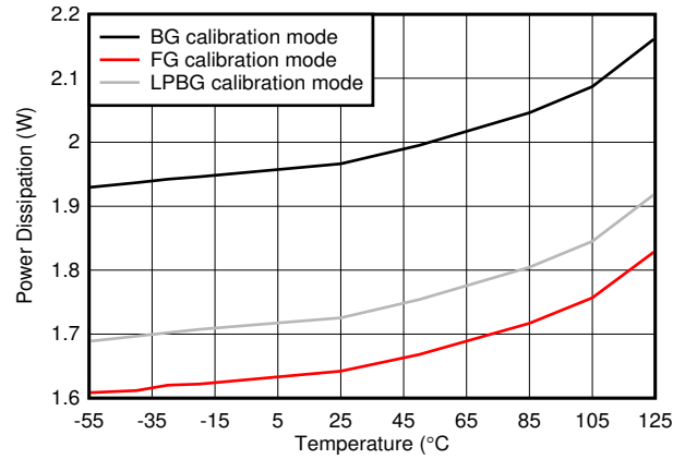
5-124. Dual Channel, Power Dissipation vs Temperature
