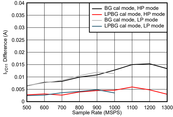
5-121. Dual Channel, I_{VD11} Change with Calibration Mode
