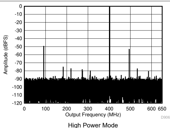
図 5-10. Single Tone FFT at 3497 MHz and -1 dBFS
