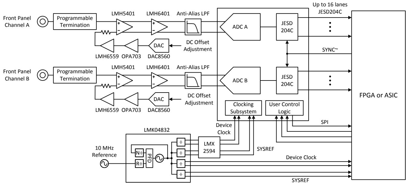
7-3. Typical Configuration for Reconfigurable Oscilloscope
