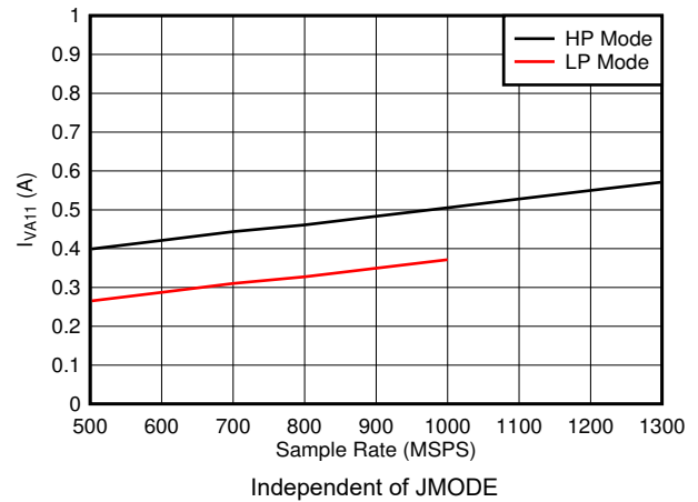
図 5-86. Quad Channel, I_{VA11} vs FS
