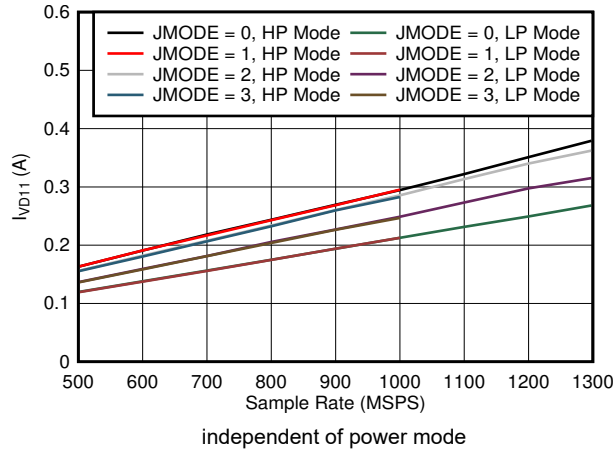
5-97. Dual Channel, I_{VD11} vs FS and JMODE 0 - 3
