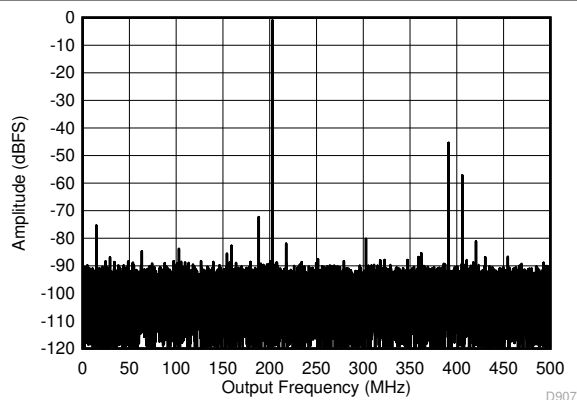
図 5-14. Single Tone FFT at 1797 MHz and -1 dBFS
