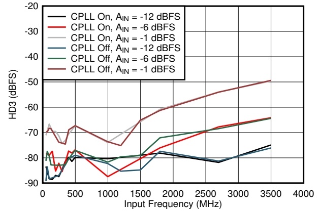
5-74. HD3 vs Input Frequency, CPLL and Input Amplitude
