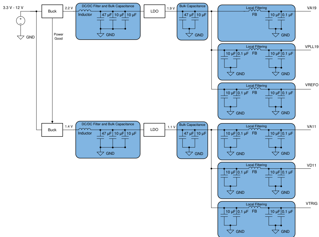
図 7-4. LDO Linear Regulator Approach Example
