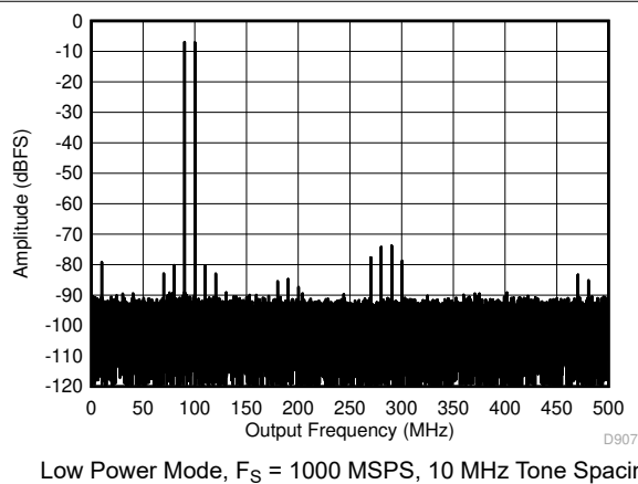
図 5-54. Two Tone FFT at 95.07 MHz Center
