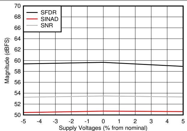
Figure 5-46. SNR, SFDR and SINAD vs Supply Voltage
