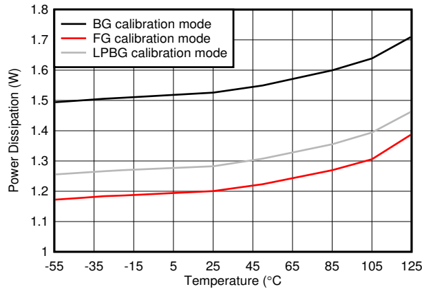
5-125. Single Channel, Power Dissipation vs Temperature
