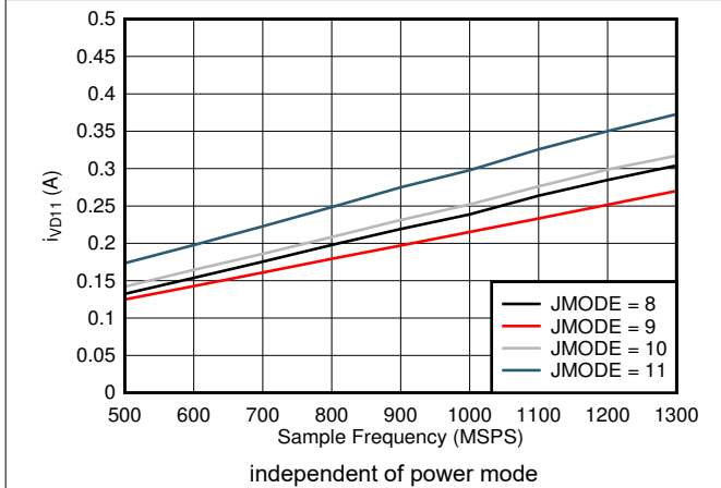
5-99. Dual Channel, I_{VD11} vs FS and JMODE 8 - 11
