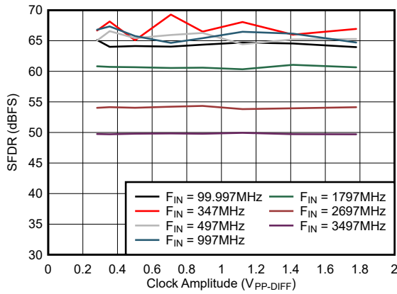
Figure 5-33. SFDR vs Clock Amplitude
