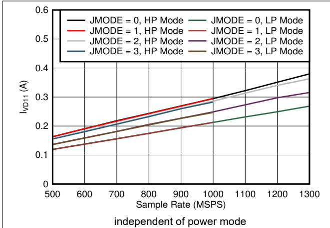
5-97. Dual Channel, I_{VD11} vs FS and JMODE 0 - 3
