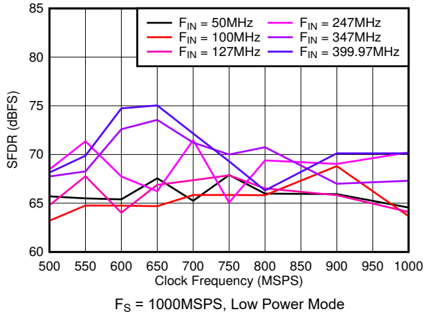
図 5-25. SFDR vs Sample Rate
