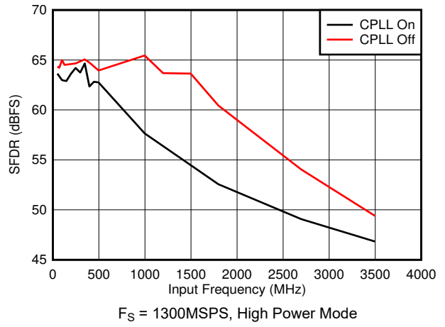
5-62. SFDR vs Input Frequency and CPLL
