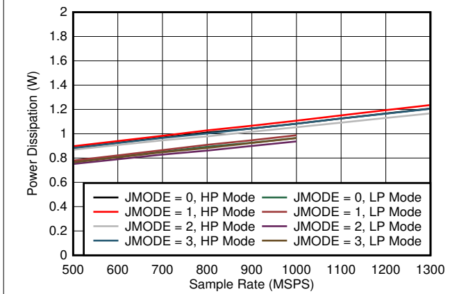
5-101. Single Channel, Power Dissipation vs FS for JMODES 0 - 3
