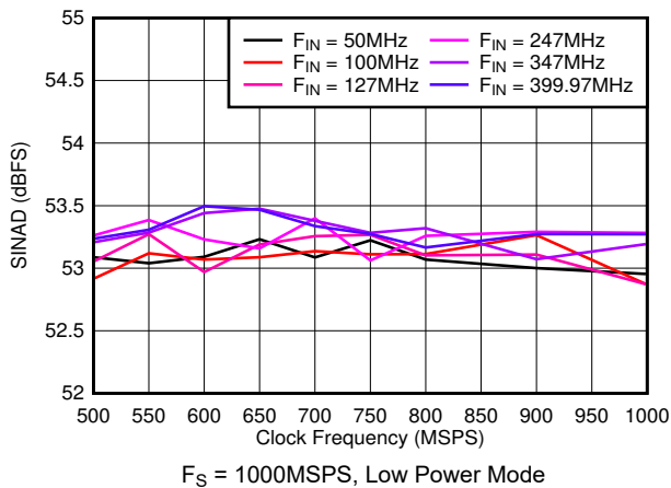
図 5-27. SINAD vs Sample Rate
