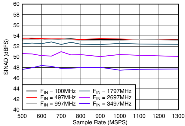
5-23. SINAD vs Sample Rate
