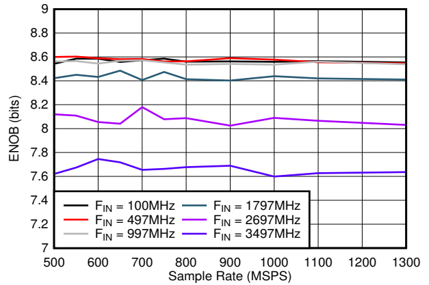
5-24. ENOB vs Sample Rate
