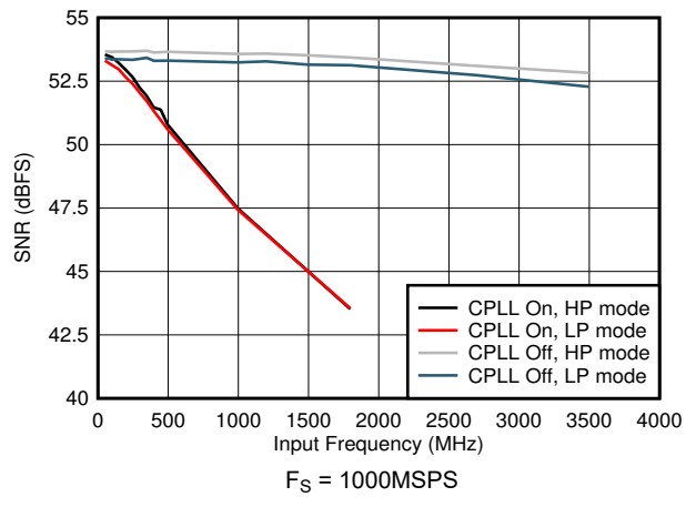
5-66. SNR vs Input Frequency and CPLL
