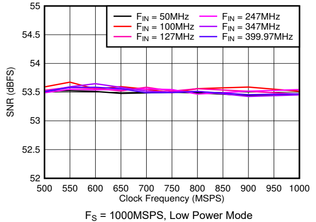
図 5-26. SNR vs Sample Rate
