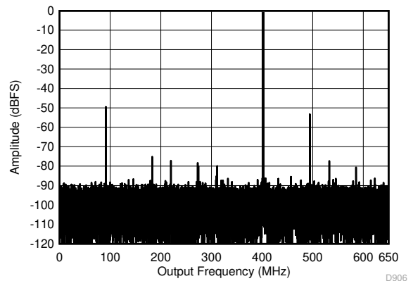
5-8. Single Tone FFT at 1797 MHz and -1 dBFS
