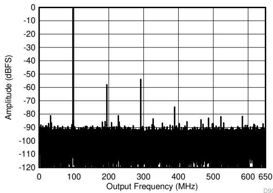
5-7. Single Tone FFT at 1497 MHz and -1 dBFS
