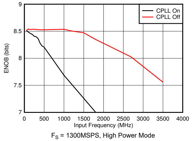
5-64. ENOB vs Input Frequency and CPLL
