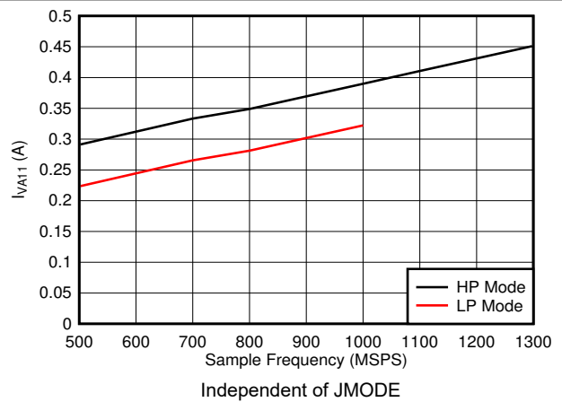
5-96. Dual Channel, I_{VA11} vs FS
