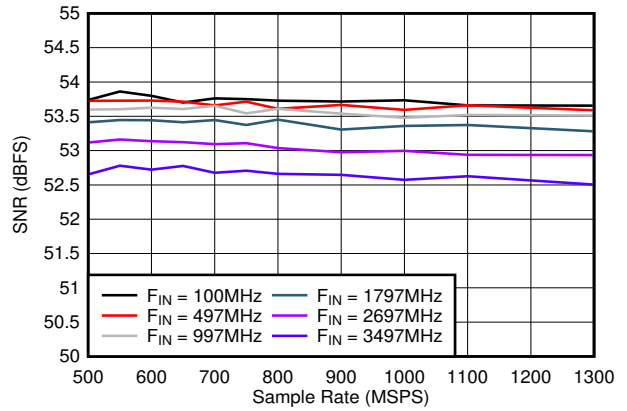
5-22. SNR vs Sample Rate
