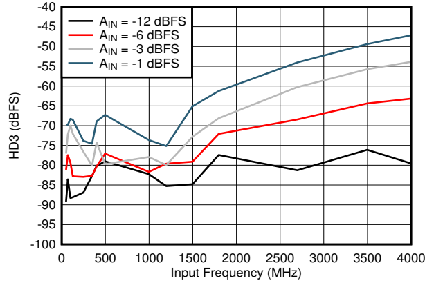
5-20. HD3 vs Input Frequency
