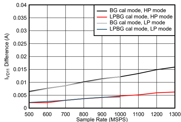
5-122. Dual Channel, I_{VD11} Change with Calibration Mode
