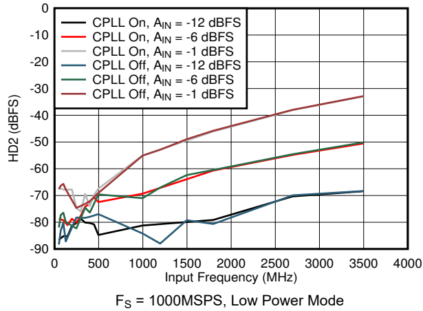
5-79. HD2 vs Input Frequency, CPLL and Input Amplitude
