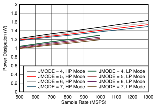
図 5-92. Dual Channel, Power Dissipation vs FS for JMODES 4 - 7
