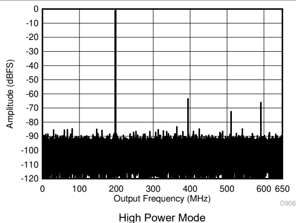
図 5-7. Single Tone FFT at 1497 MHz and -1 dBFS
