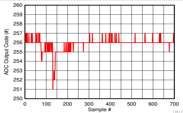
5-126. Background Calibration Core Transition (midscale voltage)
