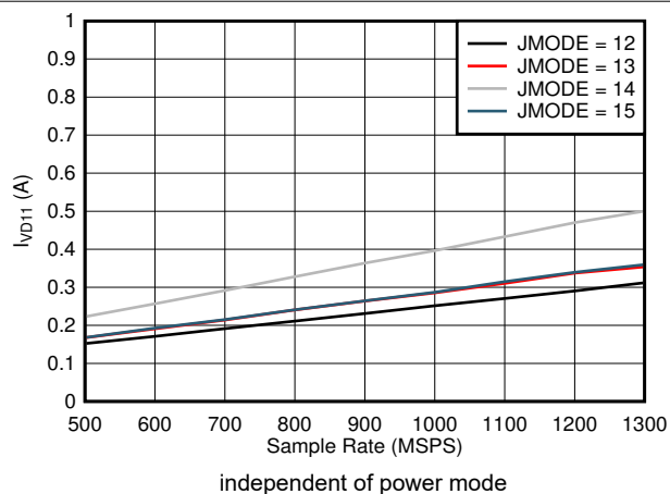
図 5-90. Quad Channel, I_{VD11} vs FS and JMODE 12 - 15
