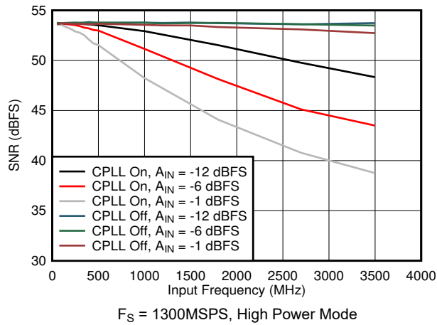
図 5-69. SNR vs Input Frequency, CPLL and Input Amplitude
