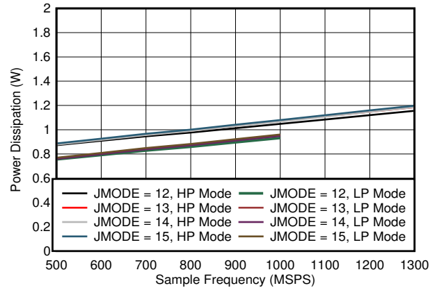
5-104. Single Channel, Power Dissipation vs FS for JMODES 12 - 15
