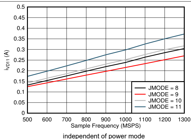
Figure 5-99. Dual Channel, I_{VD11} vs FS and JMODE 8 - 11
