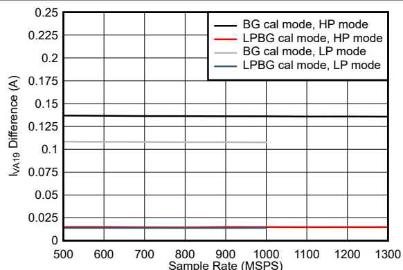
5-116. Single Channel, I_{VA19} Change with Calibration Mode
