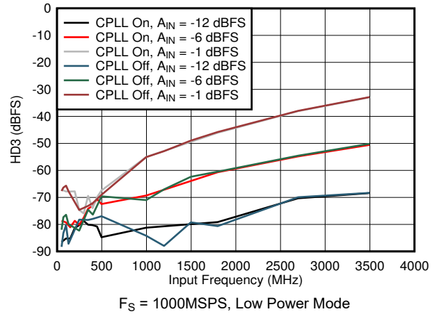
5-80. HD3 vs Input Frequency, CPLL and Input Amplitude
