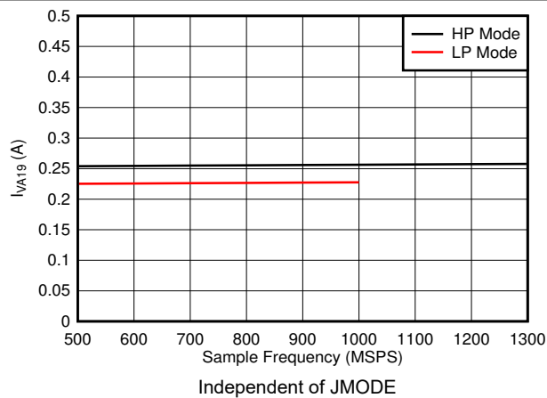
5-105. Single Channel, I_{VA19} vs FS
