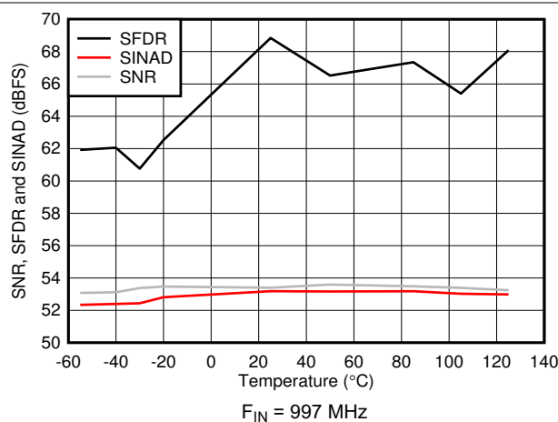
図 5-35. SNR, SFDR and SINAD vs Temperature
