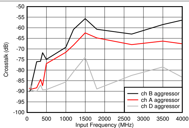
図 5-60. Crosstalk to Channel B vs F_{IN}
