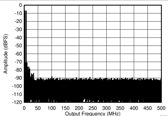
図 5-56. Two Tone FFT at 998 MHz Center
