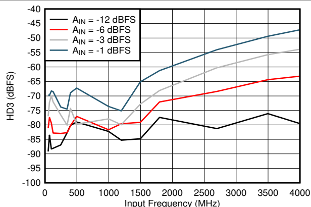
図 5-20. HD3 vs Input Frequency
