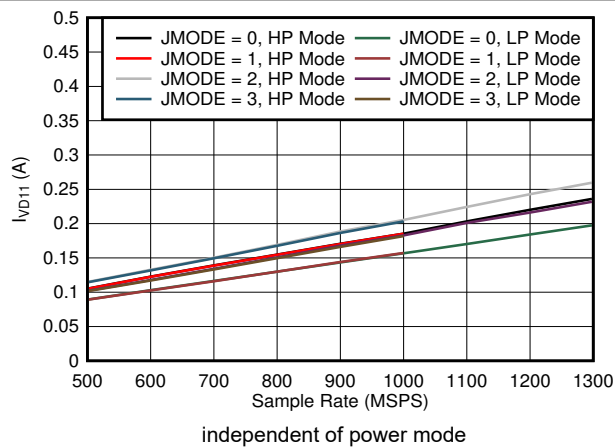
5-107. Single Channel, I_{VD11} vs FS and JMODE 0 - 3
