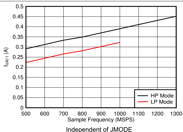
図 5-96. Dual Channel, I_{VA11} vs FS
