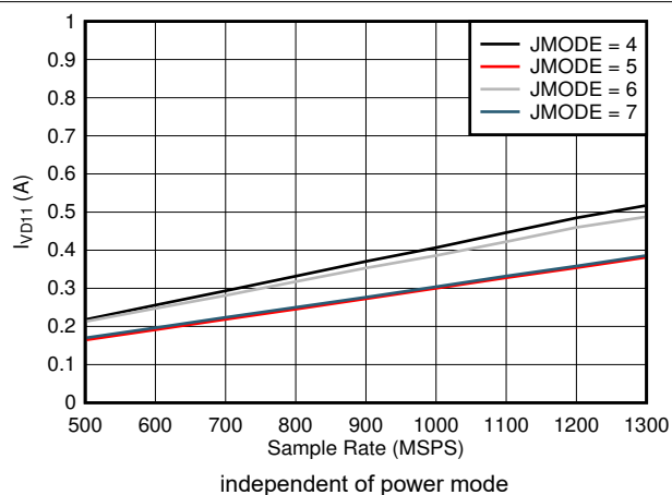
図 5-88. Quad Channel, I_{VD11} vs FS and JMODE 4 - 7
