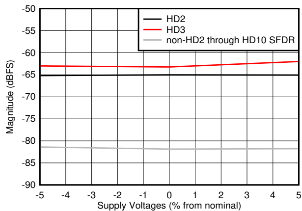
5-45. HD2, HD3 and Worst non-HD Spur vs Supply Voltage
