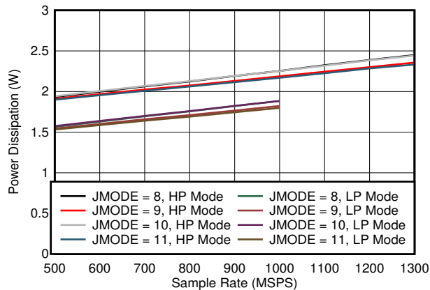
5-83. Quad Channel, Power Dissipation vs FS for JMODES 8 - 11
