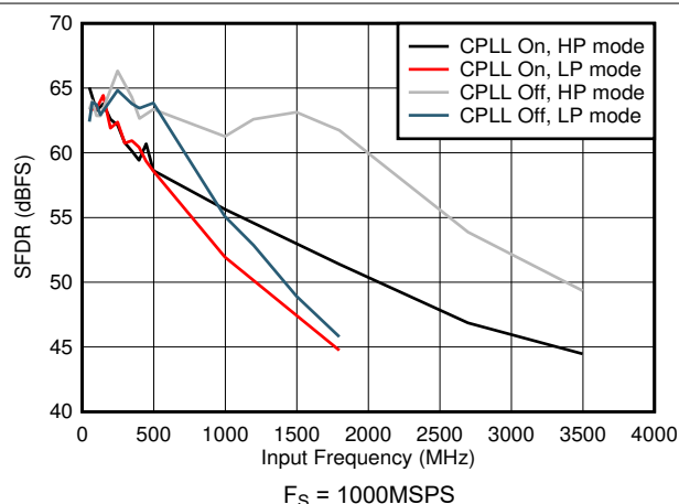
5-65. SFDR vs Input Frequency and CPLL
