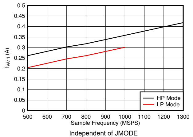
5-106. Single Channel, I_{VA11} vs FS
