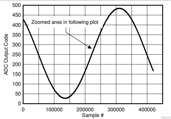
図 5-127. Background Calibration Core Transition (AC Signal)
