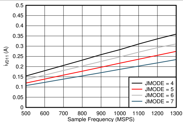
Figure 5-98. Dual Channel, I_{VD11} vs FS and JMODE 4 - 7
