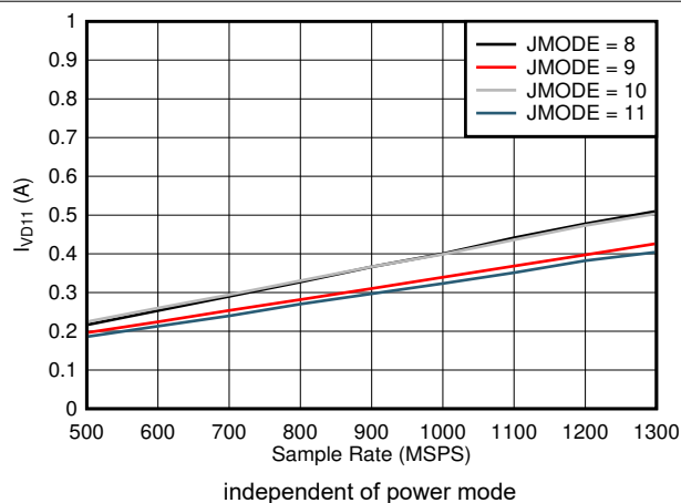
図 5-89. Quad Channel, I_{VD11} vs FS and JMODE 8 - 11
