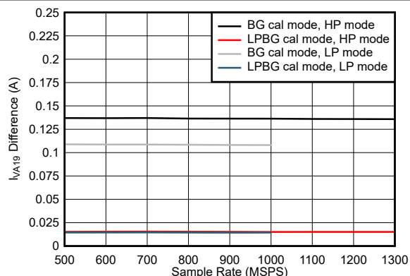
5-115. Dual Channel, I_{VA19} Change with Calibration Mode
