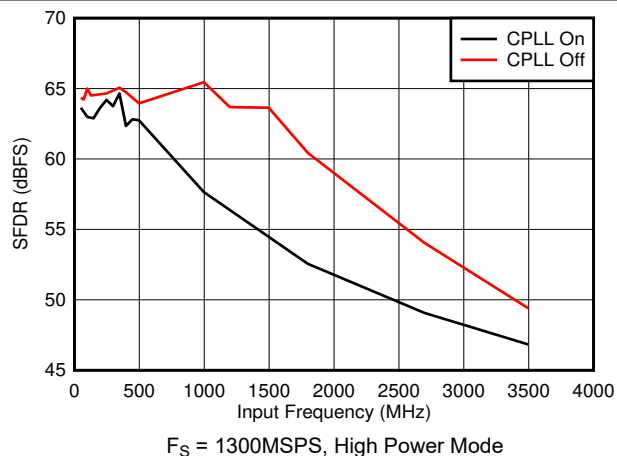
5-62. SFDR vs Input Frequency and CPLL
