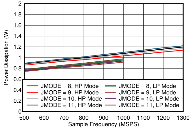
5-103. Single Channel, Power Dissipation vs FS for JMODES 8 - 11
