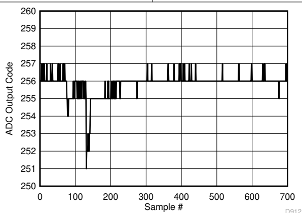
図 5-129. Background Calibration Core Transition (DC Signal)
