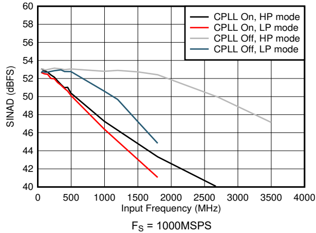
図 5-67. SINAD vs Input Frequency and CPLL
