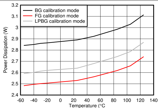
5-123. Quad Channel, Power Dissipation vs Temperature
