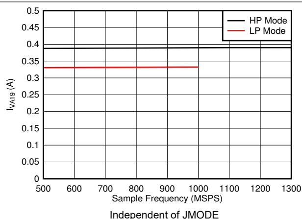
図 5-95. Dual Channel, I_{VA19} vs FS
