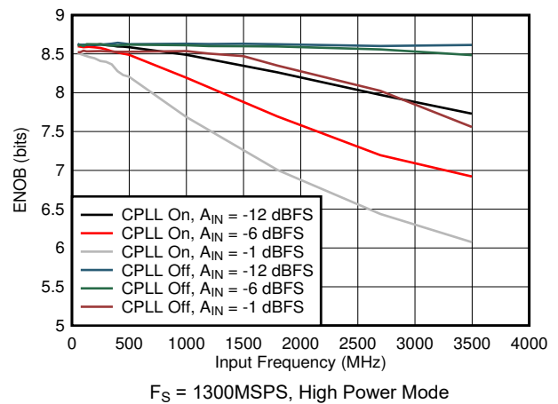
図 5-72. ENOB vs Input Frequency, CPLL and Input Amplitude
