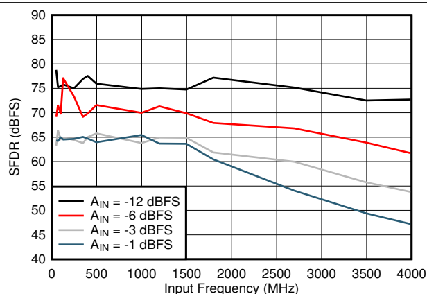
図 5-15. SFDR vs Input Frequency
