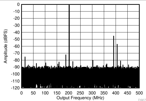
図 5-14. Single Tone FFT at 1797 MHz and -1 dBFS
