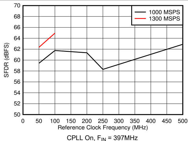
5-61. SFDR vs Reference Clock Frequency
