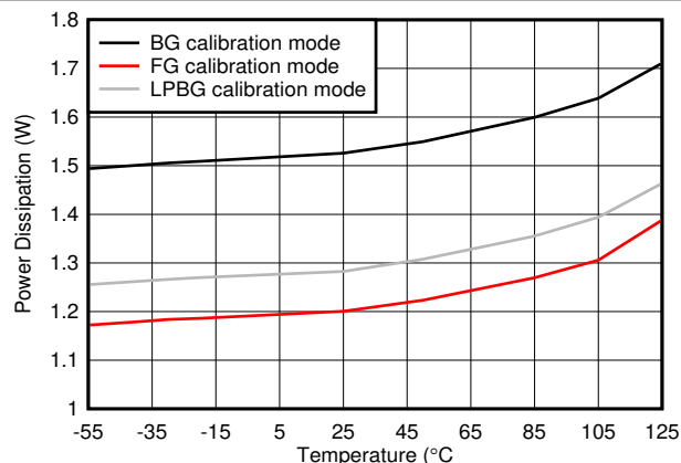
5-125. Single Channel, Power Dissipation vs Temperature
