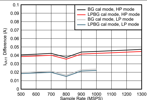
5-117. Quad Channel, I_{VA11} Change with Calibration Mode
