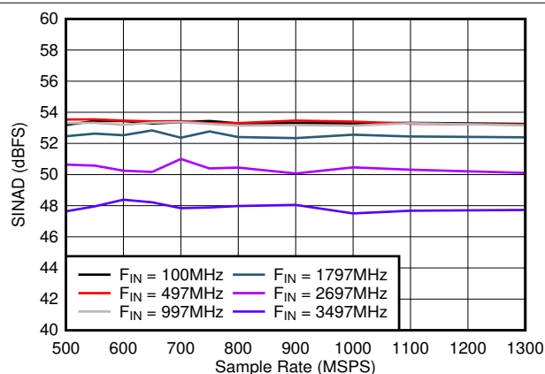
図 5-23. SINAD vs Sample Rate
