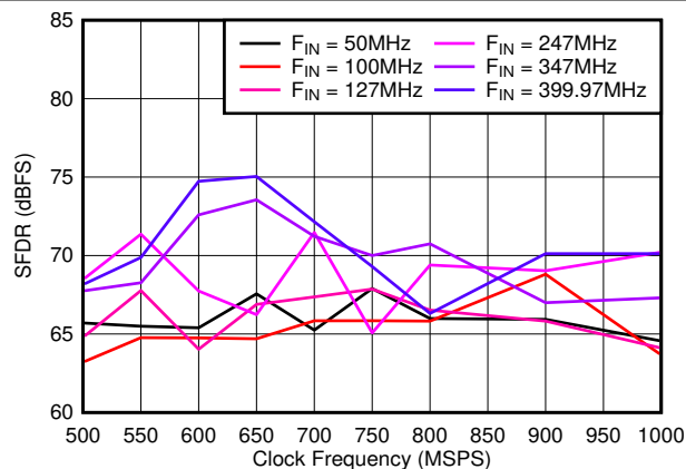
図 5-25. SFDR vs Sample Rate
