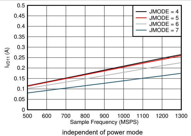
5-108. Single Channel, I_{VD11} vs FS and JMODE 4 - 7
