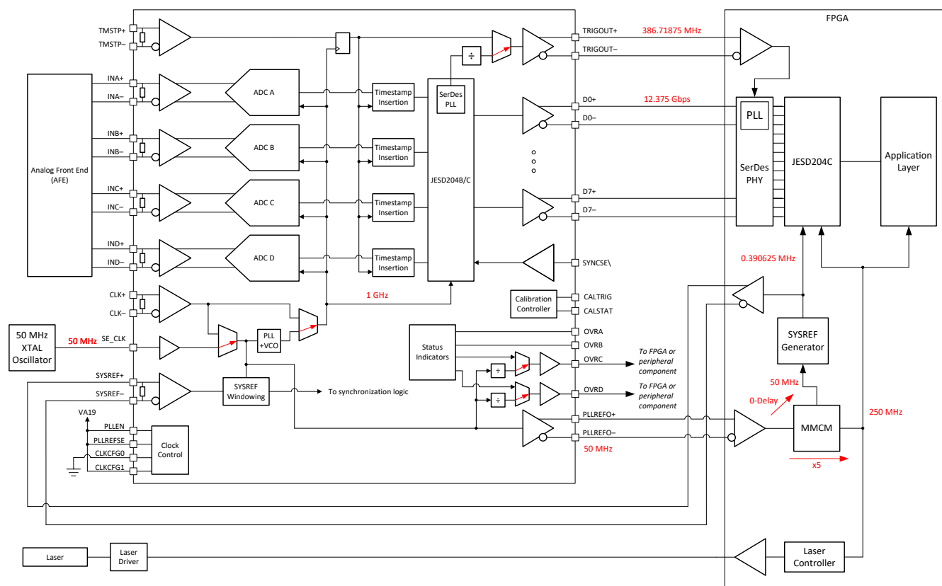
7-1. Typical Configuration for a LiDAR Digitizer
