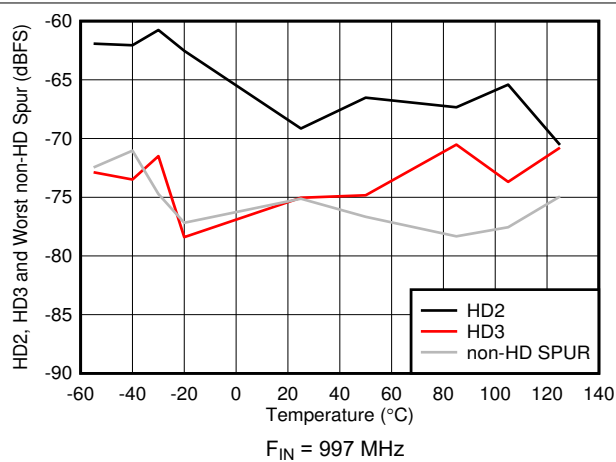
図 5-36. HD2, HD3 and worst non-HD Spur vs Temperature
