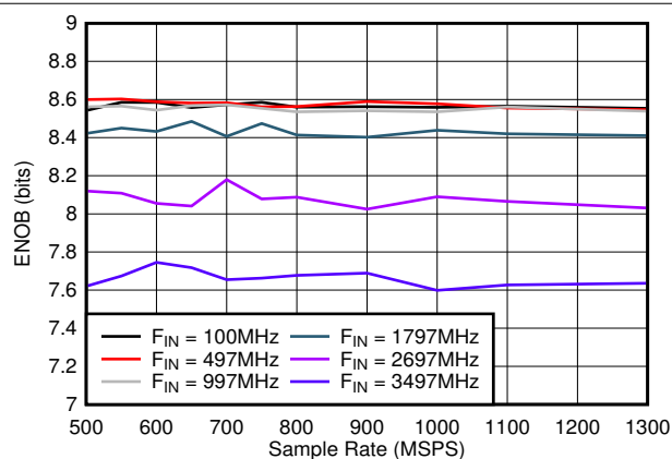
図 5-24. ENOB vs Sample Rate
