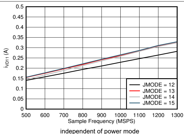
Figure 5-100. Dual Channel, I_{VD11} vs FS and JMODE 12 - 15
