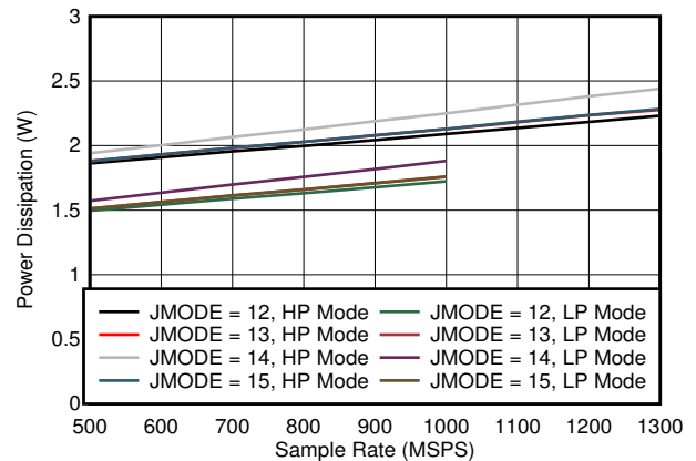
5-84. Quad Channel, Power Dissipation vs FS for JMODES 12 - 15
