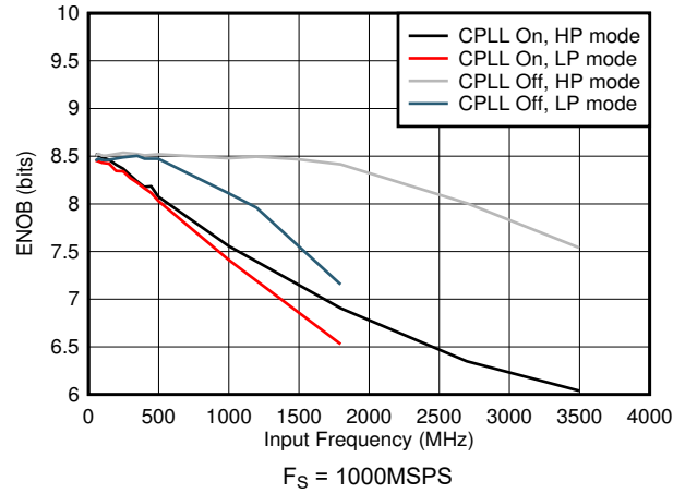
図 5-68. ENOB vs Input Frequency and CPLL
