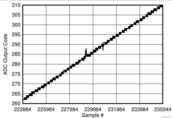
図 5-128. Background Calibration Core Transition (AC Signal Zoomed)
