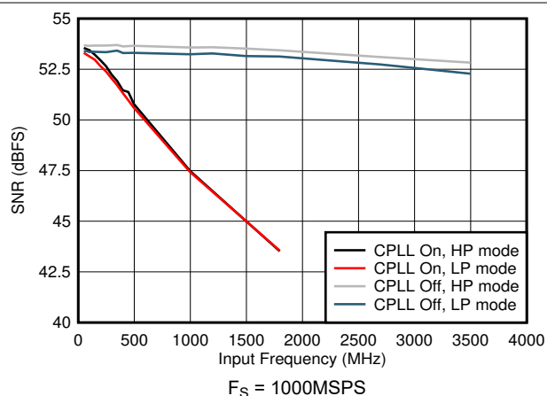
5-66. SNR vs Input Frequency and CPLL
