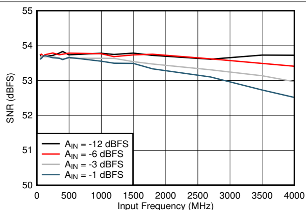
図 5-16. SNR vs Input Frequency
