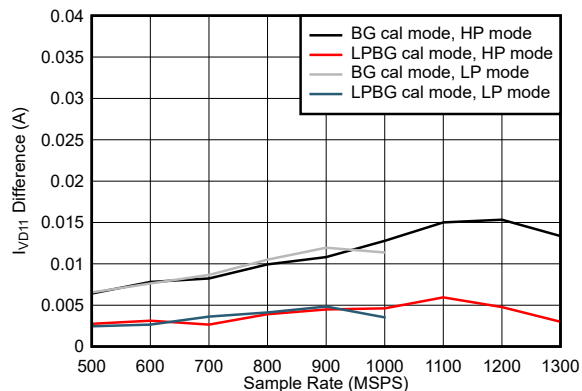
5-121. Dual Channel, I_{VD11} Change with Calibration Mode
