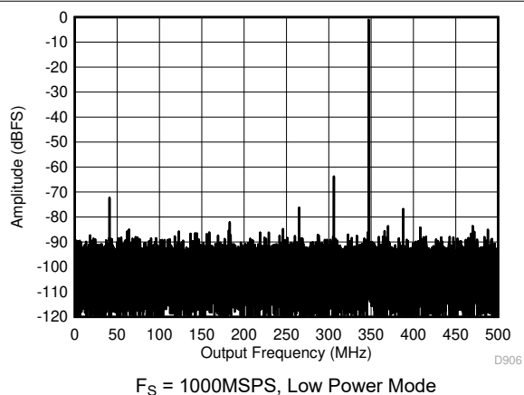
図 5-12. Single Tone FFT at 347 MHz and -1 dBFS
