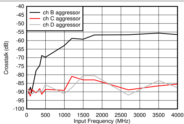
図 5-59. Crosstalk to Channel A vs F_{IN}
