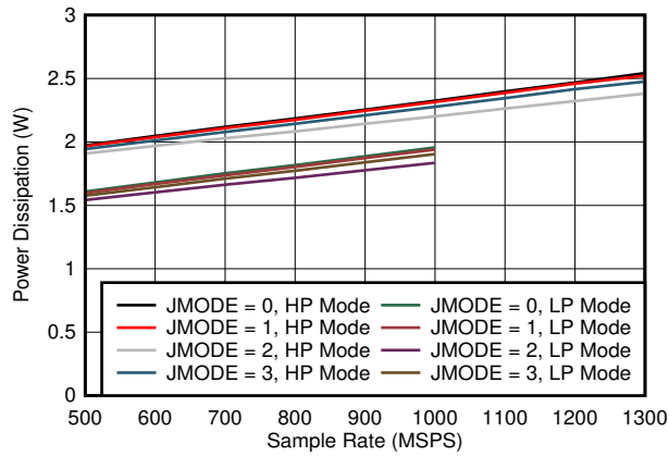
5-81. Quad Channel, Power Dissipation vs FS for JMODES 0 - 3
