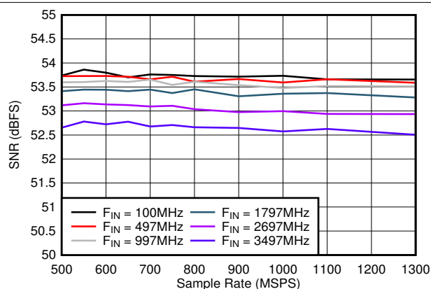
図 5-22. SNR vs Sample Rate
