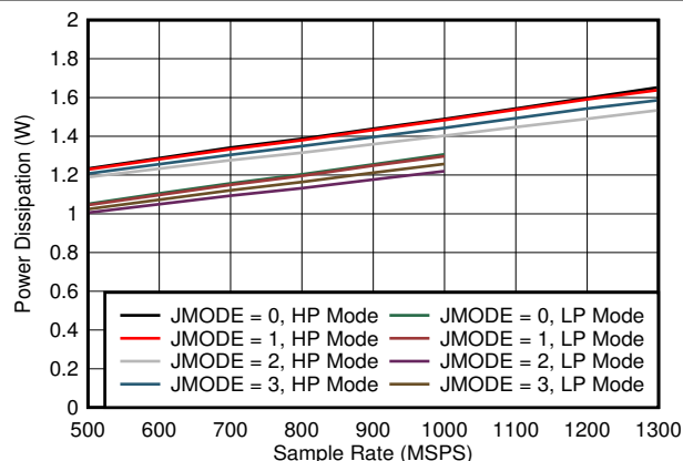
図 5-91. Dual Channel, Power Dissipation vs FS for JMODES 0 - 3
