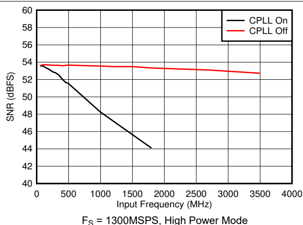
5-63. SNR vs Input Frequency and CPLL
