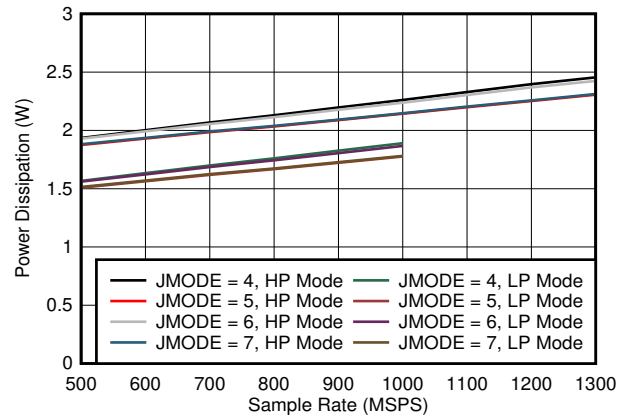
5-82. Quad Channel, Power Dissipation vs FS for JMODES 4 - 7
