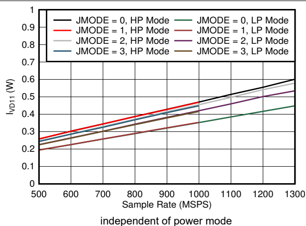
図 5-87. Quad Channel, I_{VD11} vs FS and JMODE 0 - 3
