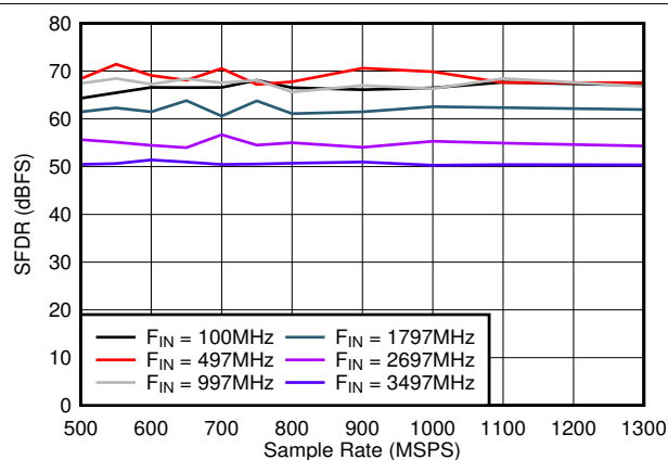
図 5-21. SFDR vs Sample Rate
