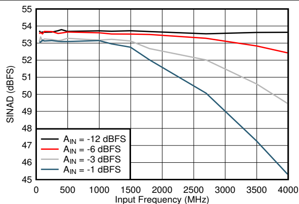
図 5-17. SINAD vs Input Frequency
