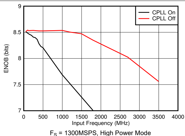
5-64. ENOB vs Input Frequency and CPLL
