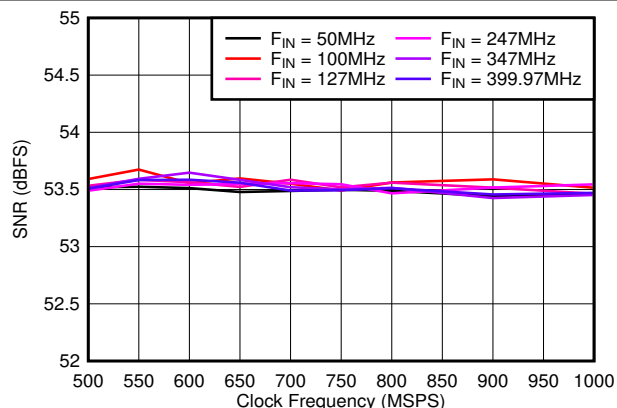
図 5-26. SNR vs Sample Rate
