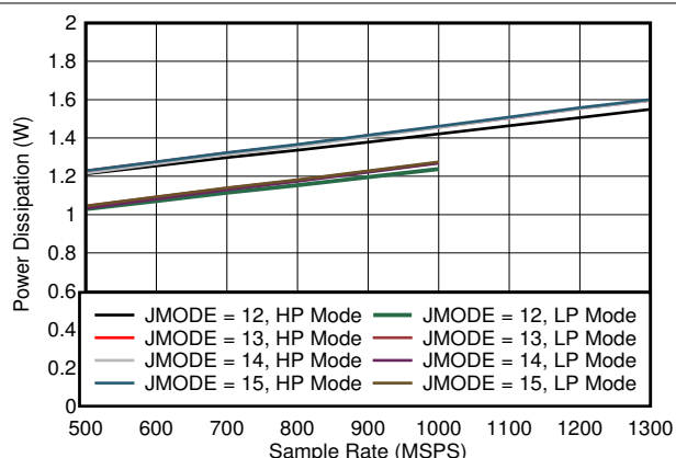
図 5-94. Dual Channel, Power Dissipation vs FS for JMODES 12 - 15
