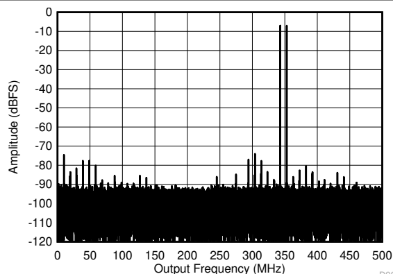
図 5-55. Two Tone FFT at 348 MHz Center
