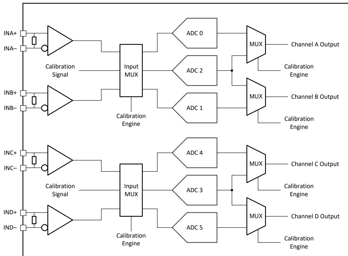
図 6-15. Quad Channel Calibration System Block Diagram
