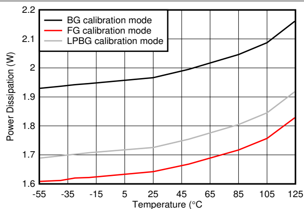
5-124. Dual Channel, Power Dissipation vs Temperature
