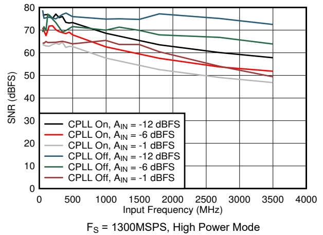
図 5-70. SFDR vs Input Frequency, CPLL and Input Amplitude
