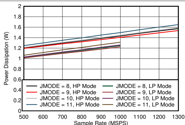
図 5-93. Dual Channel, Power Dissipation vs FS for JMODES 8 - 11
