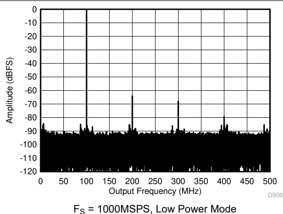
図 5-11. Single Tone FFT at 99.997 MHz and -1 dBFS
