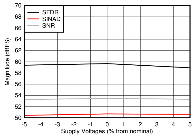
5-46. SNR, SFDR and SINAD vs Supply Voltage
