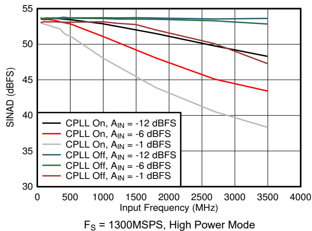
図 5-71. SINAD vs Input Frequency, CPLL and Input Amplitude
