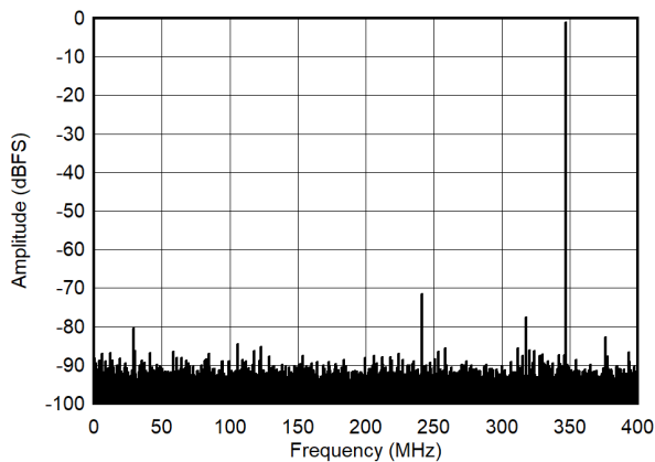
図 5-11. Single Tone FFT at 347MHz and -1dBFS
