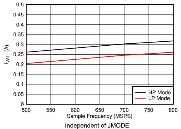
図 5-96. Single Channel, I_{VA11} vs F_S
