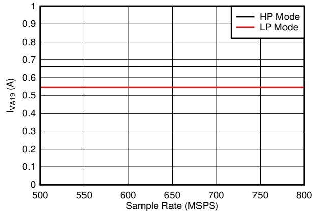
Figure 5-75. Quad Channel, I_{VA19} vs F_S
