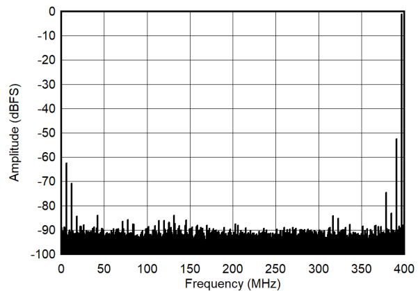
図 5-12. Single Tone FFT at 1197MHz and -1dBFS
