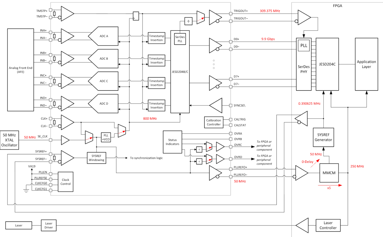
図 7-1. Typical Configuration for a LiDAR Digitizer
