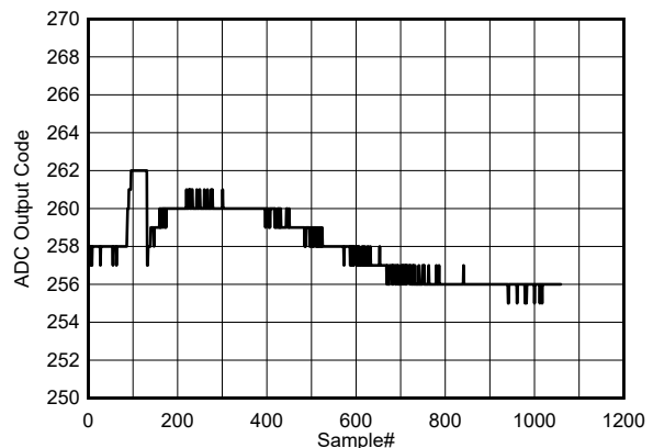
5-116. Background Core Transition (DC midscale input)
