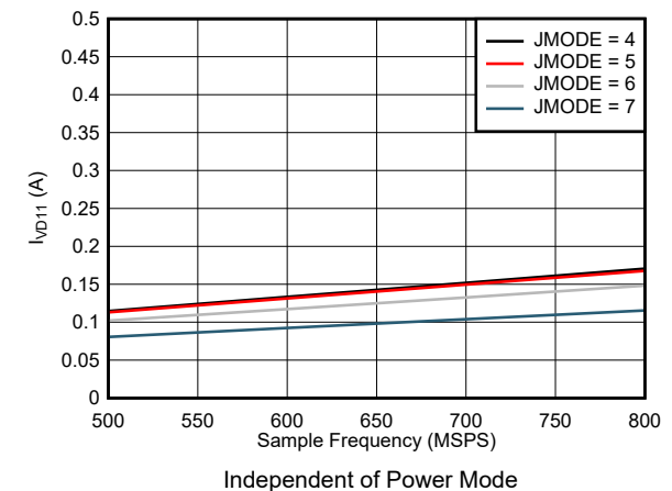
図 5-98. Single Channel, I_{VD11} vs F_S for JMODES 4 - 7
