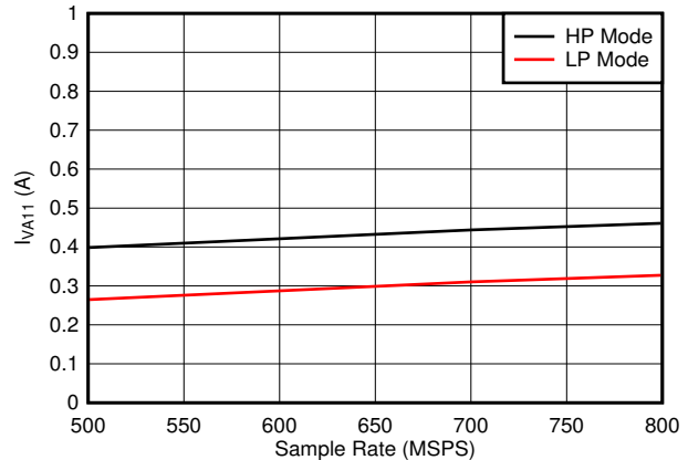
Figure 5-76. Quad Channel, I_{VA11} vs F_S
