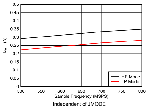
図 5-86. Dual Channel, I_{VA11} vs F_S
