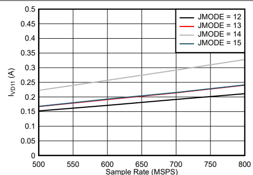
Figure 5-80. Quad Channel, I_{VD11} vs F_S for JMODES 12 - 15
