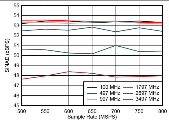
Figure 5-22. SINAD vs Sample Rate
