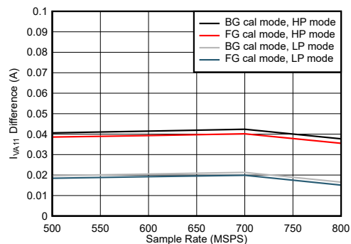
Figure 5-107. Quad Channel, I_{VA11} Change with Calibration Mode
