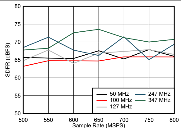
Figure 5-24. SFDR vs Sample Rate
